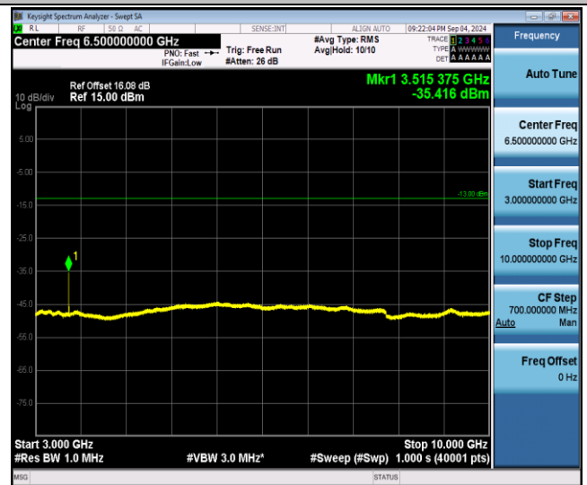
Band12-10MHz-QPSK-23095-1RB#0-3000~10000-PASS
