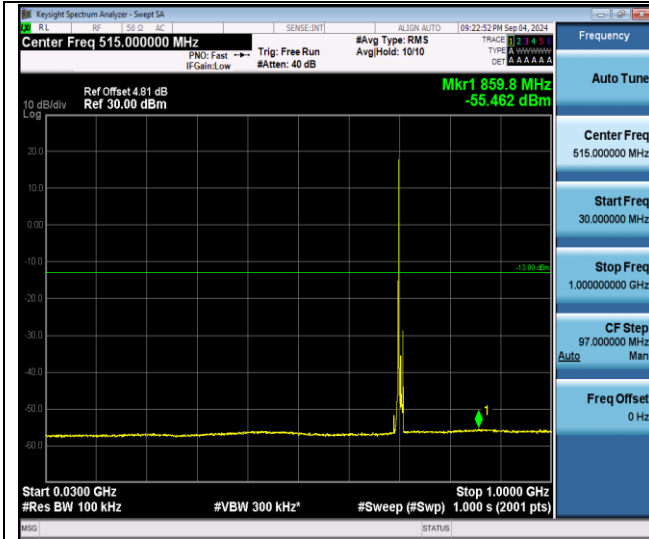
Band12-10MHz-QPSK-23130-1RB#0-30~1000-PASS
