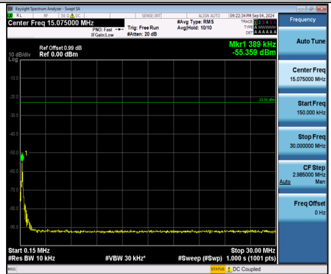
Band12-10MHz-QPSK-23130-1RB#0-0.15~30-PASS
