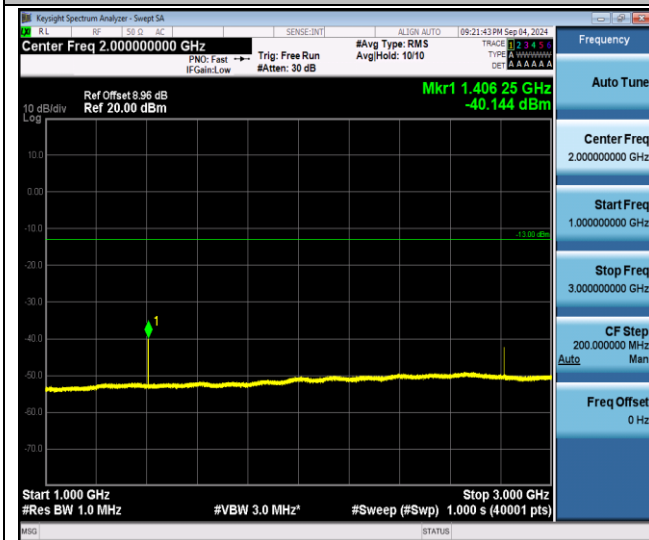
Band12-10MHz-QPSK-23095-1RB#0-1000~3000-PASS
