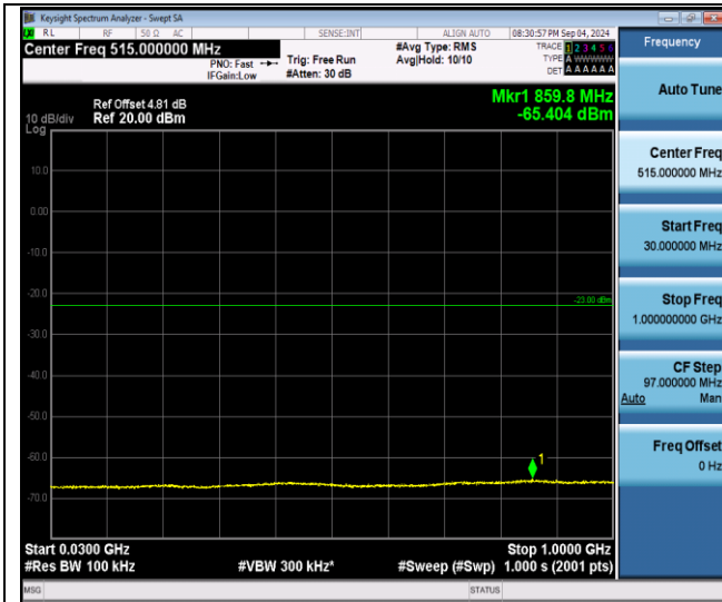
Band4-20MHz-QPSK-20300-1RB#0-30~1000-PASS
