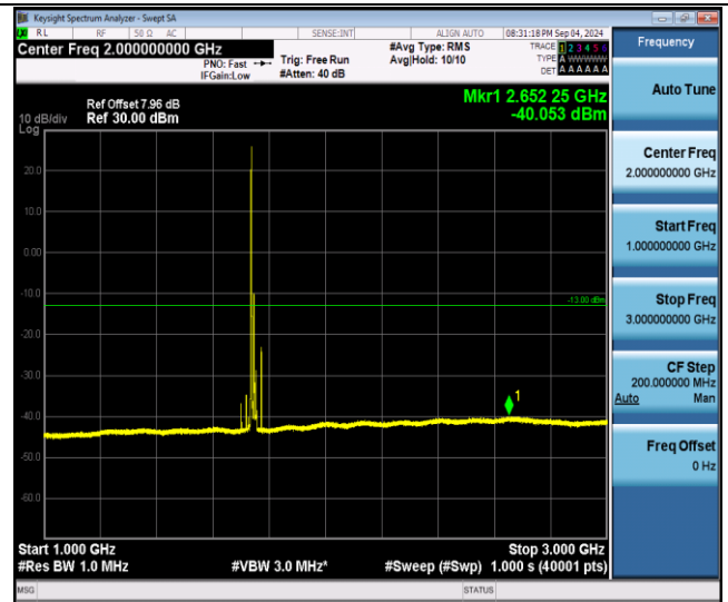
Band4-20MHz-QPSK-20300-1RB#0-1000~3000-PASS
