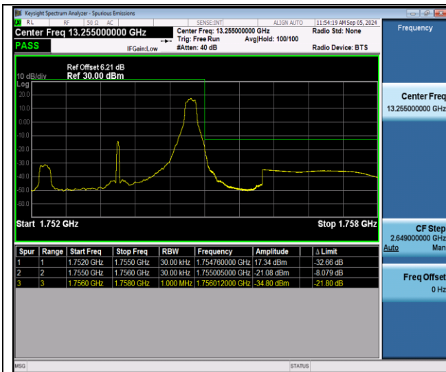
Band4-3MHz-QPSK-20385-1RB#14-PASS
