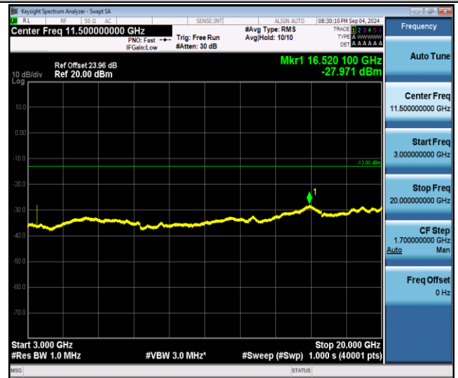
Band4-20MHz-QPSK-20175-1RB#0-3000~20000-PASS
