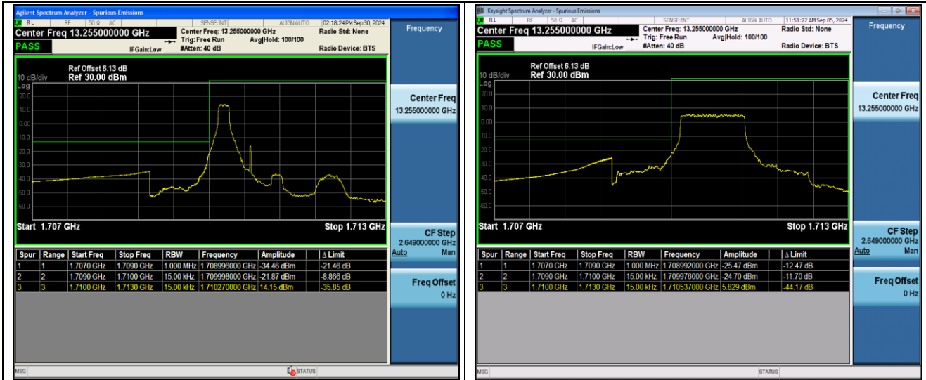
Band4-1.4MHz-QPSK-19957-1RB#0-PASS
