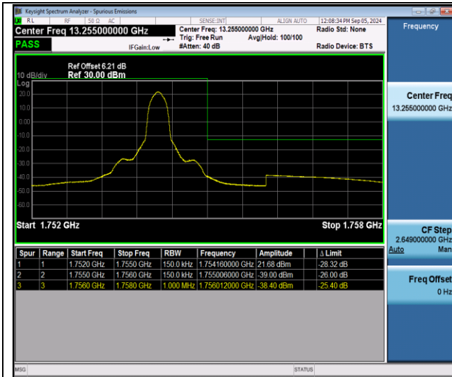
Band4-15MHz-QPSK-20325-1RB#74-PASS
