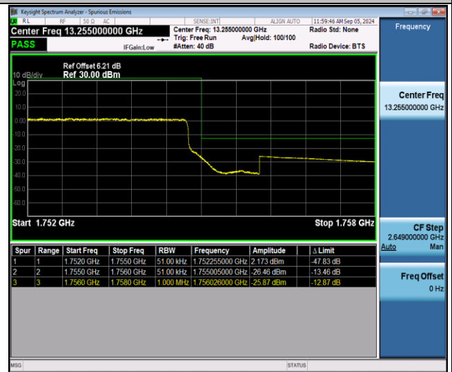
Band4-5MHz-QPSK-20375-25RB#0-PASS
