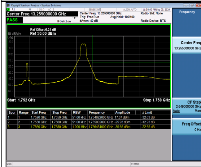
Band4-5MHz-QPSK-20375-1RB#24-PASS
