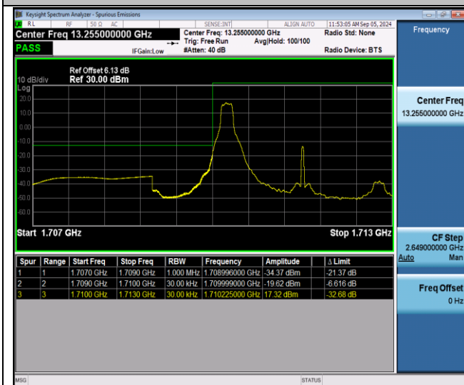
Band4-3MHz-QPSK-19965-1RB#0-PASS
