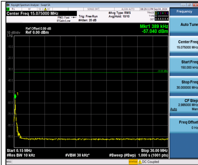
Band4-20MHz-QPSK-20175-1RB#0-0.15~30-PASS
