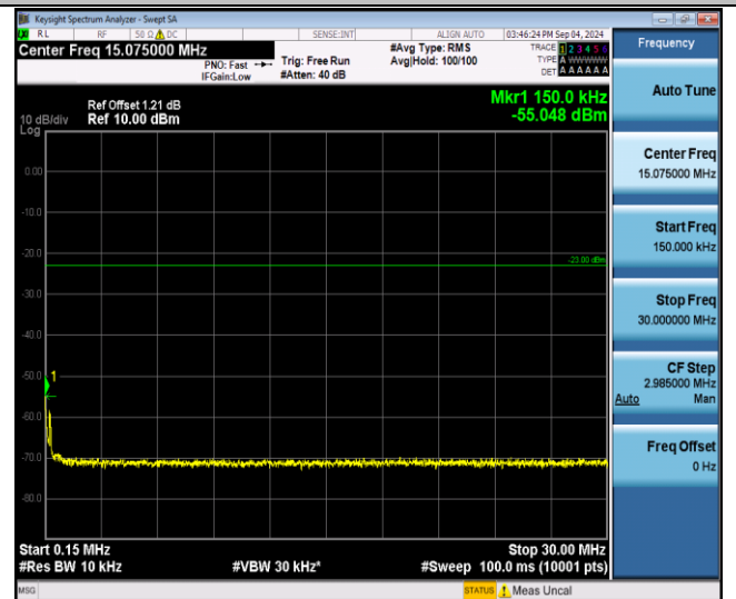
EGPRS850-251-8-0.15~30MHz-PASS
