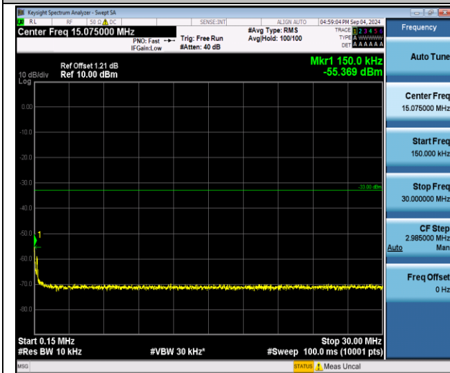
EGPRS1900-512-2-0.15~30MHz-PASS
