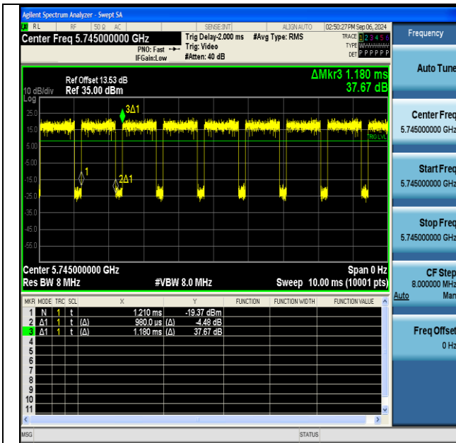
NTNV-11ac20SISO-Ant1-5745
