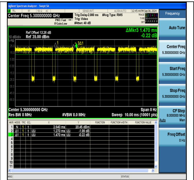
NTNV-11n20SISO-Ant1-5300
