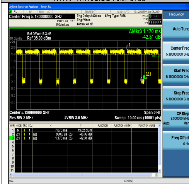
NTNV-11ac20SISO-Ant1-5180
