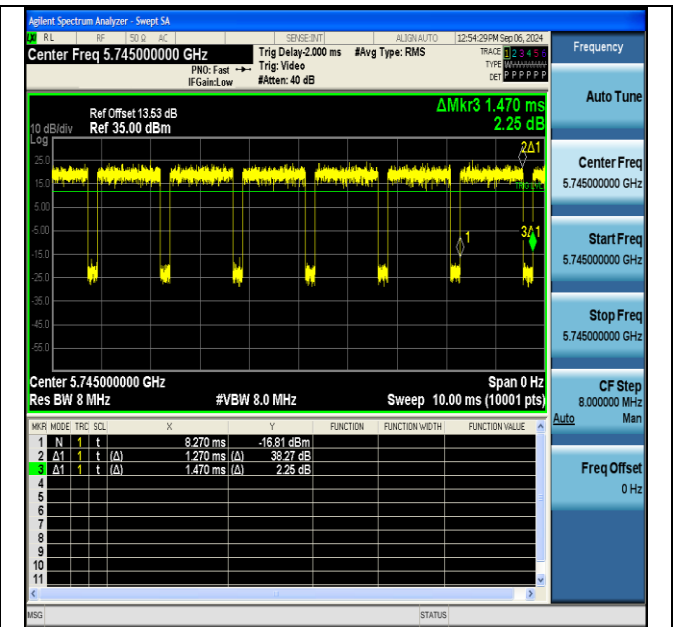
NTNV-11n20SISO-Ant1-5745
