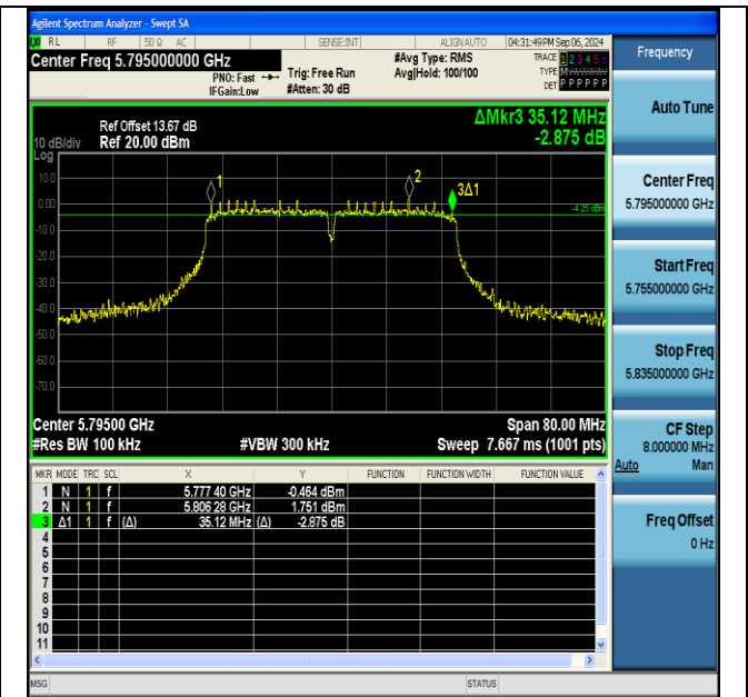
11ac40SISO-Ant1-5795-PASS
