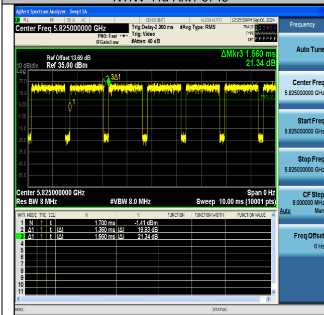
NTNV-11a-Ant1-5825
