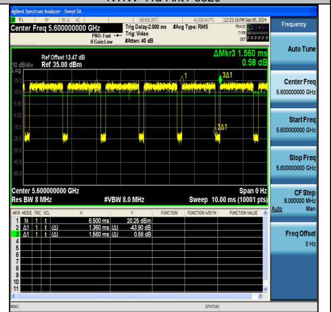
NTNV-11a-Ant1-5600
