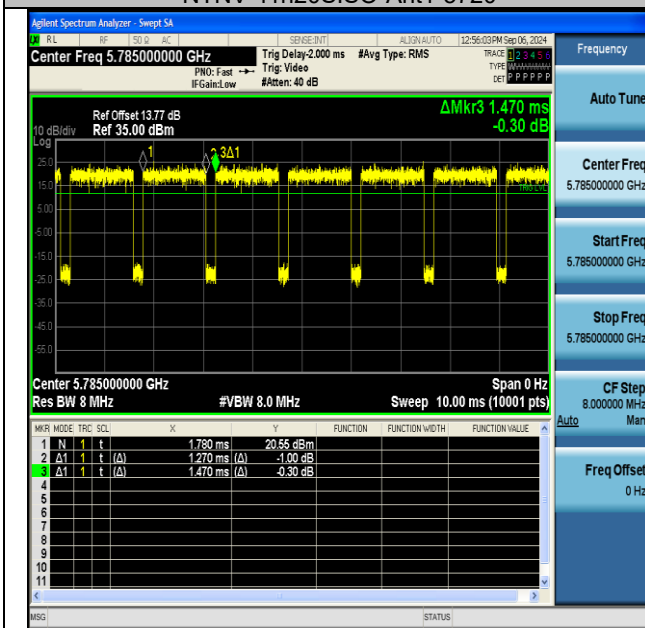
NTNV-11n20SISO-Ant1-5785
