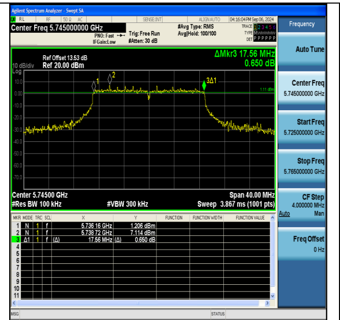
11n20SISO-Ant1-5745-PASS
