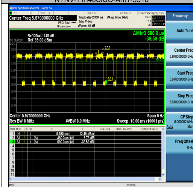
NTNV-11n40SISO-Ant1-5670
