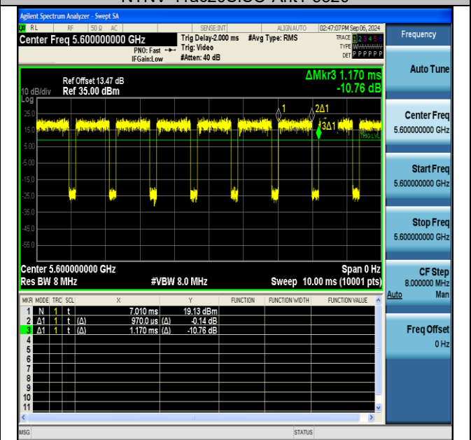
NTNV-11ac20SISO-Ant1-5600
