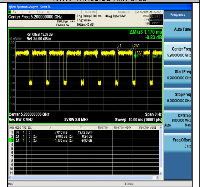
NTNV-11ac20SISO-Ant1-5200
