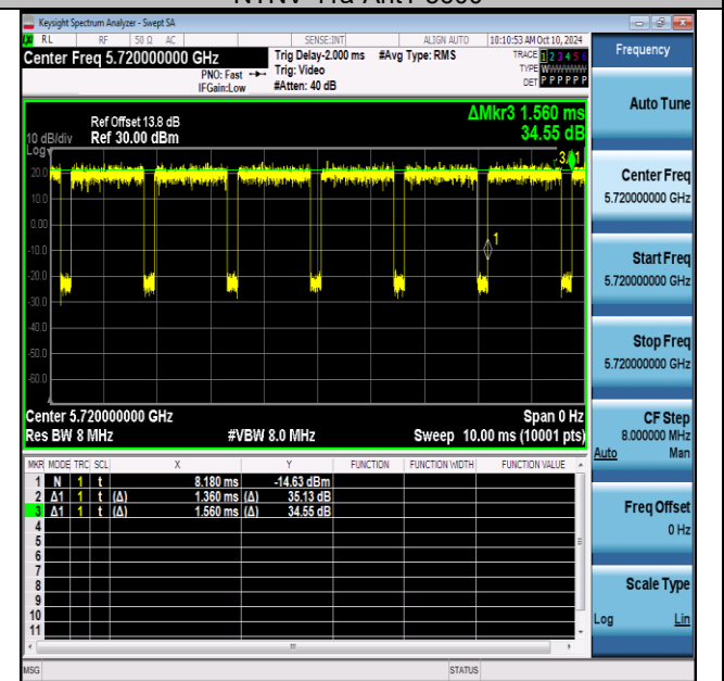
NTNV-11a-Ant1-5720
