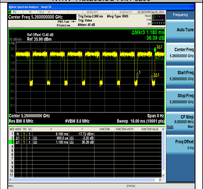
NTNV-11ac20SISO-Ant1-5260
