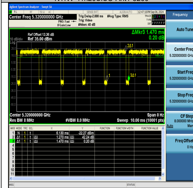
NTNV-11n20SISO-Ant1-5320
