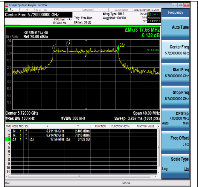
11ac20SISO-Ant1-5720
