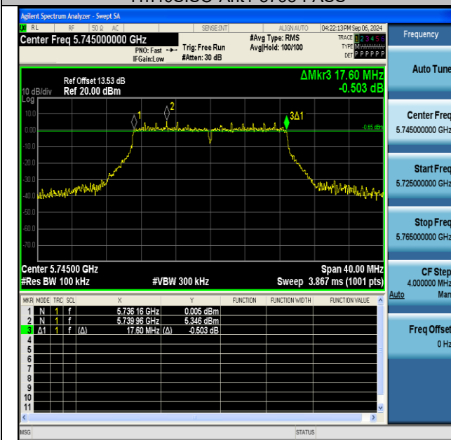
11ac20SISO-Ant1-5745-PASS
