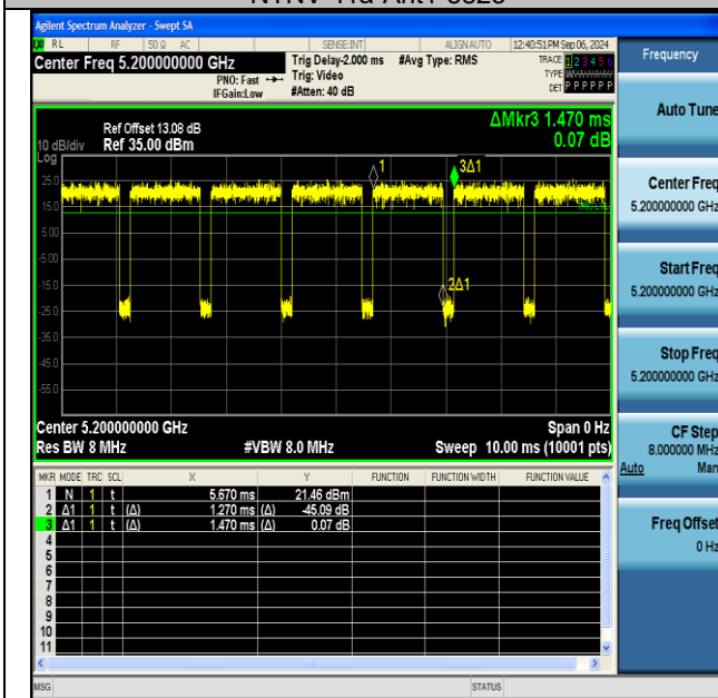
NTNV-11n20SISO-Ant1-5200
