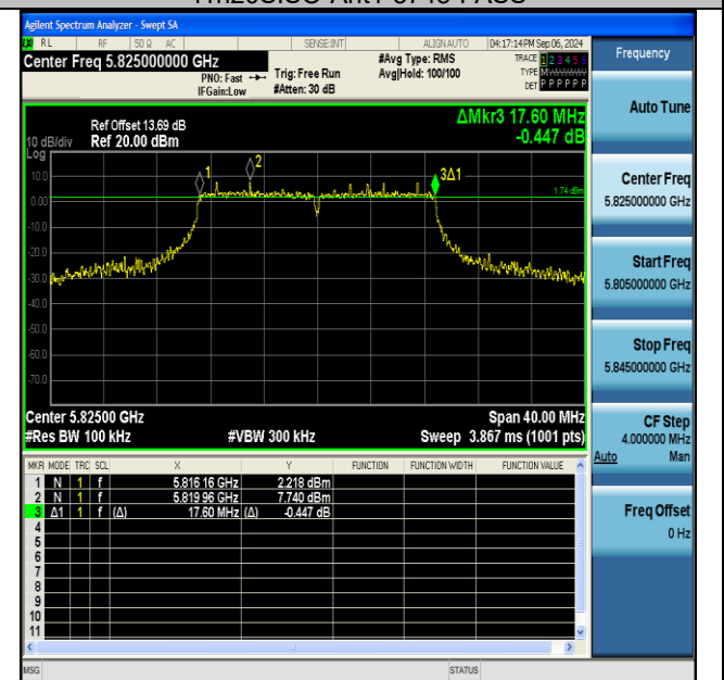
11n20SISO-Ant1-5825-PASS
