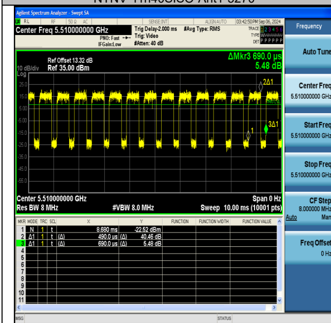
NTNV-11n40SISO-Ant1-5510
