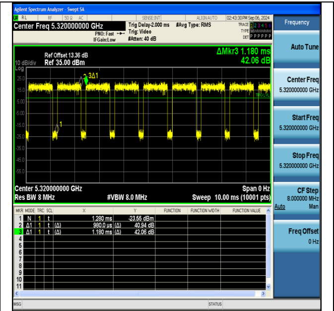
NTNV-11ac20SISO-Ant1-5320
