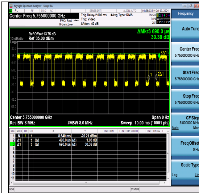
NTNV-11n40SISO-Ant1-5755
