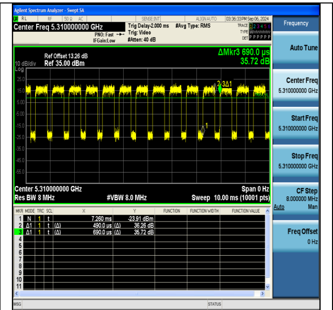
NTNV-11n40SISO-Ant1-5310
