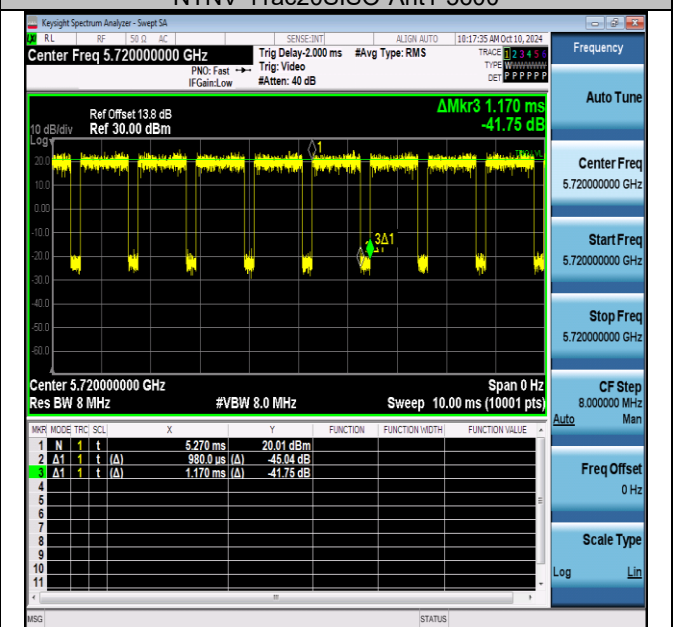
NTNV-11ac20SISO-Ant1-5720
