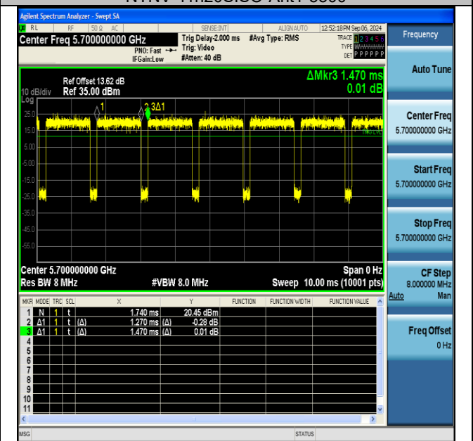
NTNV-11n20SISO-Ant1-5700
