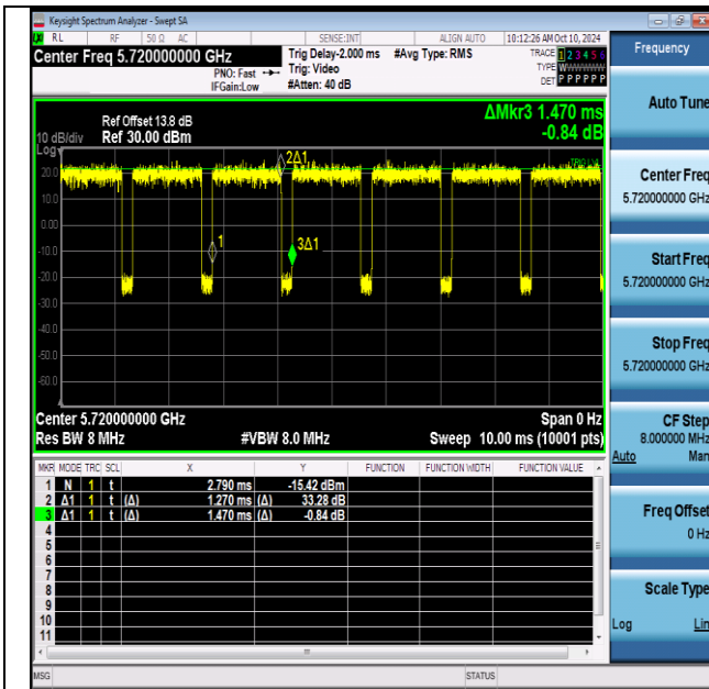
NTNV-11n20SISO-Ant1-5720
