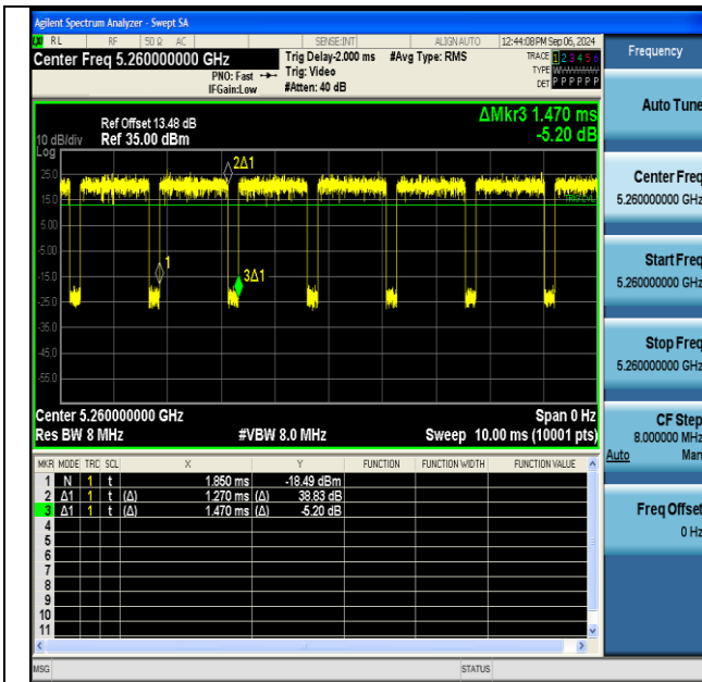
NTNV-11n20SISO-Ant1-5260
