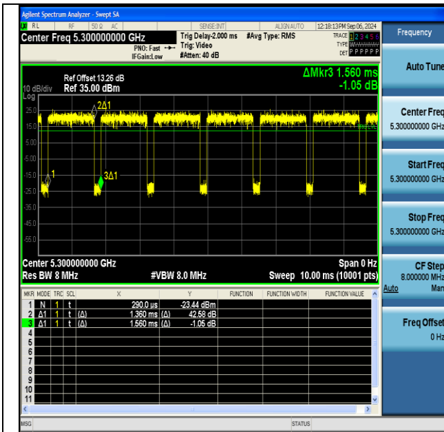
NTNV-11a-Ant1-5300
