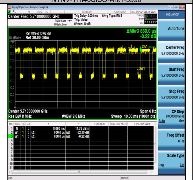
NTNV-11n40SISO-Ant1-5710
