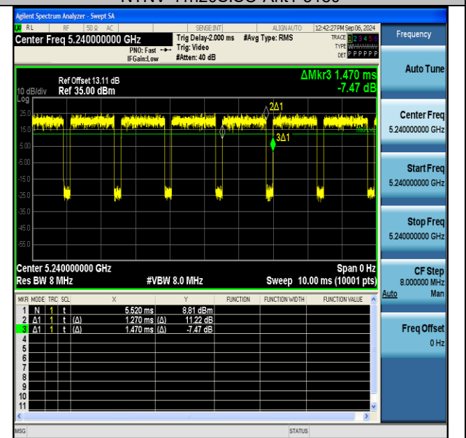
NTNV-11n20SISO-Ant1-5240
