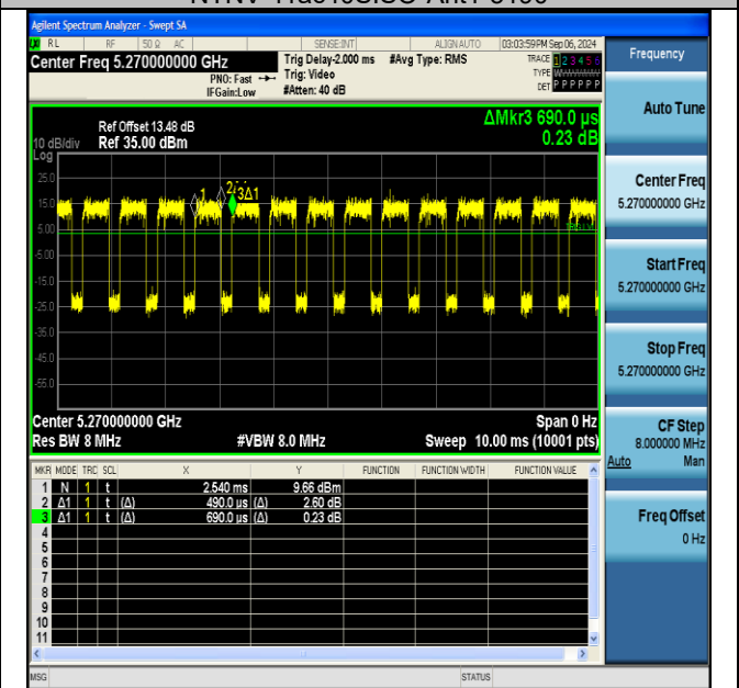
NTNV-11ac40SISO-Ant1-5270
