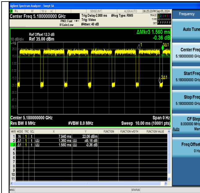
NTVN-11a-Ant1-5180
