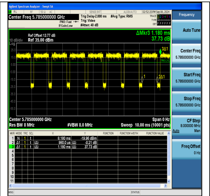
NTNV-11ac20SISO-Ant1-5785
