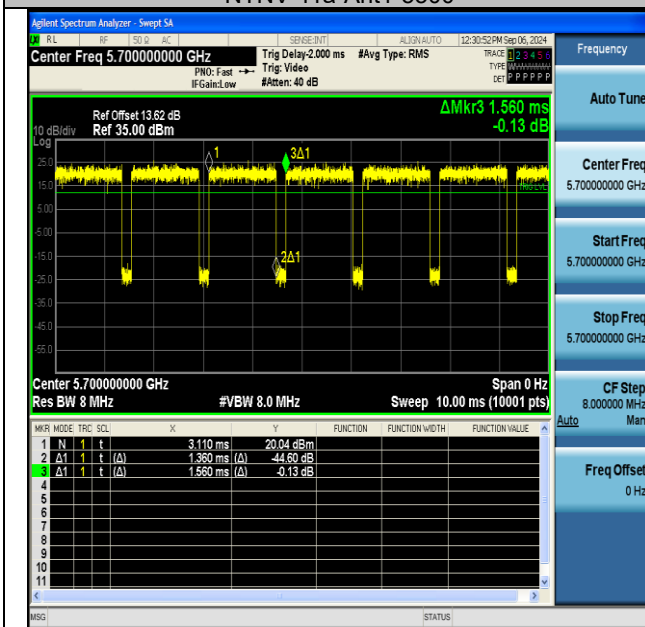
NTNV-11a-Ant1-5700
