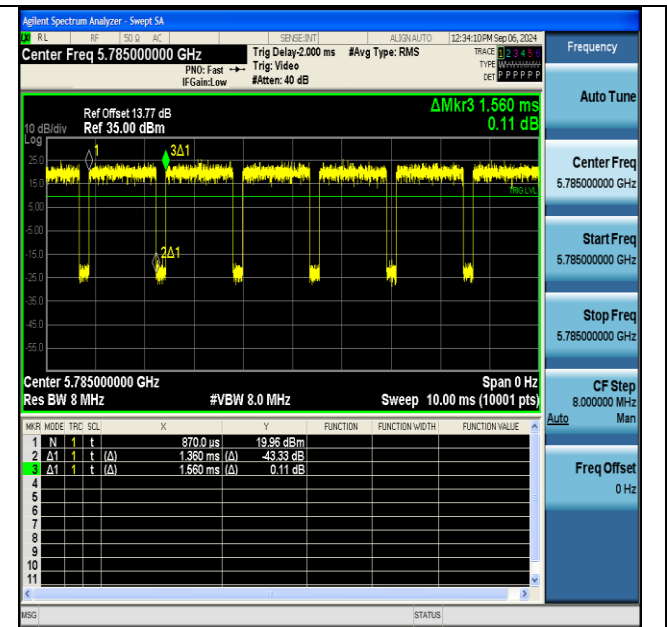
NTNV-11a-Ant1-5785
