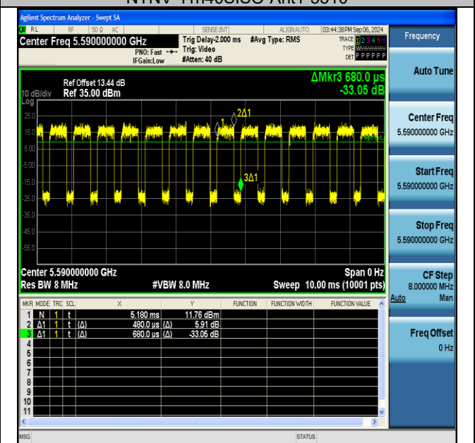
NTNV-11n40SISO-Ant1-5590
