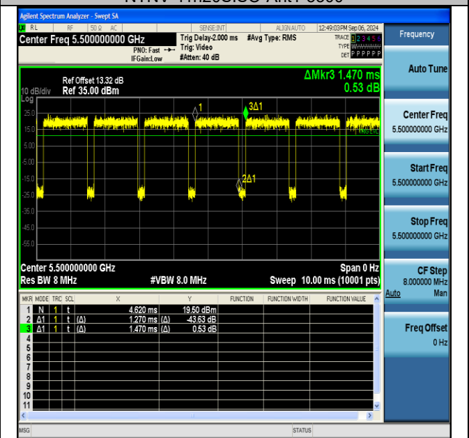
NTNV-11n20SISO-Ant1-5500
