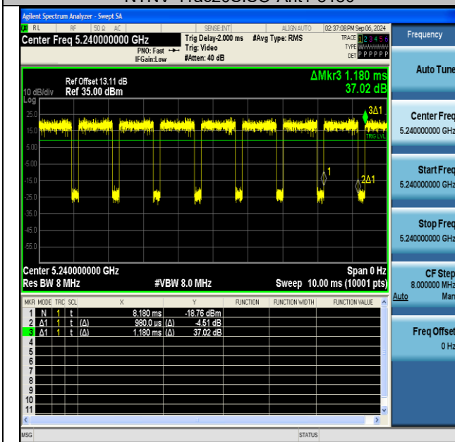
NTNV-11ac20SISO-Ant1-5240
