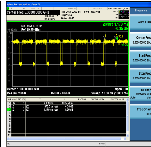
NTNV-11ac20SISO-Ant1-5300
