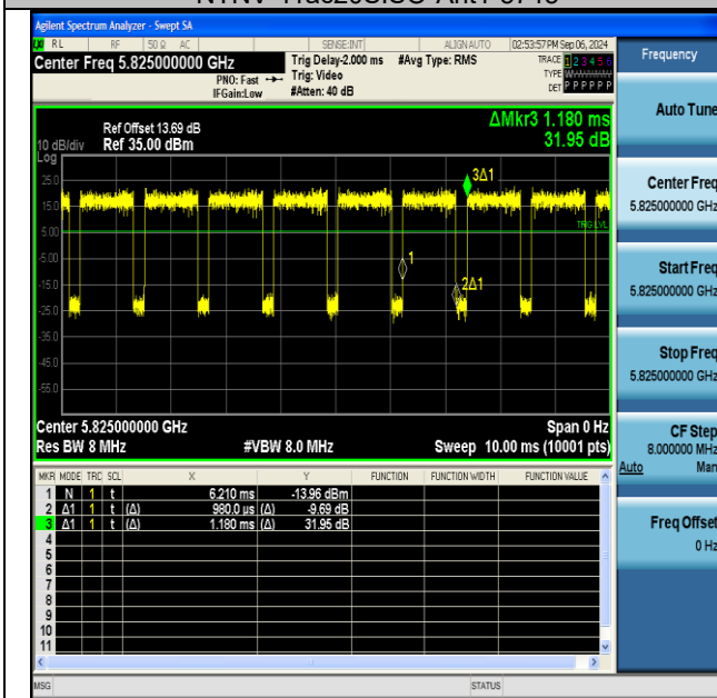
NTNV-11ac20SISO-Ant1-5825
