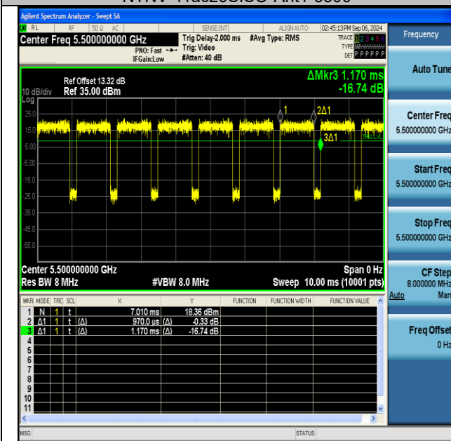
NTNV-11ac20SISO-Ant1-5500
