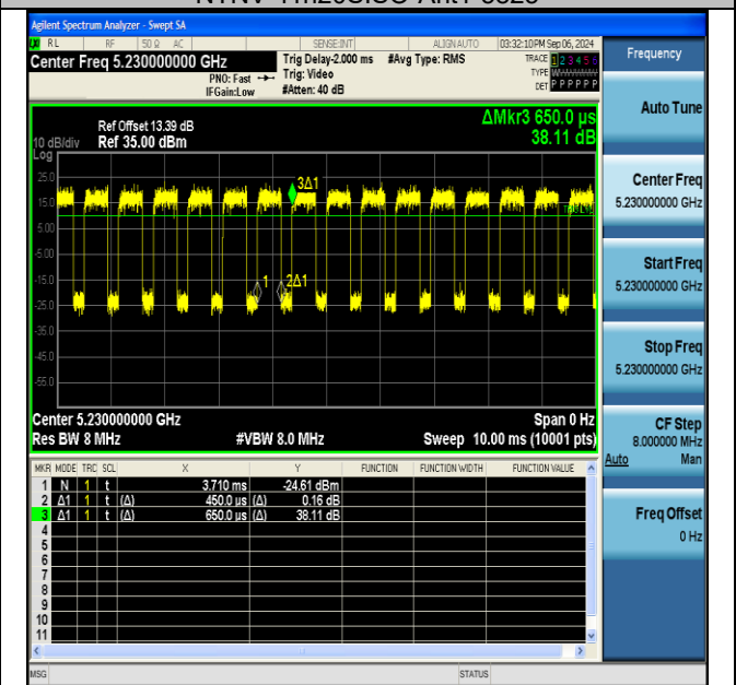
NTNV-11n40SISO-Ant1-5230
