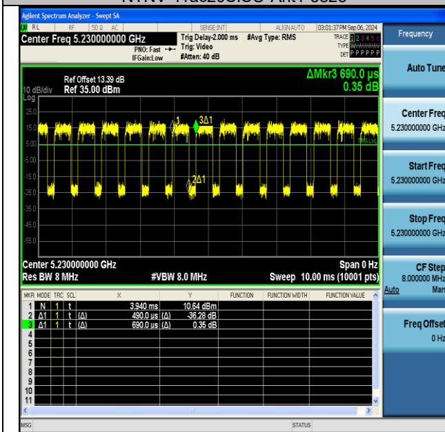
NTNV-11ac40SISO-Ant1-5230
