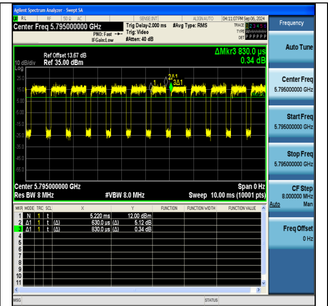
NTNV-11n40SISO-Ant1-5795
