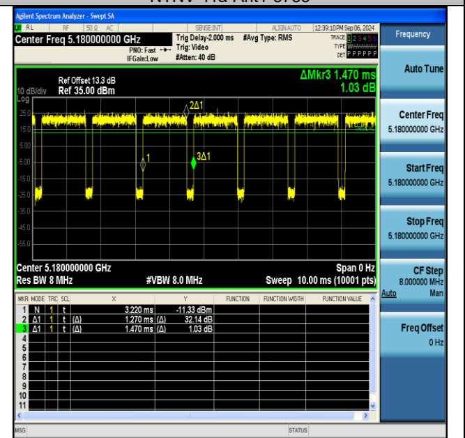
NTNV-11n20SISO-Ant1-5180
