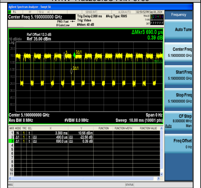
NTNV-11ac40SISO-Ant1-5190
