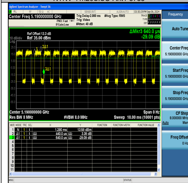
NTNV-11n40SISO-Ant1-5190
