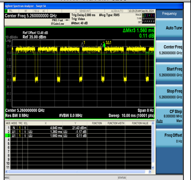
NTVN-11a-Ant1-5260
