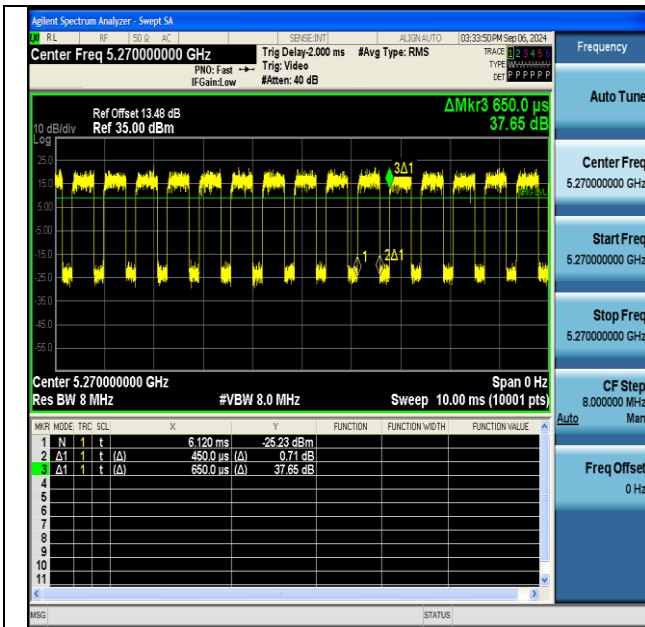
NTNV-11n40SISO-Ant1-5270
