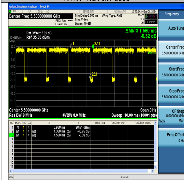
NTNV-11a-Ant1-5500
