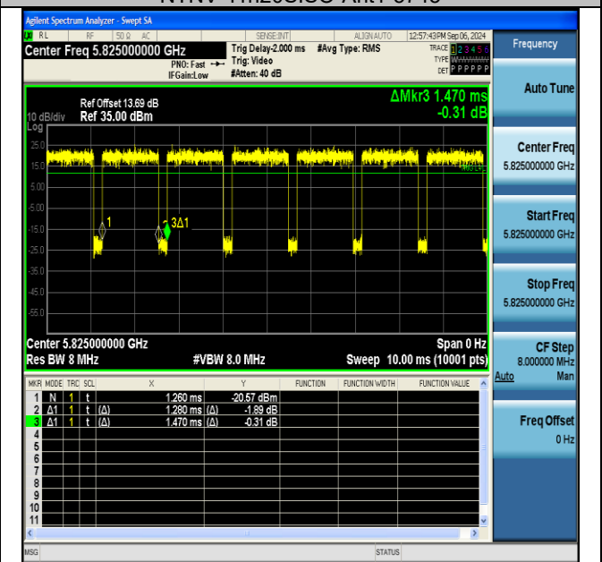
NTNV-11n20SISO-Ant1-5825
