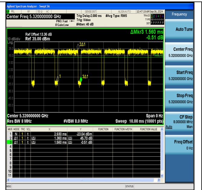
NTNV-11a-Ant1-5320
