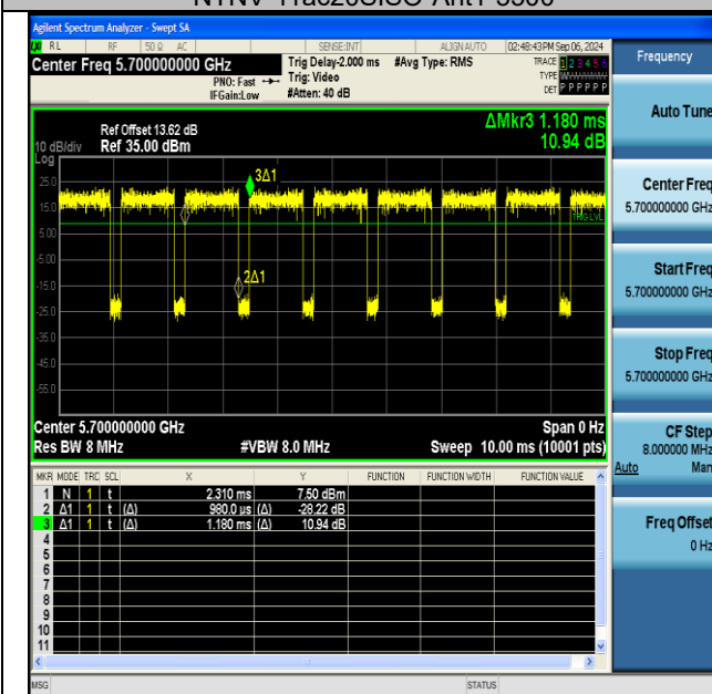
NTNV-11ac20SISO-Ant1-5700
