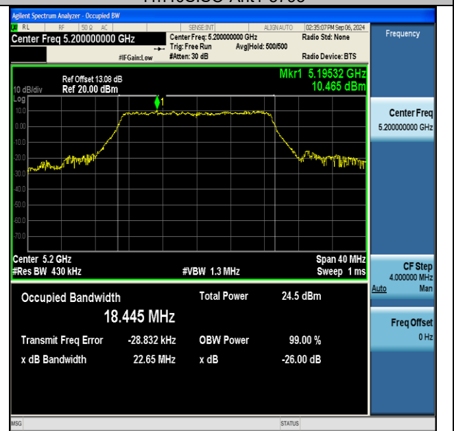
11ac20SISO-Ant1-5200
