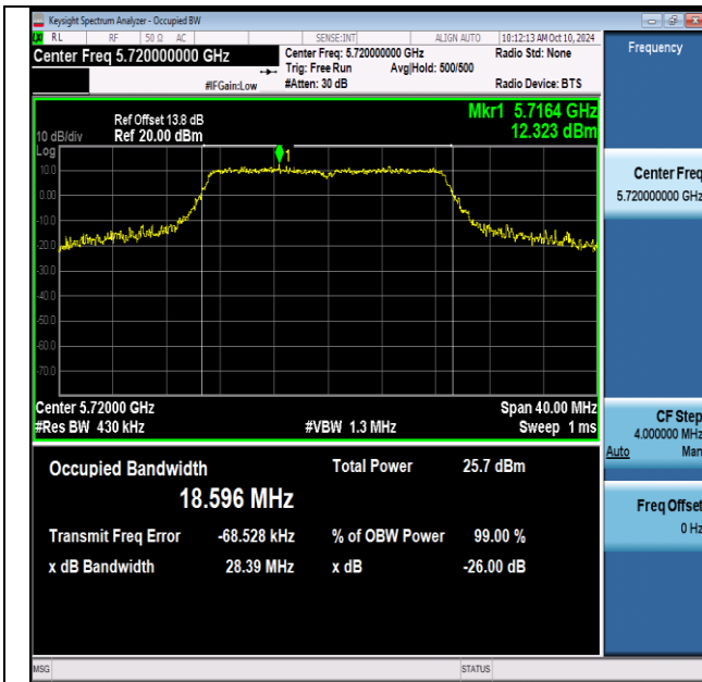
11n20SISO-Ant1-5720
