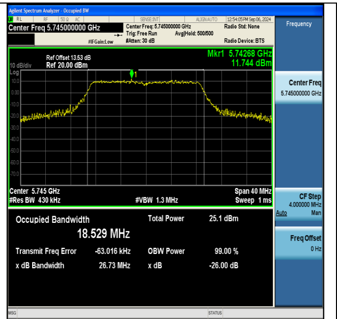
11n20SISO-Ant1-5745
