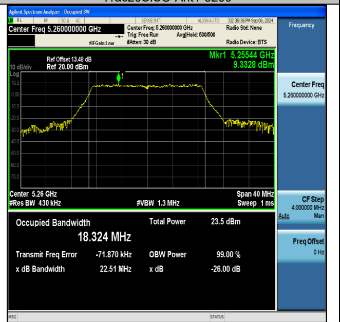
11ac20SISO-Ant1-5260
