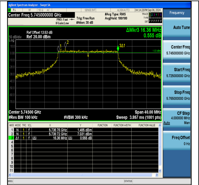
11a-Ant1-5745-PASS
