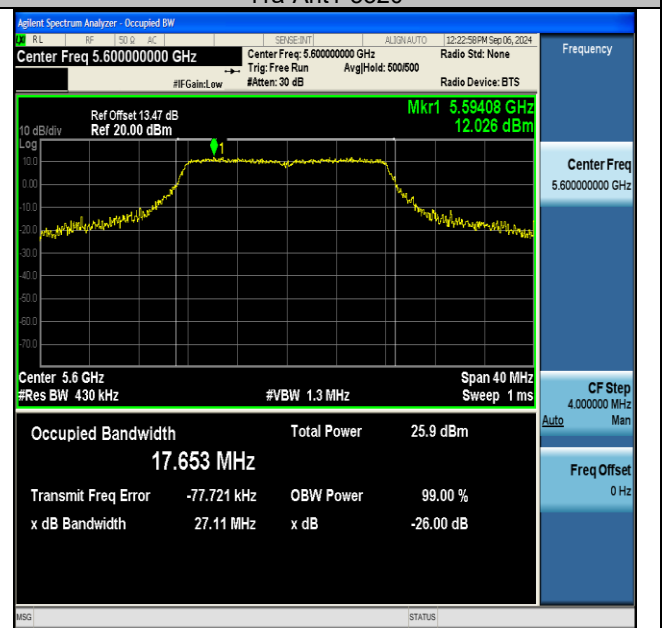
11a-Ant1-5600
