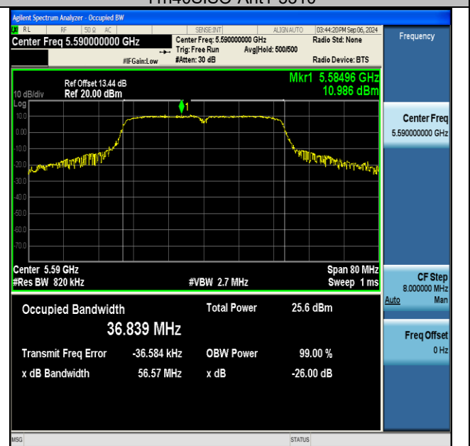
11n40SISO-Ant1-5590
