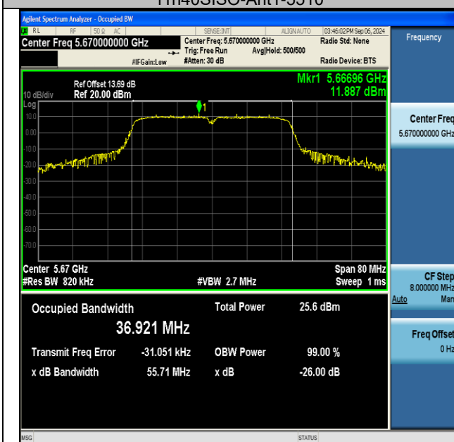
11n40SISO-Ant1-5670
