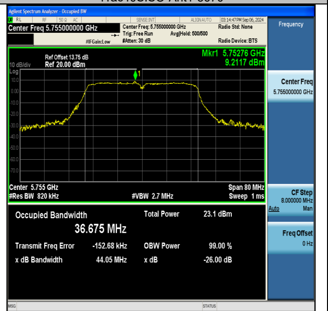
11ac40SISO-Ant1-5755
