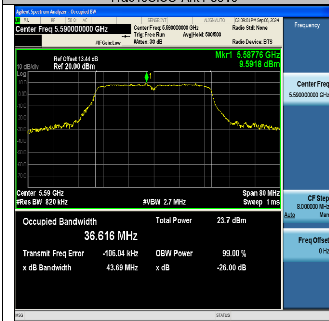
11ac40SISO-Ant1-5590
