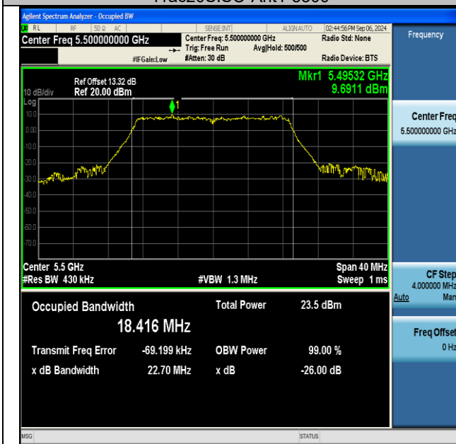
11ac20SISO-Ant1-5500
