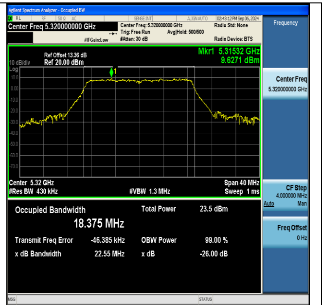
11ac20SISO-Ant1-5320
