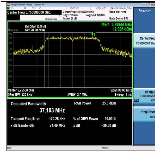
11n40SISO-Ant1-5755
