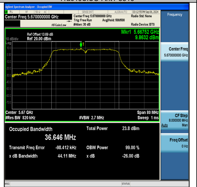
11ac40SISO-Ant1-5670
