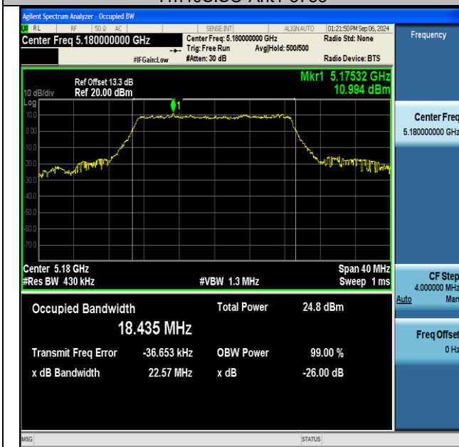
11ac20SISO-Ant1-5180
