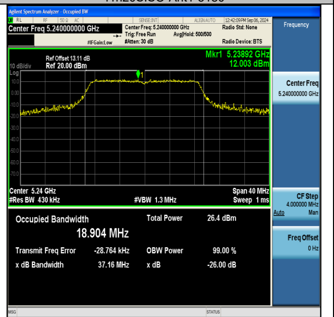
11n20SISO-Ant1-5240
