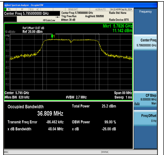
11n40SISO-Ant1-5795
