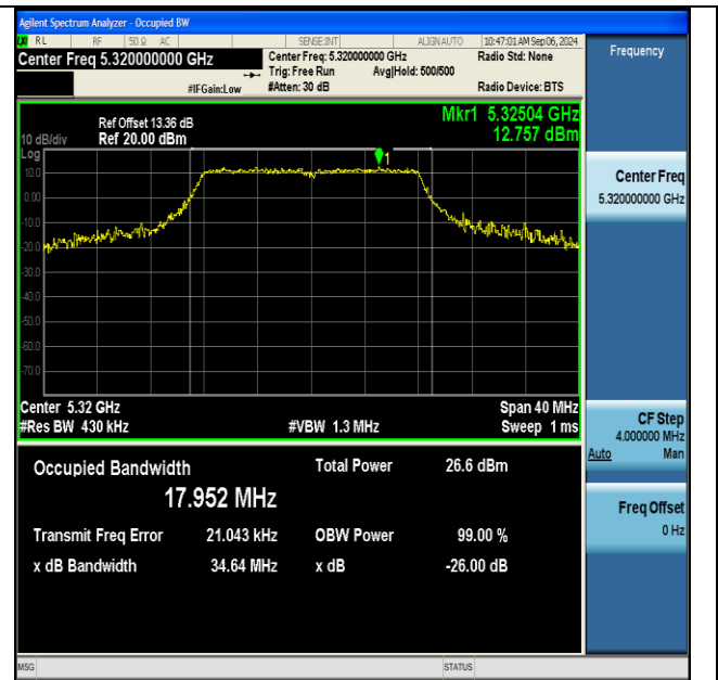
11a-Ant1-5320
