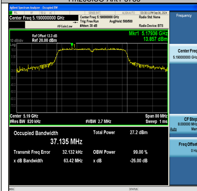
11n40SISO-Ant1-5190
