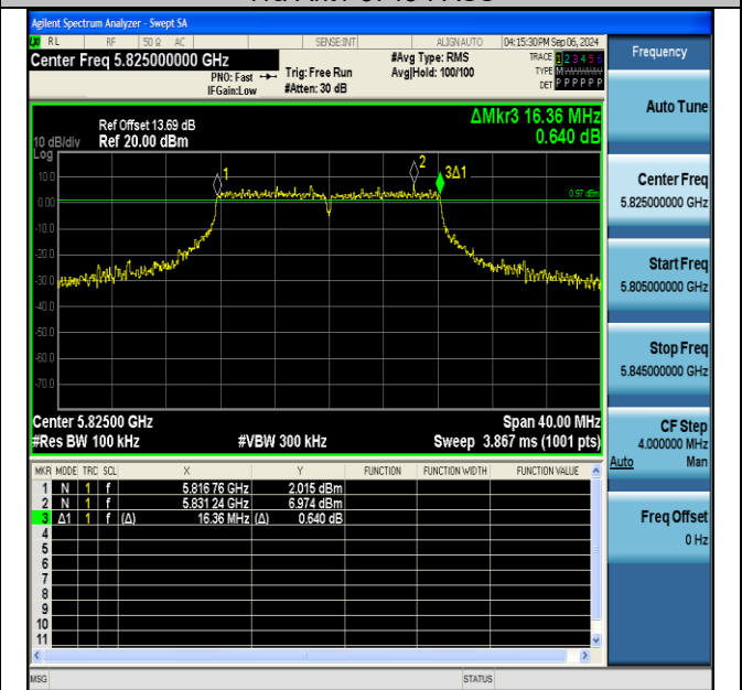
11a-Ant1-5825-PASS
