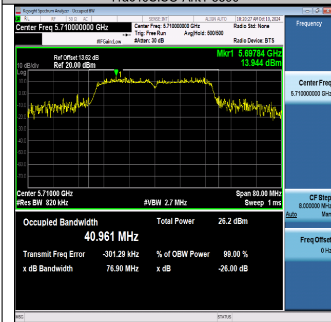
11ac40SISO-Ant1-5710
