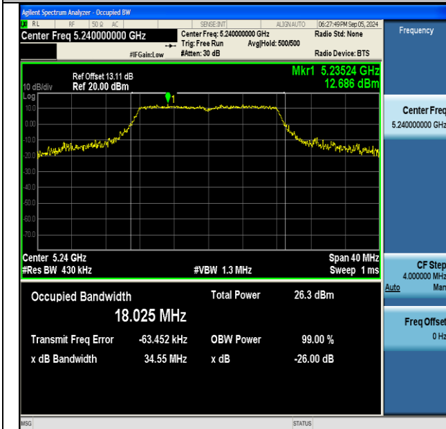
11a-Ant1-5240
