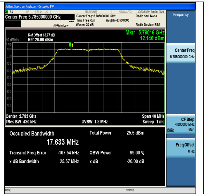
11a-Ant1-5785
