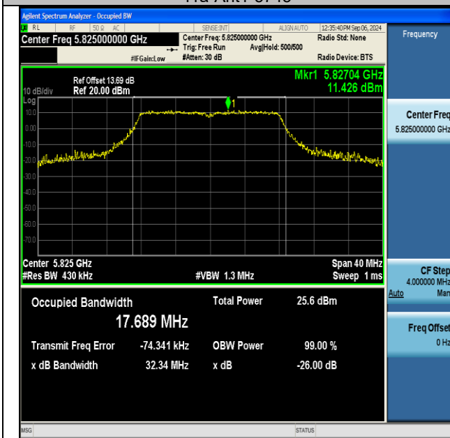
11a-Ant1-5825
