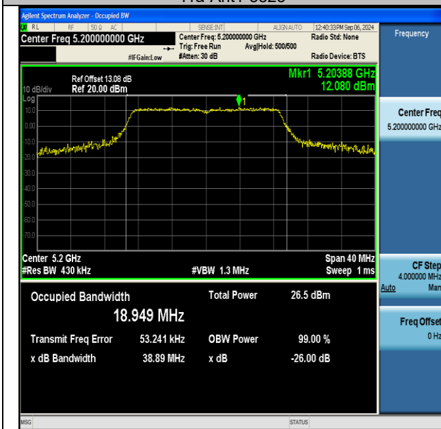
11n20SISO-Ant1-5200
