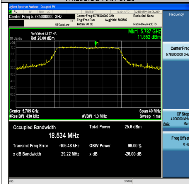
11n20SISO-Ant1-5785
