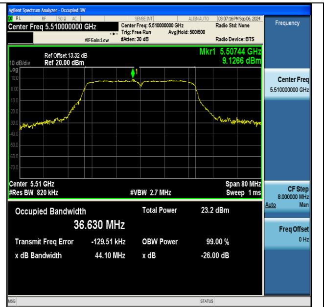
11ac40SISO-Ant1-5510
