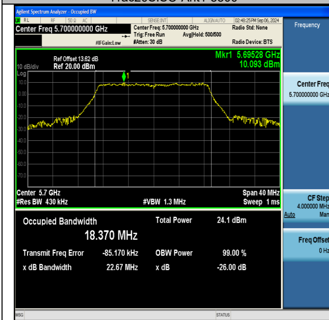
11ac20SISO-Ant1-5700
