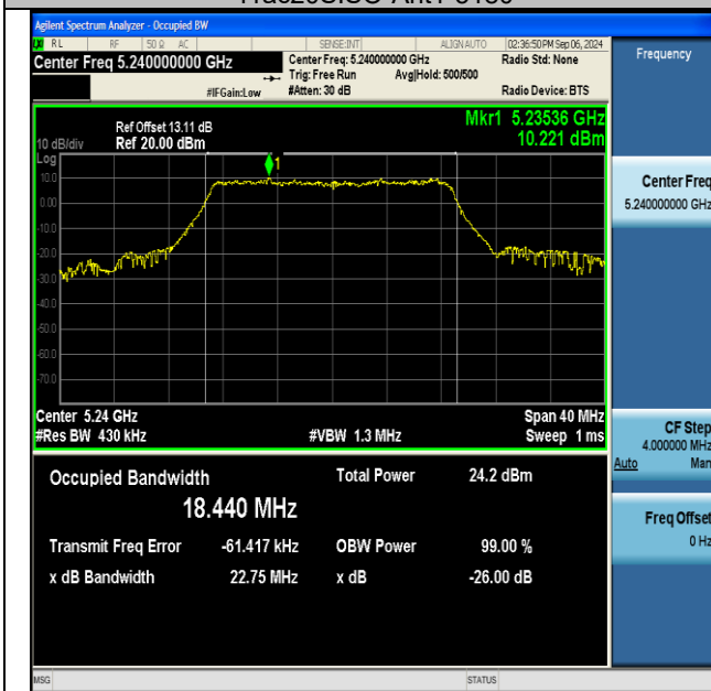
11ac20SISO-Ant1-5240
