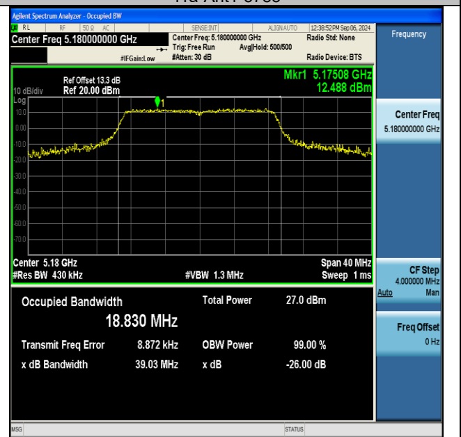
11n20SISO-Ant1-5180
