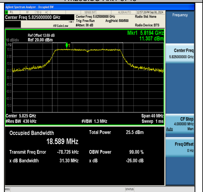
11n20SISO-Ant1-5825
