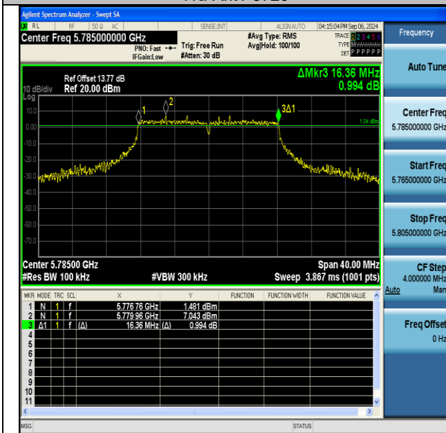
11a-Ant1-5785-PASS
