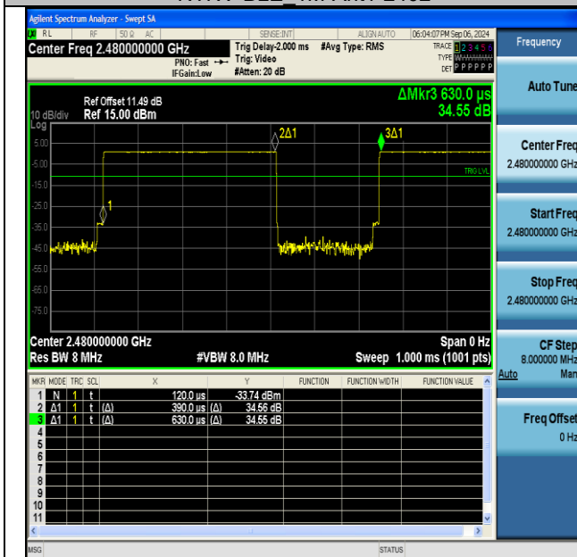
NTVN-BLE_1M-Ant1-2480
