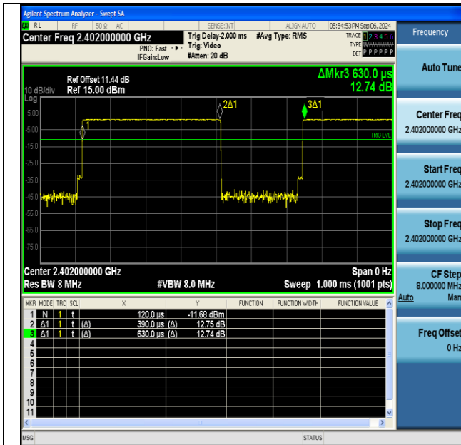
NTVN-BLE_1M-Ant1-2402
