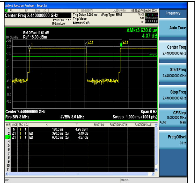
NTVN-BLE_1M-Ant1-2440
