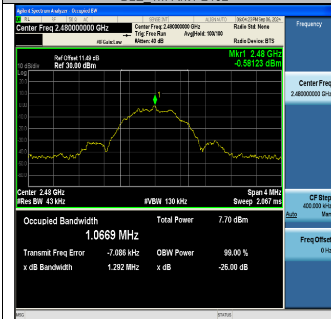
BLE_1M-Ant1-2480
