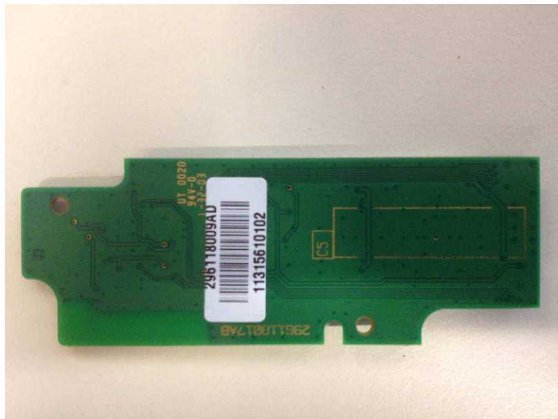
Details views of RF PCB with an without shield (Bluetooth)
