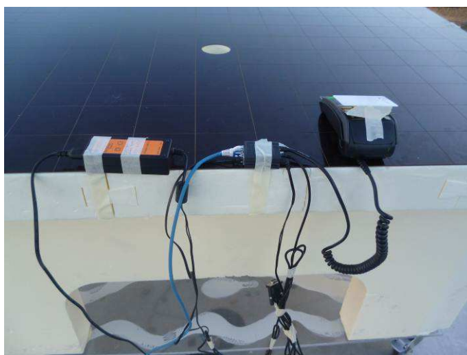
Radiated emission test setup
