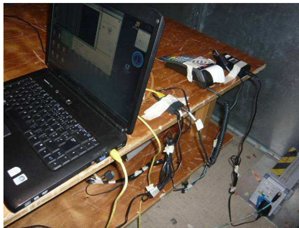
Conducted emission test setup
