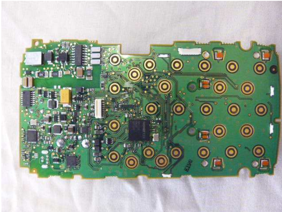
General PCB views
