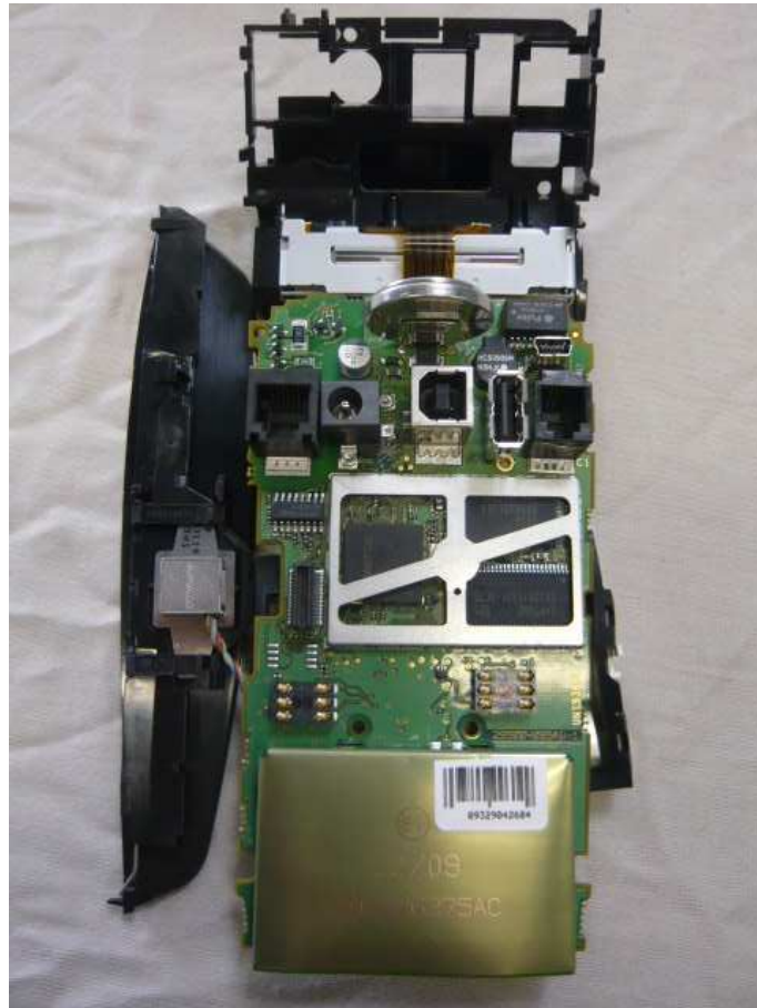
Views without enclosure
