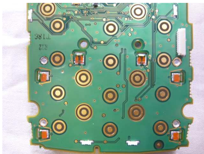
Detail PCB views
