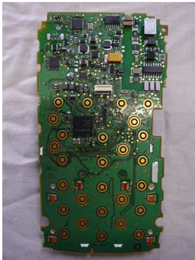
PCB detail views
