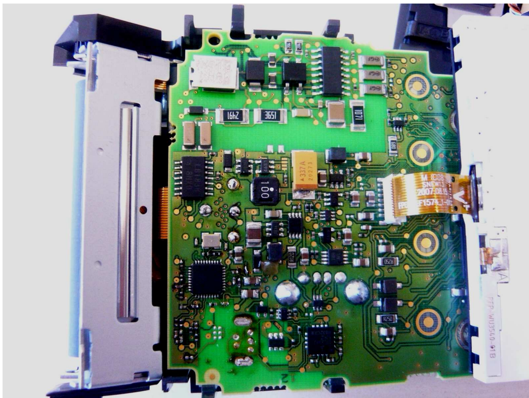
Component view, behind LCD
