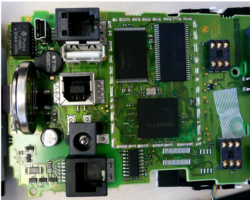
Component view, lower face
