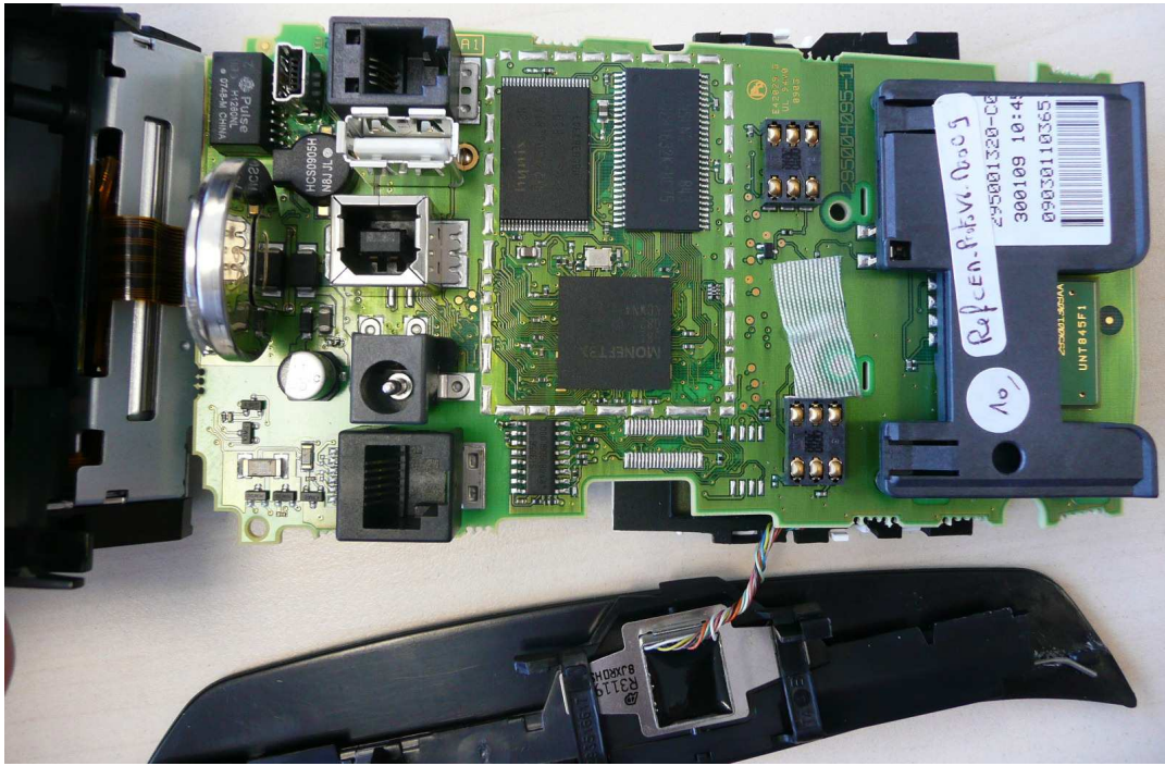
Component view, lower face
