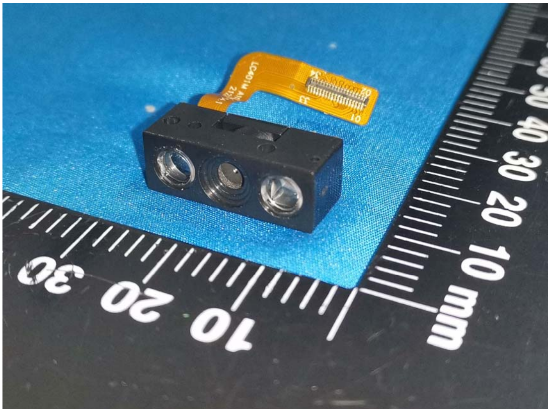
Scanner Reader
