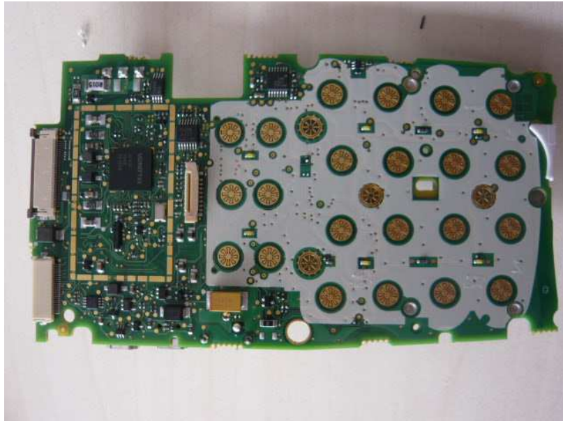
Detail views PCB
