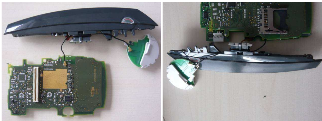
Detail views Bluetooth antenna and connector with magnetic reader
