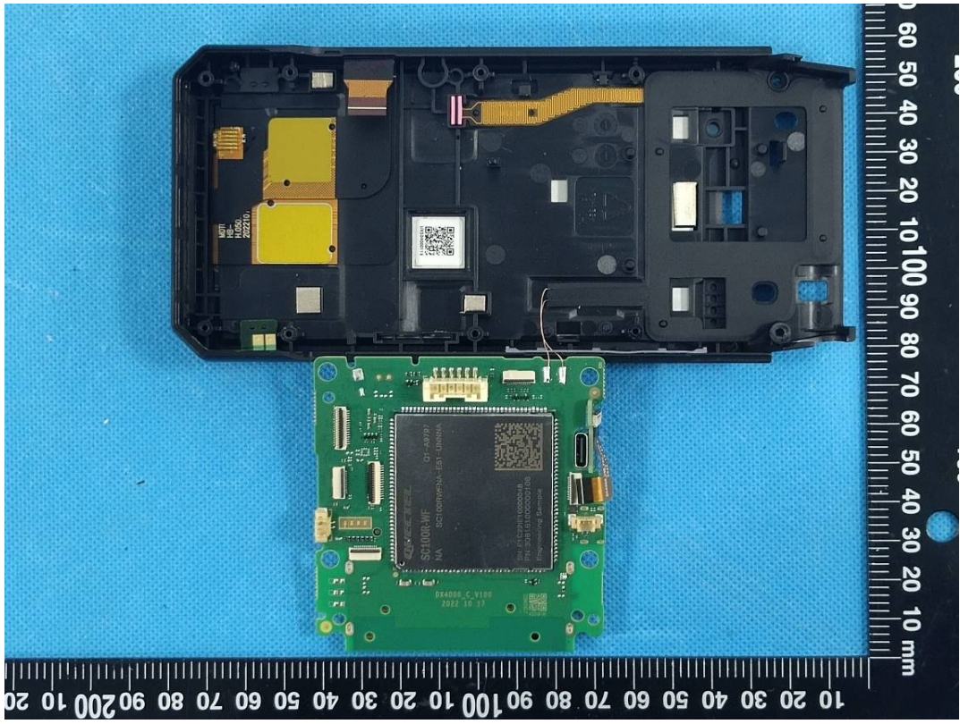
WiFi/BT Antenna
