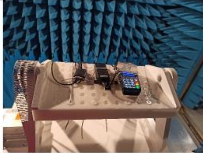
Photo Setup : anechoic chamber (XY axis)
