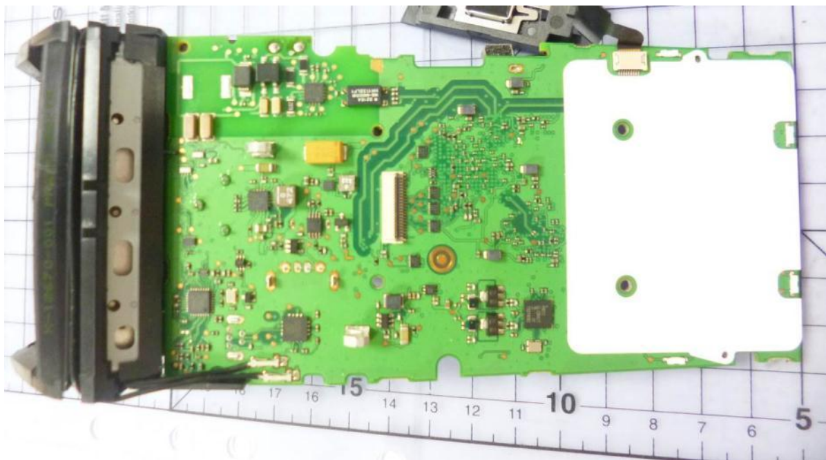
Desk 5000 : UC board PWB
