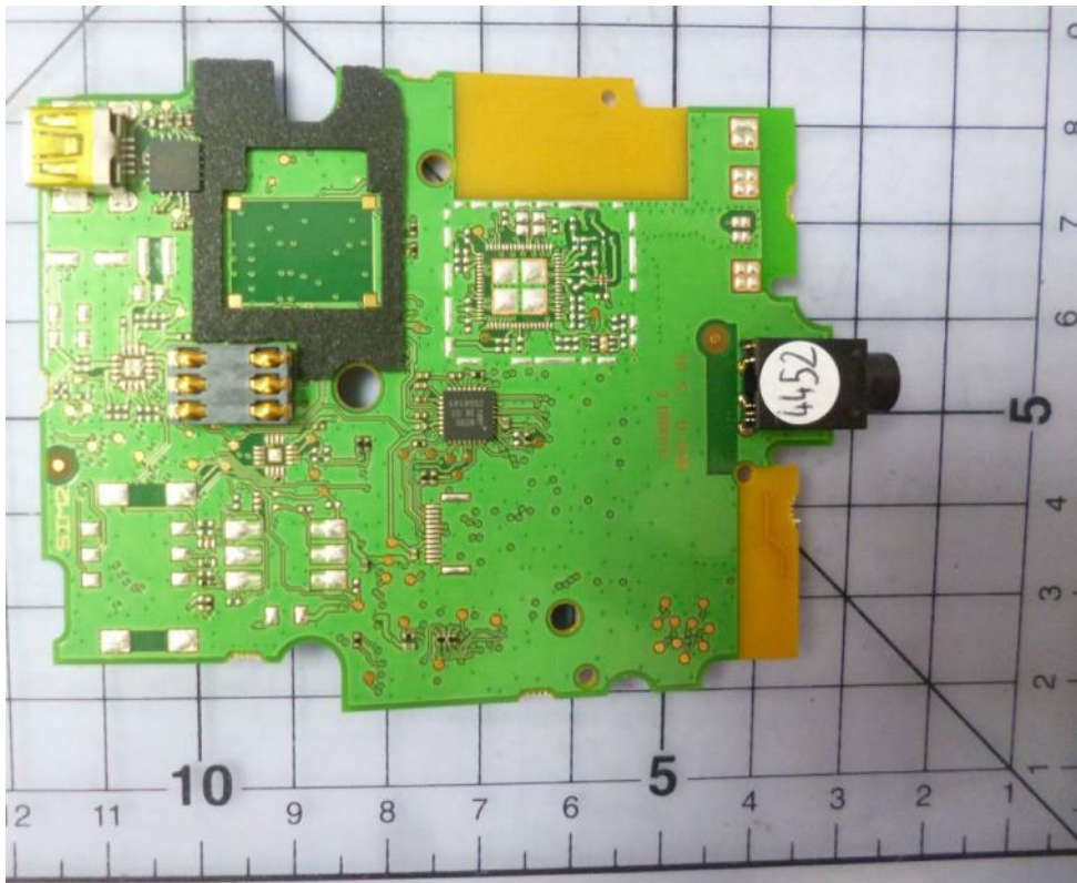
Desk 5000 : board PWB
