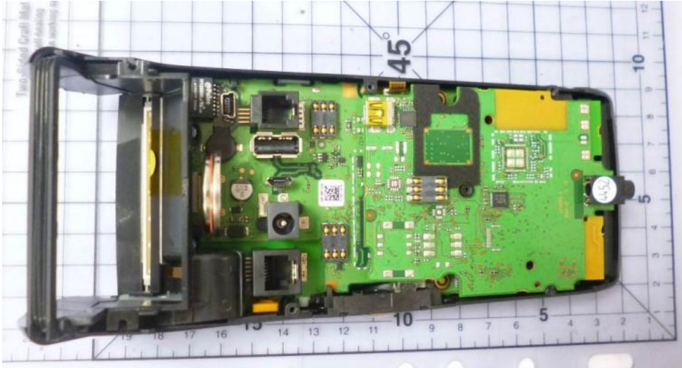
Desk 5000 : Inside view UC board
