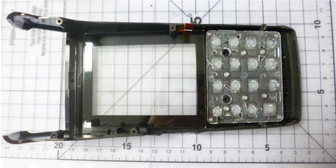
Desk 5000: Front enclosure and keypad view
