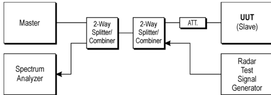
Figure 1: Setup
