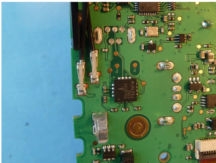
Photo 11: antenna ports
