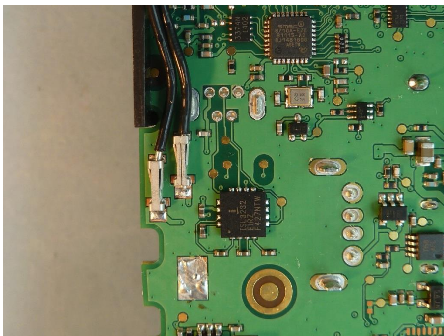
Photo 10: antenna ports
