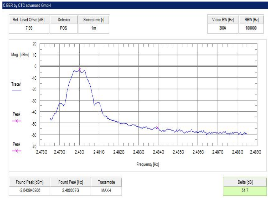
Plot 2: Upper band edge, 1 Msp
