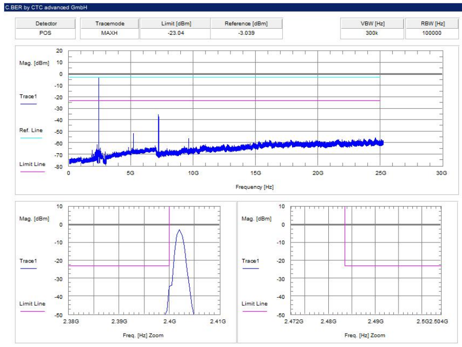
Plot 4: lowest channel, 2 Msp
