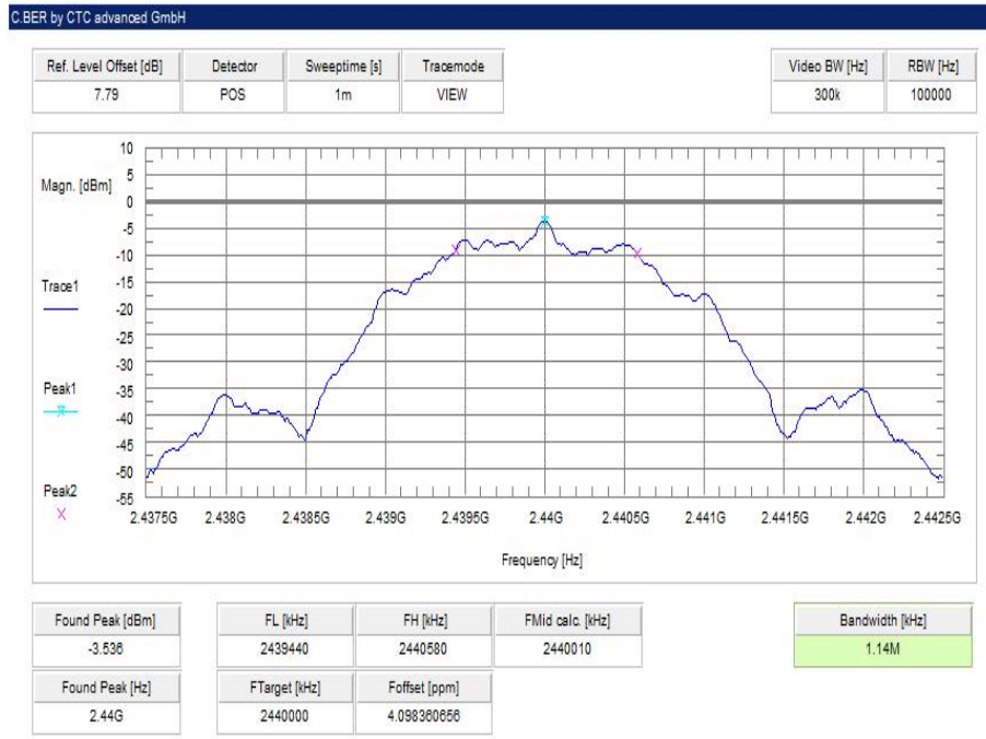
Plot 5: mid channel, 2 Msp
