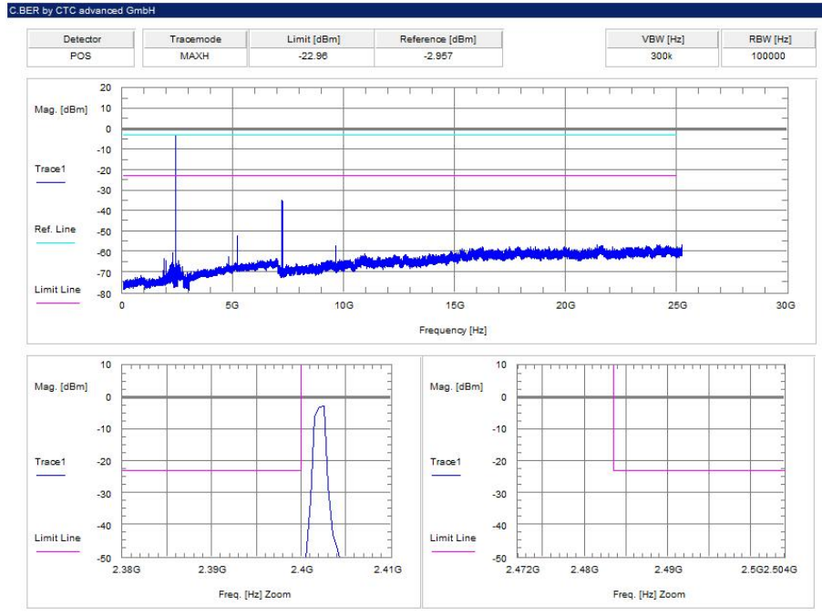
Plot 1: lowest channel, 1 Msp
