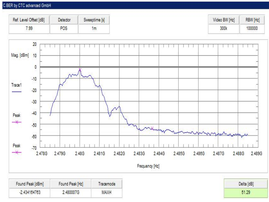
Plot 4: Upper band edge, 2 Msp
