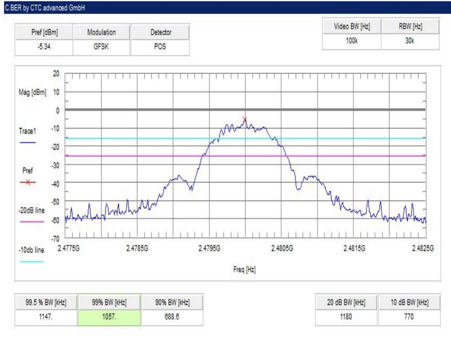
Plot 3: highest channel, 1 Msp
