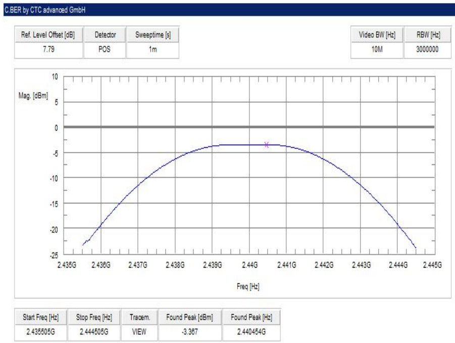
Plot 5: mid channel, 2 Msps
