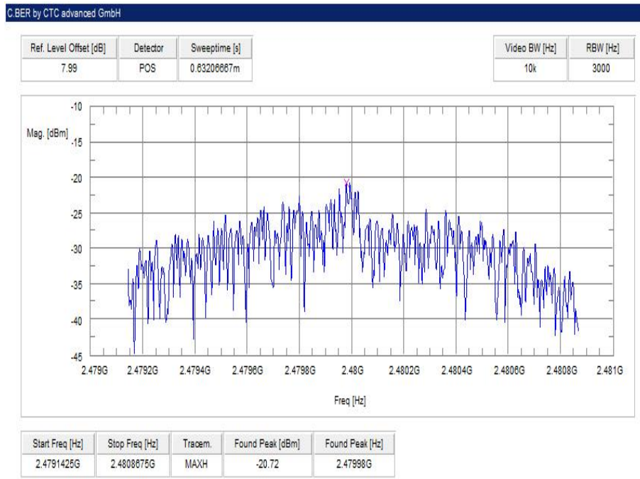
Plot 6: highest channel, 2 Msps
