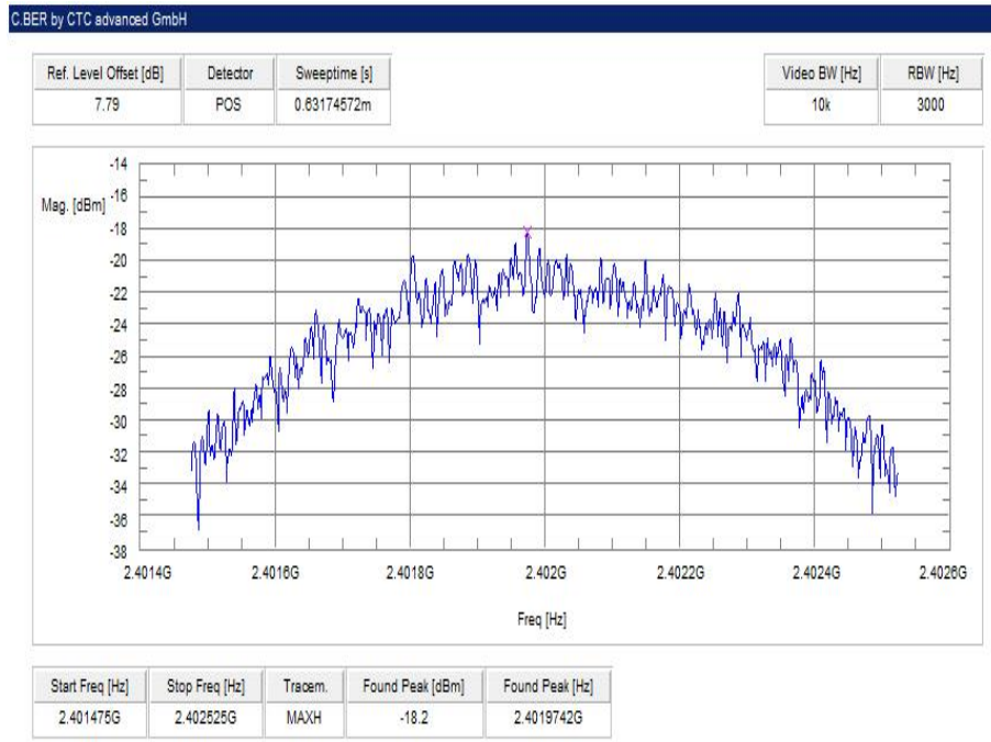
Plot 1: lowest channel, 1 Msps
