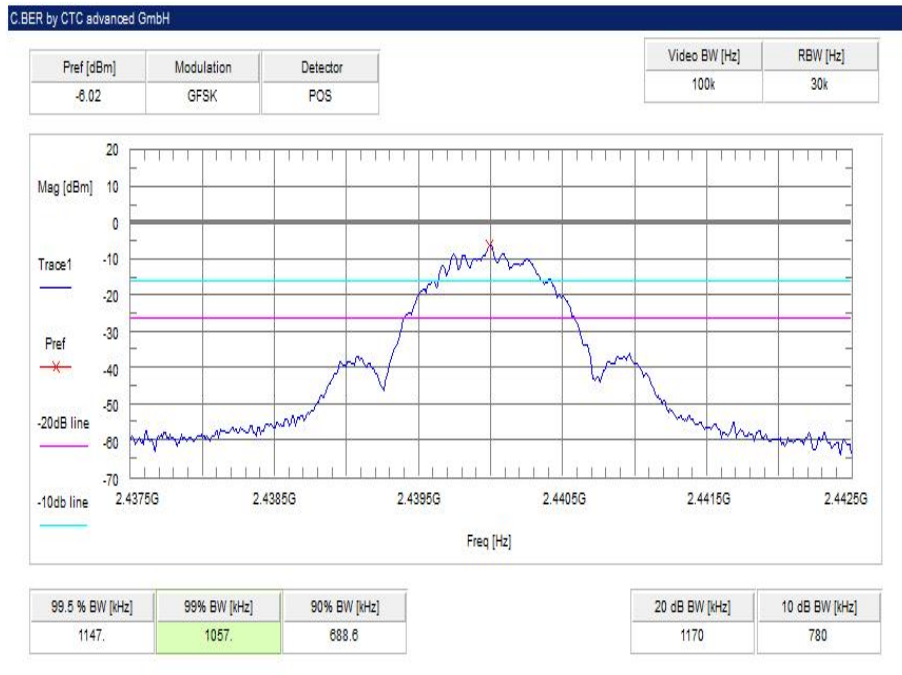
Plot 2: mid channel, 1 Msps
