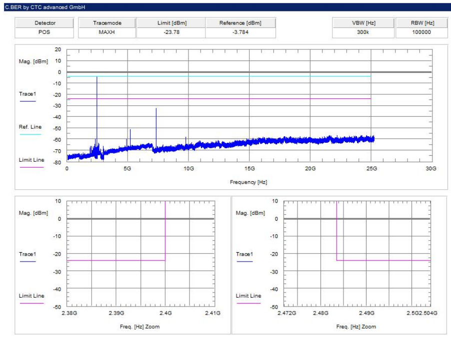
Plot 2: mid channel, 1 Msp
