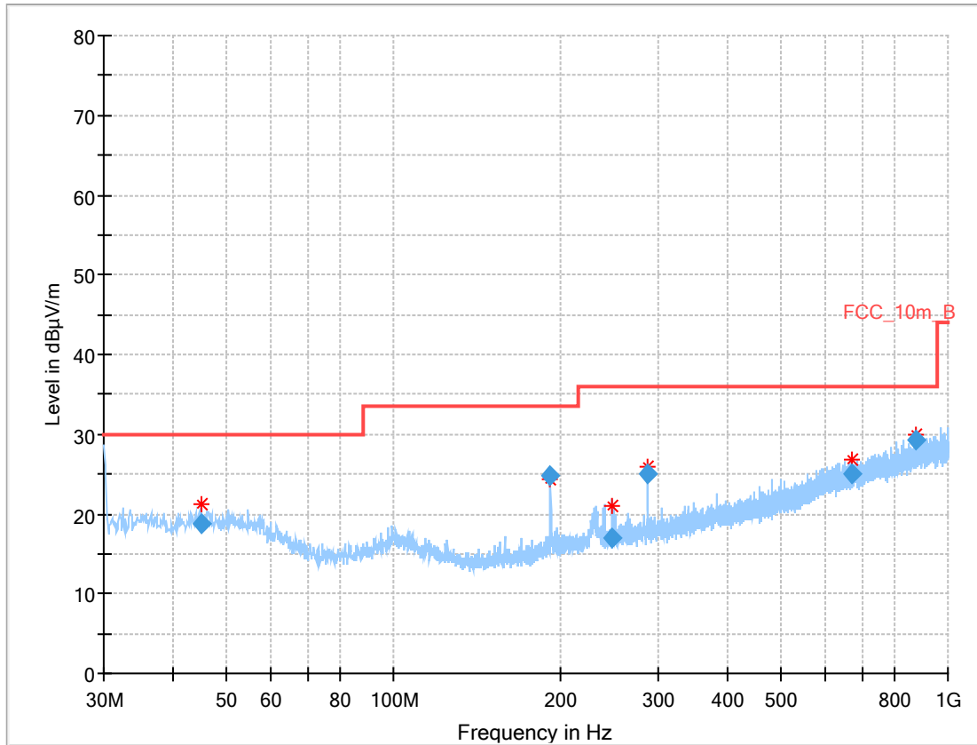
Plot 4: 30 MHz to 1 GHz, TX mode, 2402 MHz, vertical & horizontal polarization, 2 Msp
