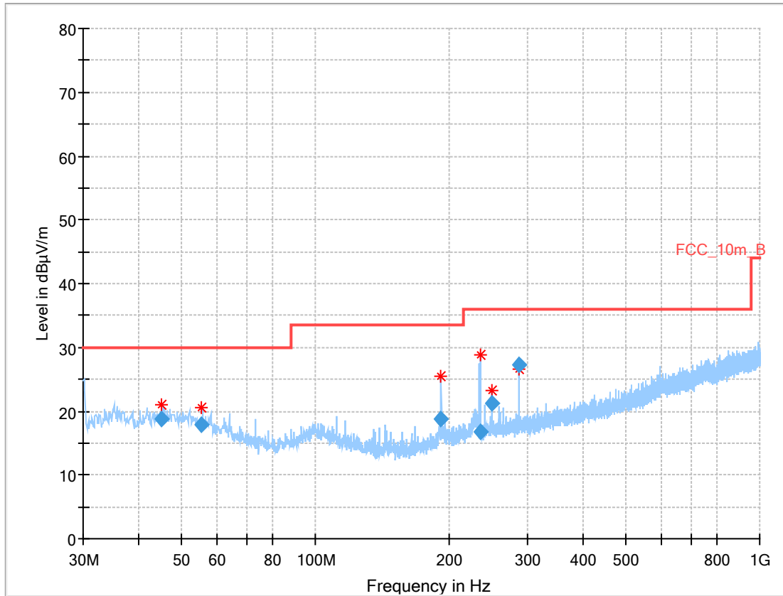
Plot 5: 30 MHz to 1 GHz, TX mode, 2440 MHz, vertical & horizontal polarization, 2 Msp
