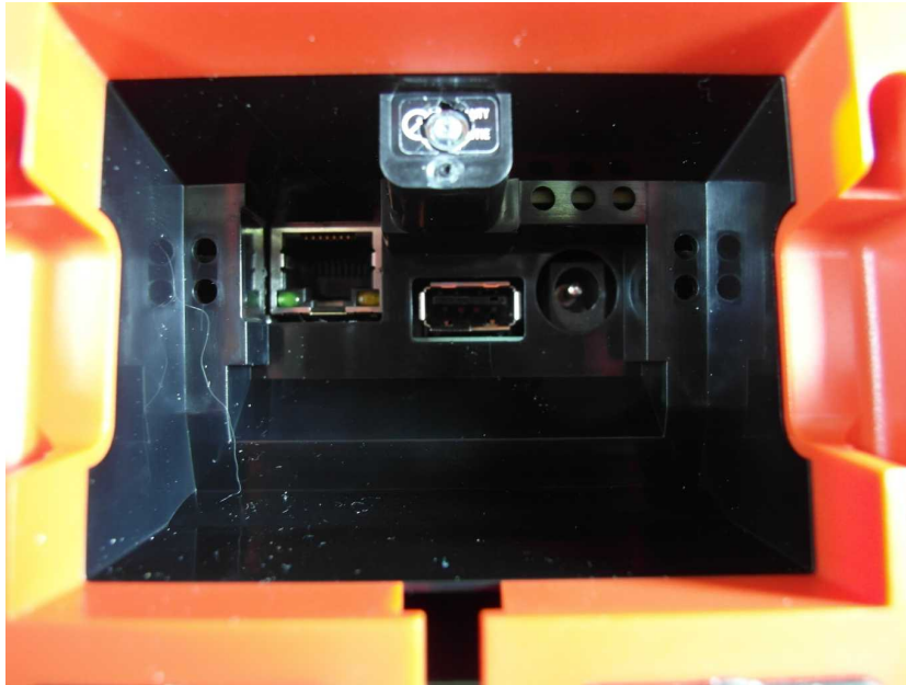
Photo 7: Connection ports
