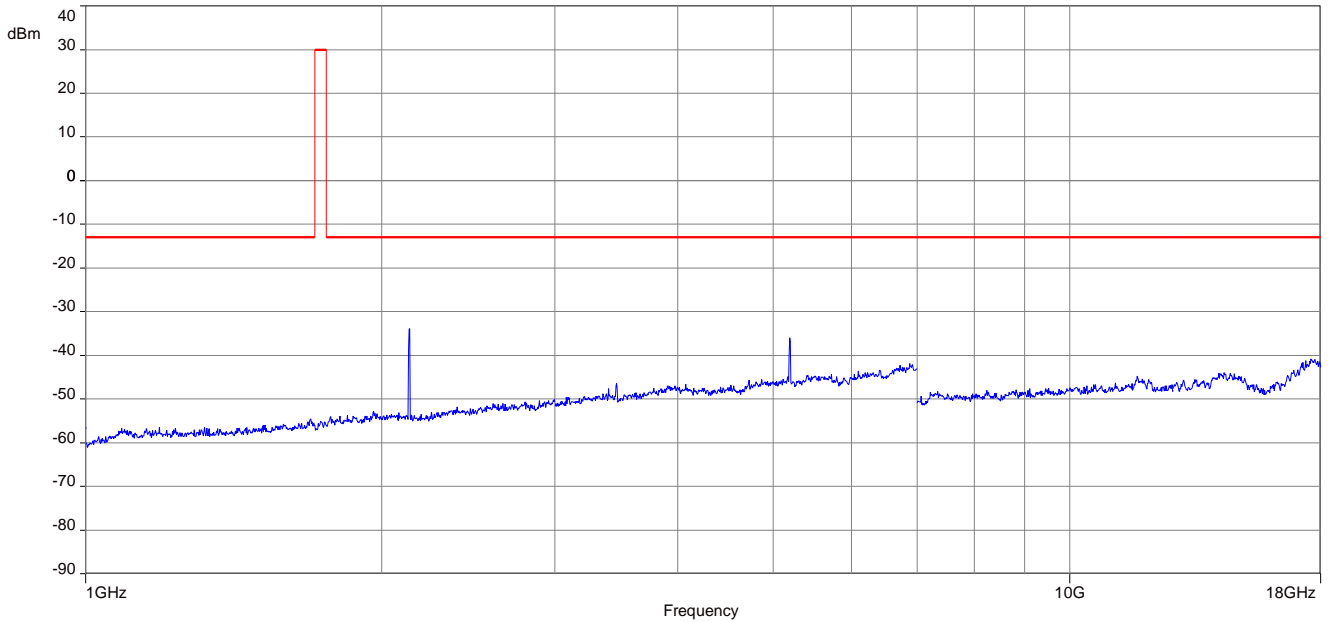
Carrier notched with 1.75 GHz rejection filter
