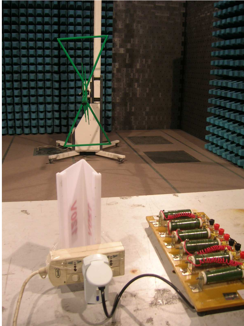
Radiated emission, 30MHz-1000MHz
