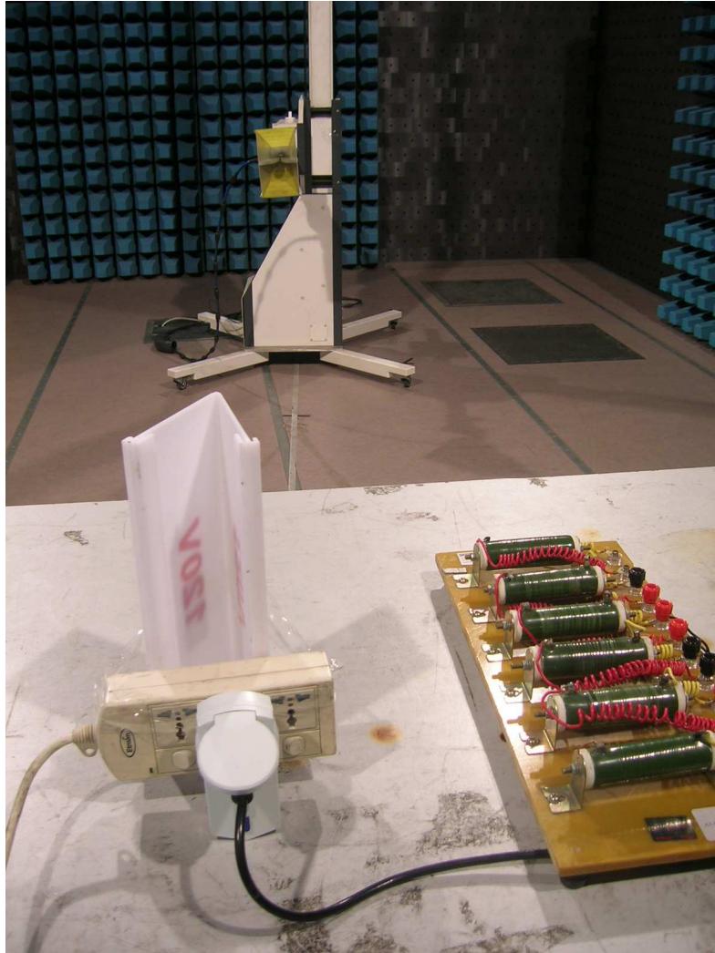
Radiated emission, 1GHz-5GHz
