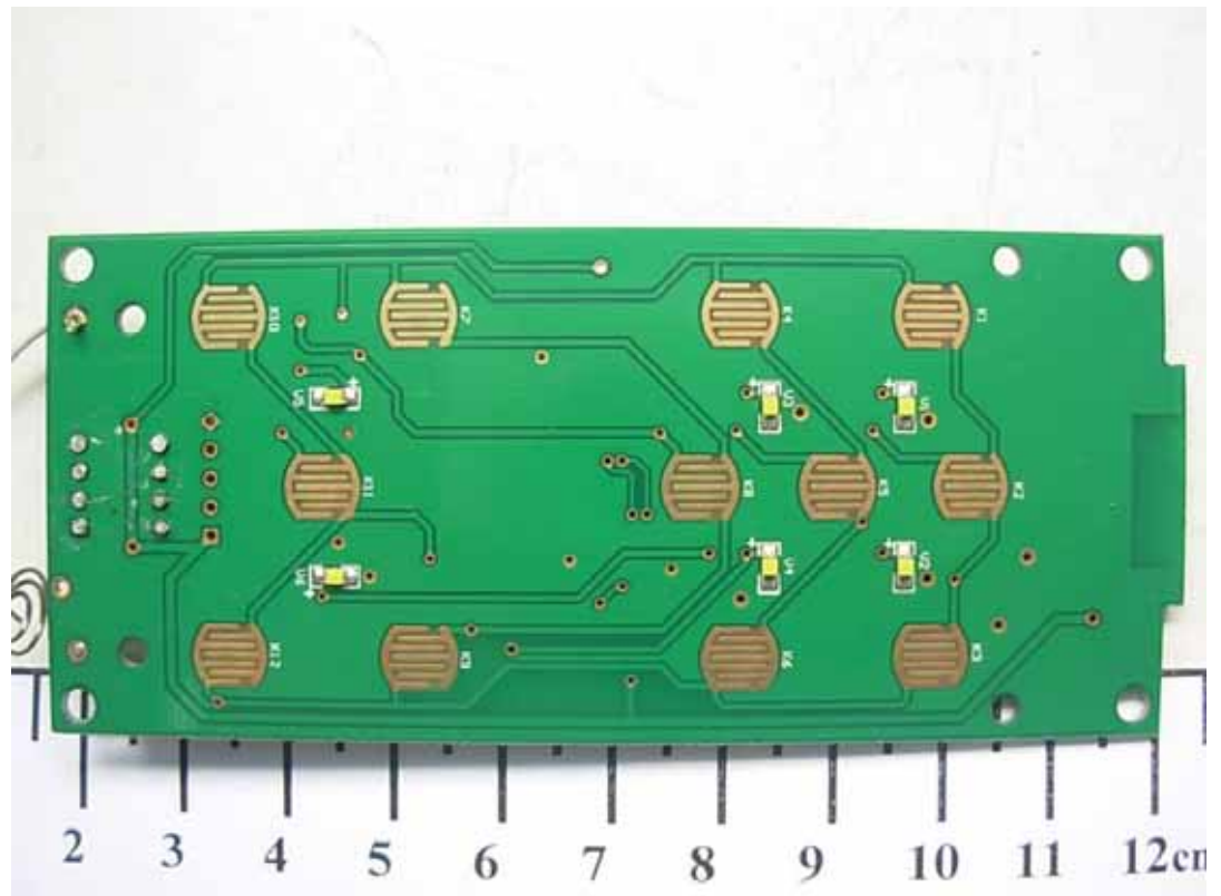
REMOTE CONTROLLER (M/N: BCYK001) MAIN BOARD (COMPONENT SIDE)
