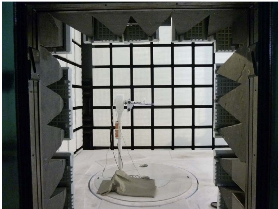
Photo 9: EUT with external rubber antenna in the anechoic chamber
