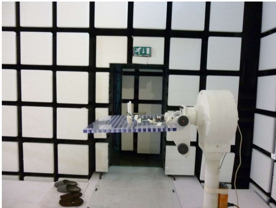
Photo 19: EUT with external PCB antenna in the anechoic chamber
