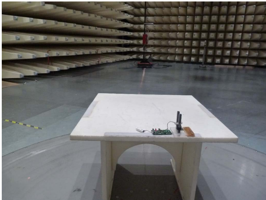
Photo 7: EUT with internal antenna in the semi-anechoic chamber
