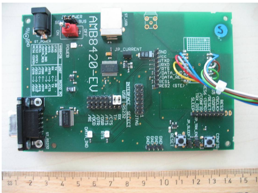
Photo 11: Extender board
