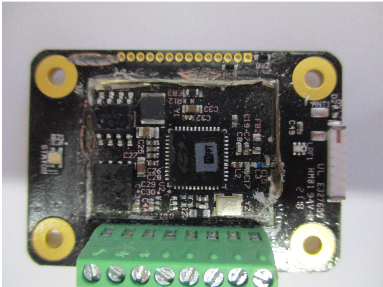
Module PCB with RF Shield Removed
