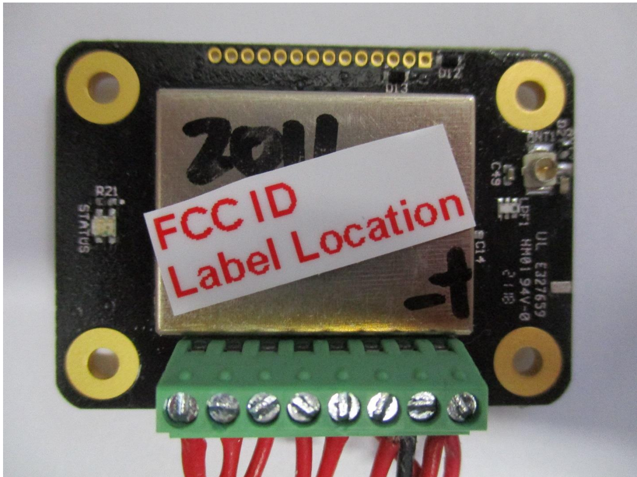
Module PCB with External Antenna Port, Top
