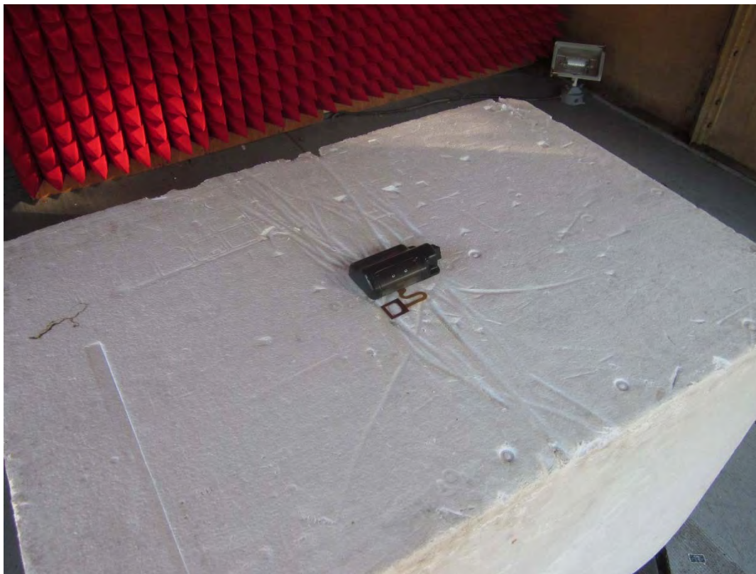
Test Setup
