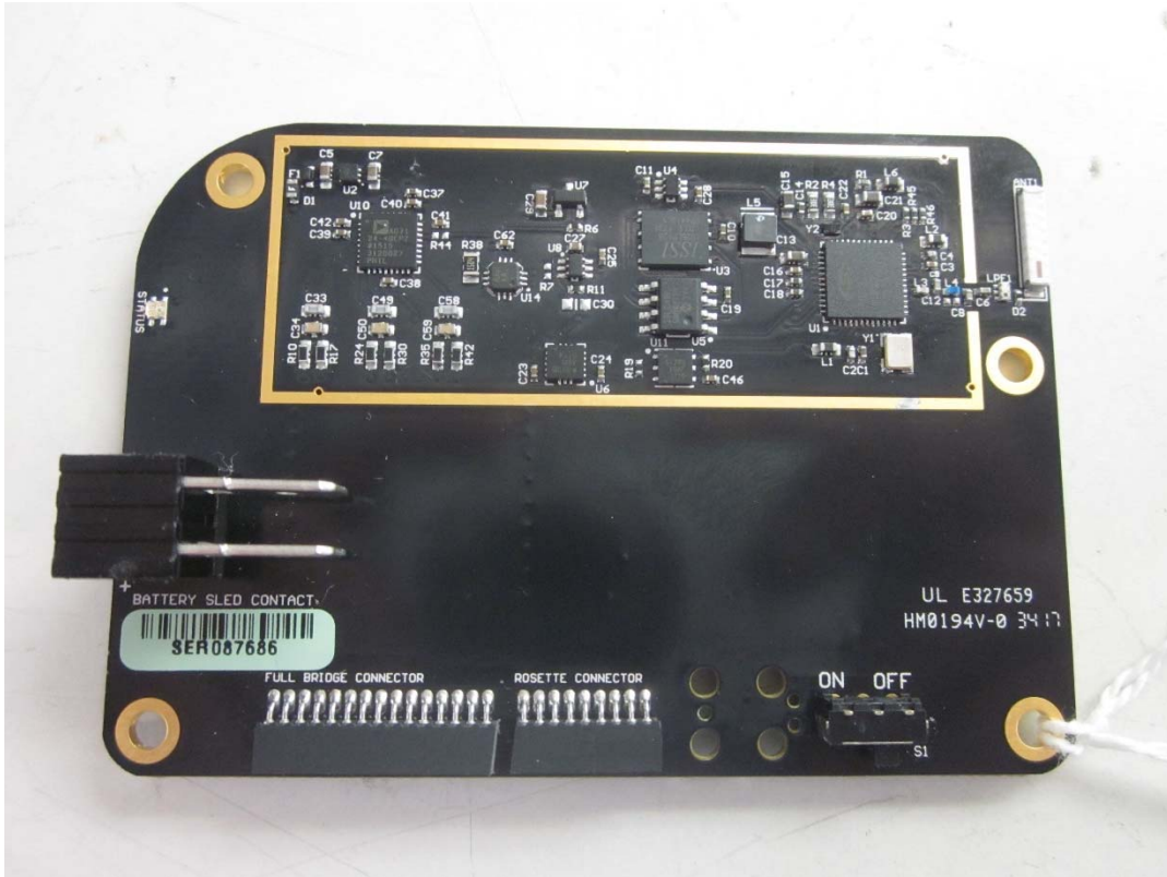
Internal Main PCB Top
