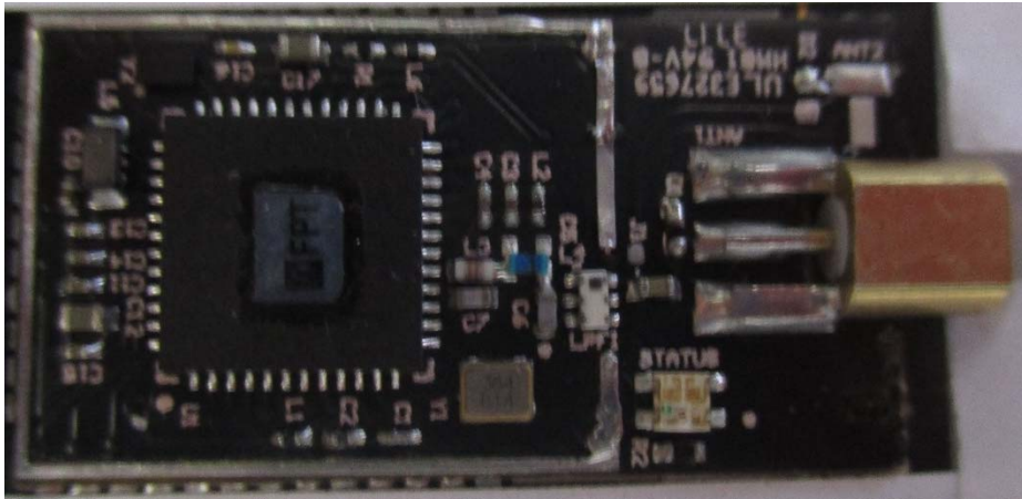
Module PCB with External Antenna, Shield Removed
