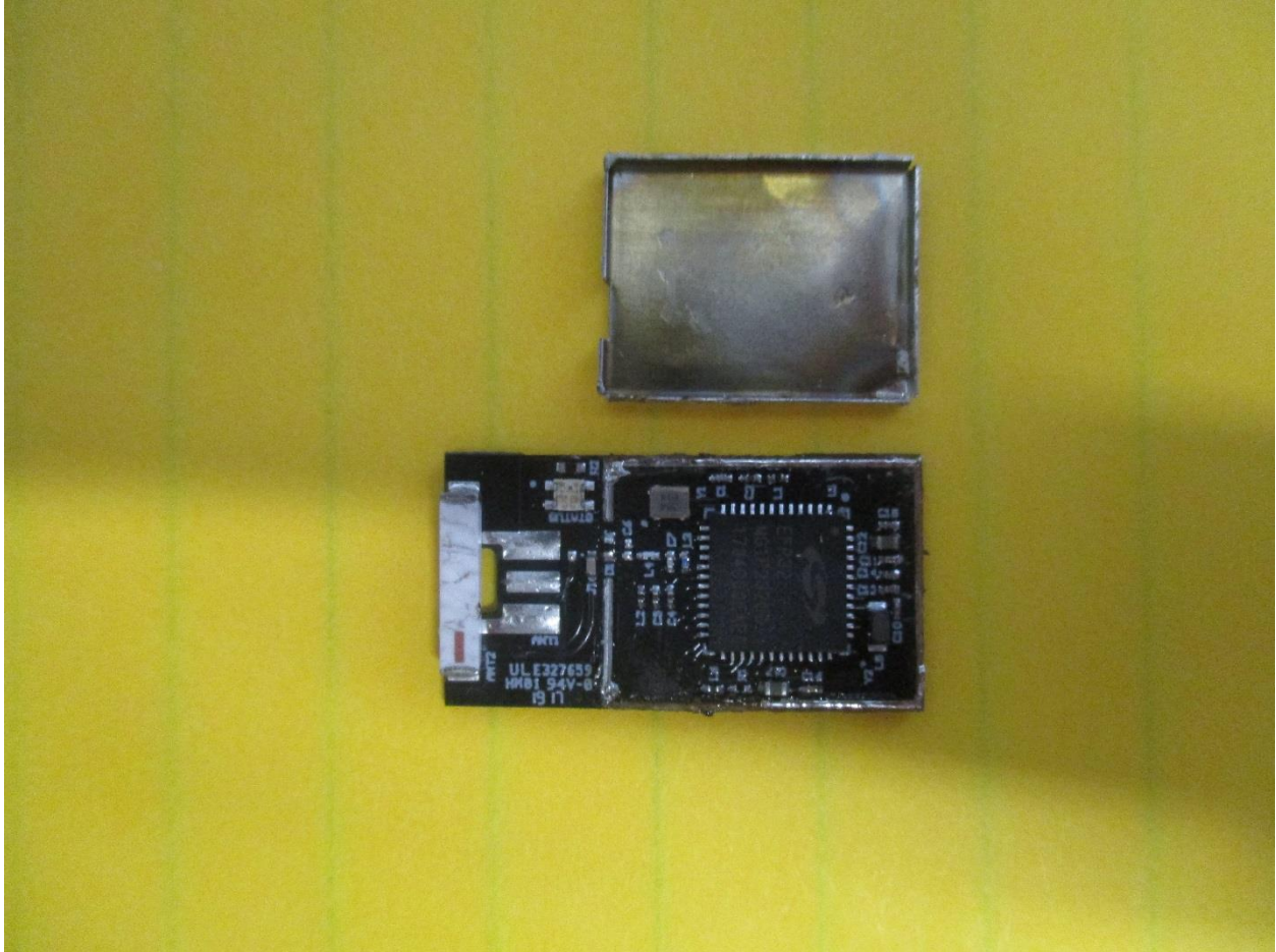
Module PCB Top with Shield Removed
