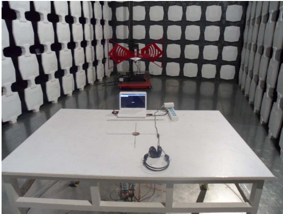
Setup for Radiated Emission test below 1GHz
