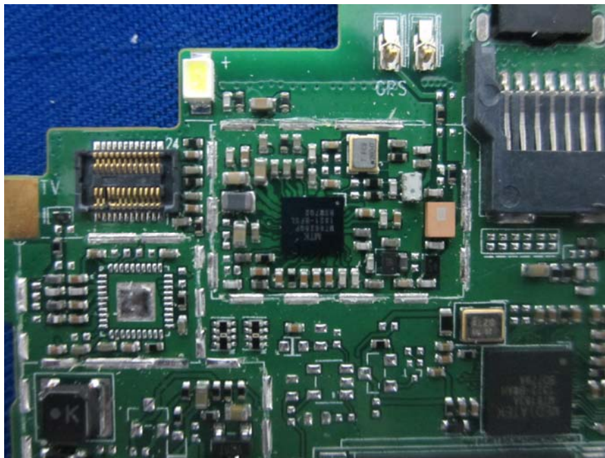
EUT- BT and Wifi Module View
