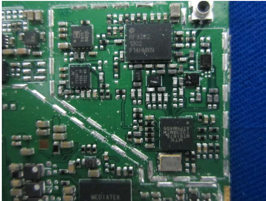
EUT- GSM and WCDMA Module View
