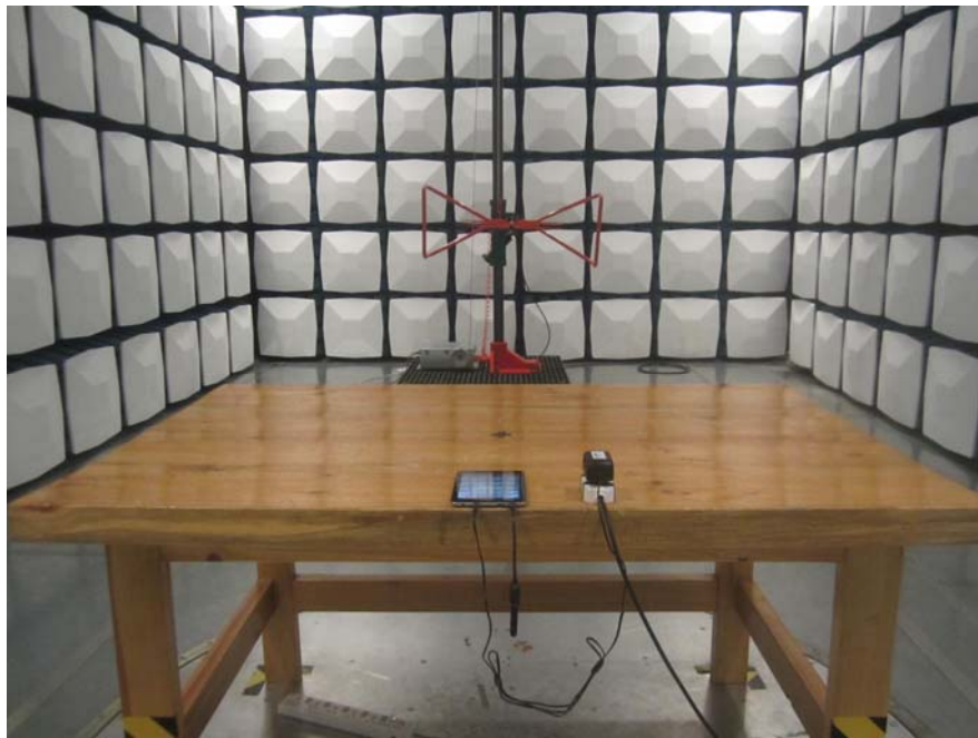
Radiated Emission - Rear View (Video Play) (Below 1GHz)
