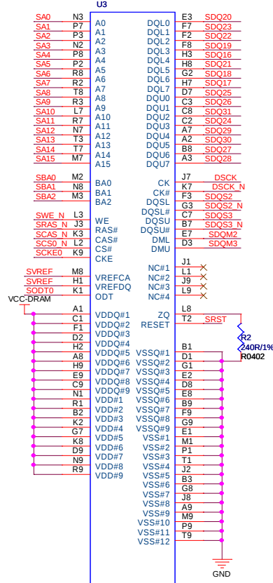
H5TQ4G63MFR-H9C-FBGA96 FBGA96C80P10X14
