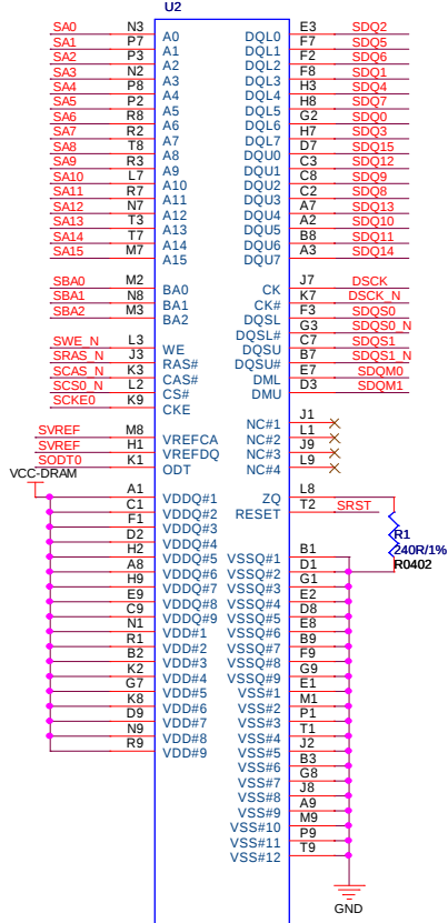
H5TQ4G63MFR-H9C-FBGA96 FBGA96C80P10X14
