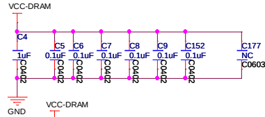
H5TQ4G63MFR-H9C-FBGA96 FBGA96C80P10X14
