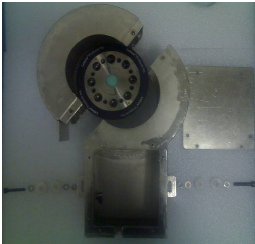
Figure 2: Shroud internal
