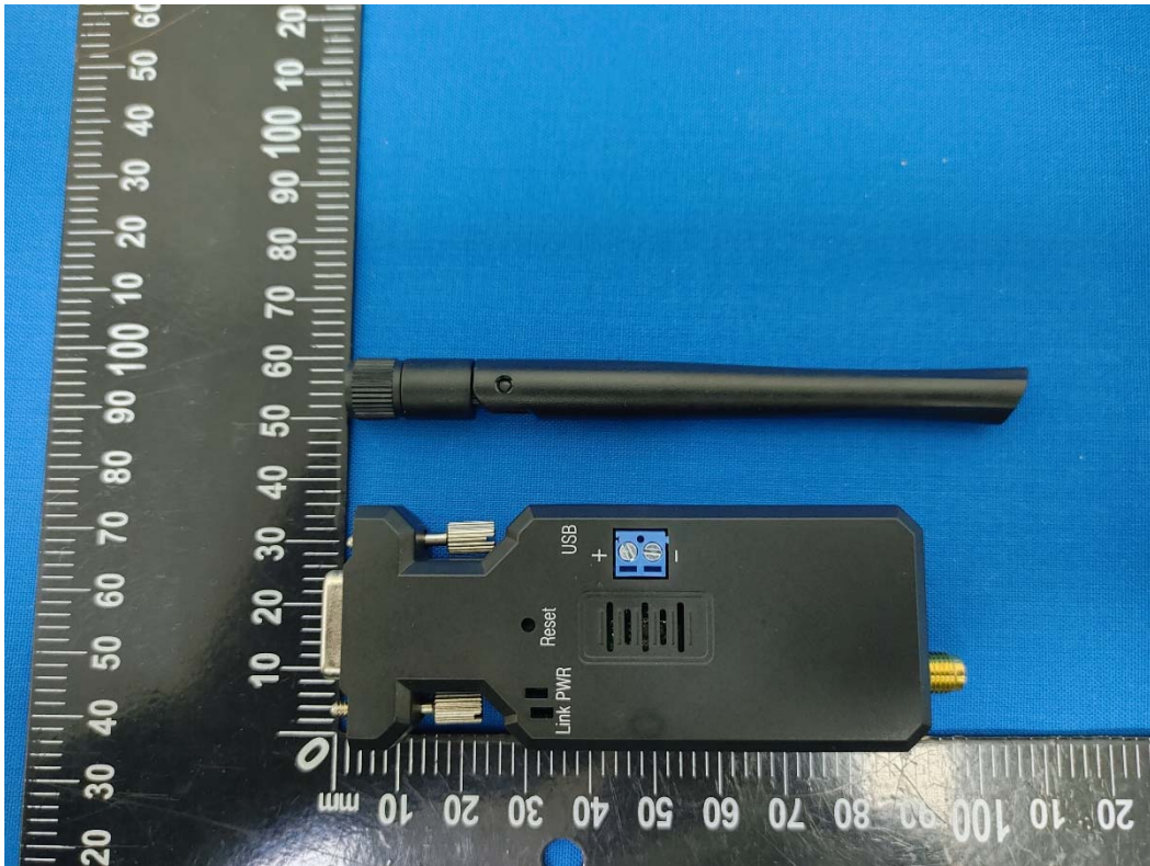
Dipole Antenna
