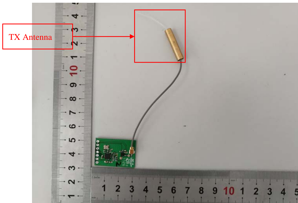
EUT – PCB-2 Module Top View
