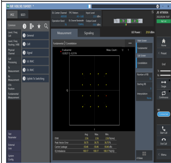
1-N70-PC3-15-15-M-3-DFT-16QAM-Outer_Full-75@0-Ant1-see graph-PASS
