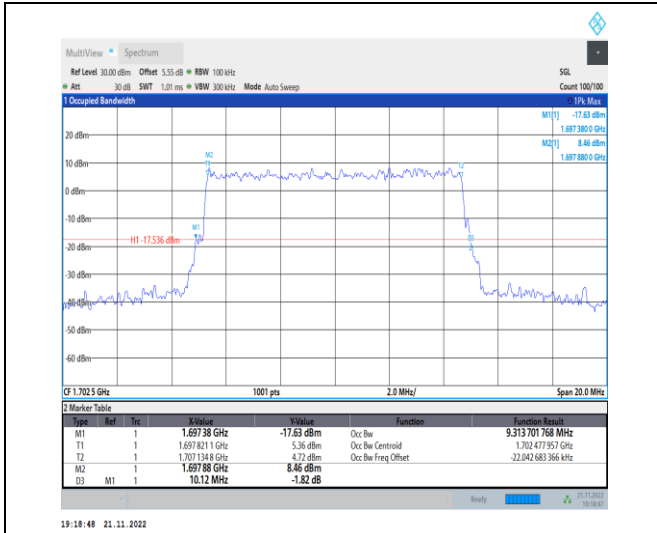
1-N70-PC3-15-10-M-9-CP-256QAM-Outer_Full-52@ 0-Ant1-9.314-10.120-≤10-PASS
