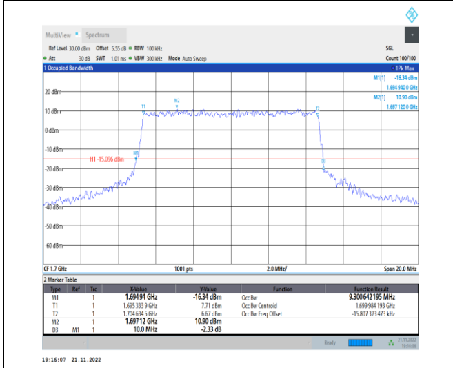
1-N70-PC3-15-10-L-8-CP-64QAM-Outer_Full-52@0-0 Ant1-9.301-10.000-≤10-PASS
