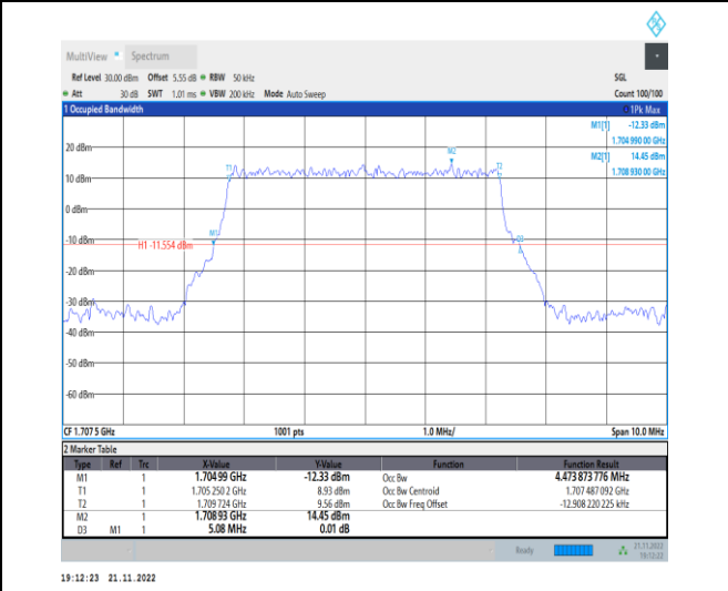
1-N70-PC3-15-5-H-2-DFT-PI2BPSK-Outer_Full-25@0-Ant1-4.474-5.080-≤5-PASS
