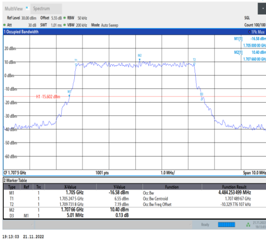
1-N70-PC3-15-5-H-5-DFT-256QAM-Outer_Full-25@0-Ant1-4.484-5.010-≤5-PASS
