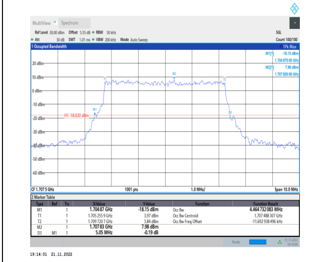
1-N70-PC3-15-5-H-9-CP-256QAM-Outer_Full-25@0-Ant1-4.465-5.050-≤5-PASS
