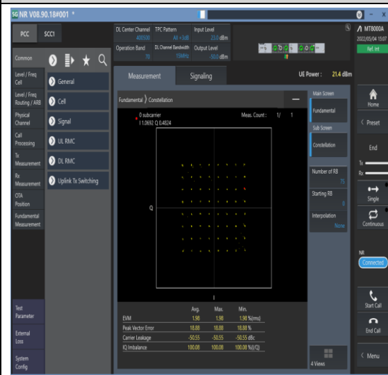
1-N70-PC3-15-15-M-4-DFT-64QAM-Outer_Full-75@0-Ant1-see graph-PASS
