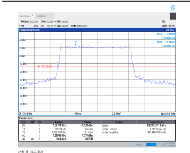
1-N70-PC3-15-10-M-3-DFT-16QAM-Outer_Full-50@0 0-Ant1-8.929-9.640-≤10-PASS
