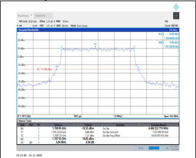
1-N70-PC3-15-5-H-8-CP-64QAM-Outer_Full-25@0-Ant1-4.469-5.040-≤5-PASS
