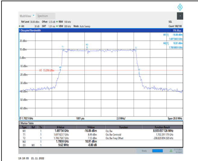
1-N70-PC3-15-10-M-5-DFT-256QAM-Outer_Full-50 @ 0-Ant1-8.935-9.620-≤10-PASS
