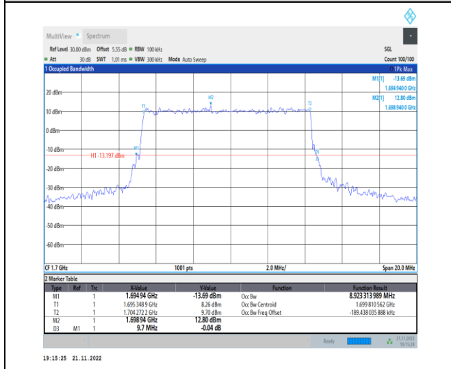
1-N70-PC3-15-10-L-4-DFT-64QAM-Outer_Full-50 @ 0-Ant1-8.923-9.700-≤10-PASS
