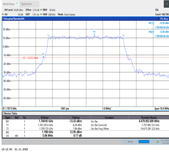
1-N70-PC3-15-5-H-3-DFT-16QAM-Outer_Full-25@0-Ant1-4.479-5.060-≤5-PASS
