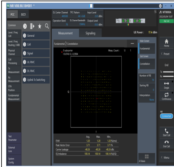
1-N70-PC3-15-15-M-9-CP-256QAM-Outer_F ull-79@0-Ant1-see graph-PASS
