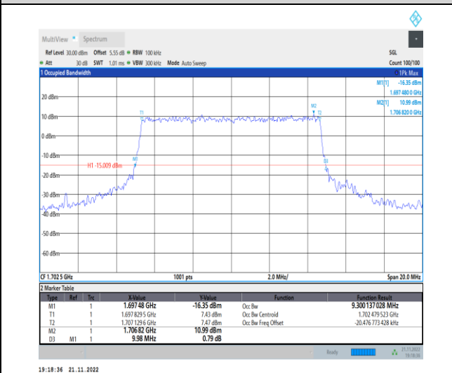
1-N70-PC3-15-10-M-4-DFT-64QAM-Outer_Full-50@0 0-Ant1-8.188-8.400-≤10-PASS
