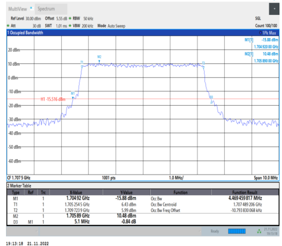
1-N70-PC3-15-5-H-6-CP-QPSK-Outer_Full-25@0-Ant1-4.469-5.100-≤5-PASS
