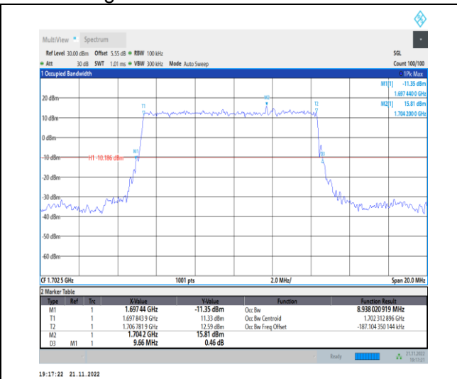
1-N70-PC3-15-10-M-2-DFT-PI2BPSK-Outer_Full-50@0 @0-Ant1-8.938-9.660-≤10-PASS
