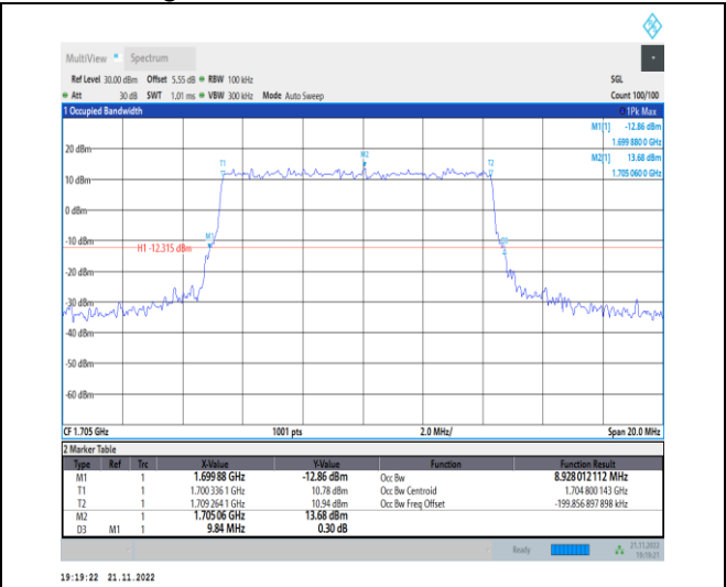
1-N70-PC3-15-10-H-1-DFT-QPSK-Outer_Full-50@0 -Ant1-8.928-9.840-≤10-PASS
