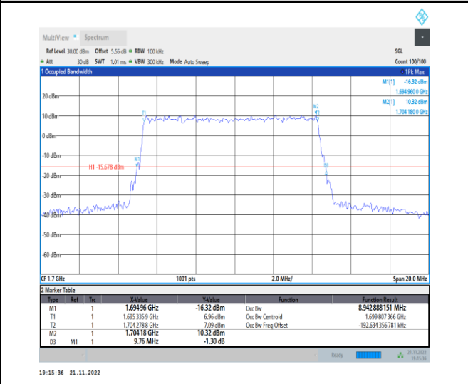
1-N70-PC3-15-10-L-5-DFT-256QAM-Outer_Full-50 @ 0-Ant1-8.943-9.760-≤10-PASS
