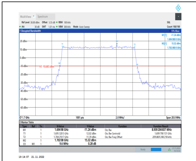
1-N70-PC3-15-10-L-2-DFT-PI2BPSK-Outer_Full-50 @ 0-Ant1-8.939-9.600-≤10-PASS
