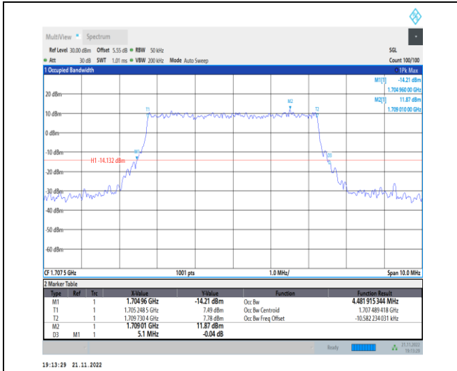
1-N70-PC3-15-5-H-7-CP-16QAM-Outer_Full-25@0-Ant1-4.482-5.100-≤5-PASS
