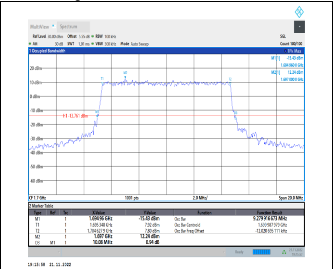
1-N70-PC3-15-10-L-7-CP-16QAM-Outer_Full-52@0-0 Ant1-9.28-10.080-≤10-PASS
