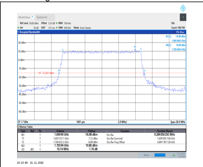
1-N70-PC3-15-10-L-3-DFT-16QAM-Outer_Full-50 @ 0-Ant1-8.939-9.520-≤10-PASS
