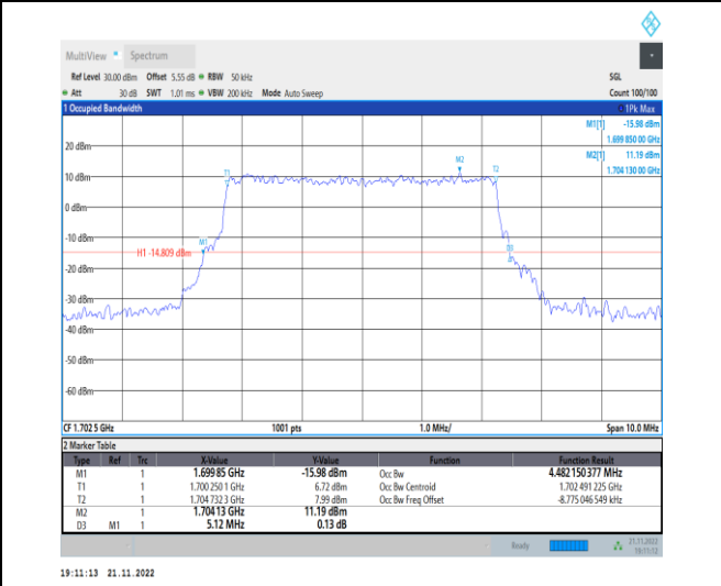
1-N70-PC3-15-5-M-7-CP-16QAM-Outer_Full-25@0-Ant1-4.482-5.120-≤5-PASS
