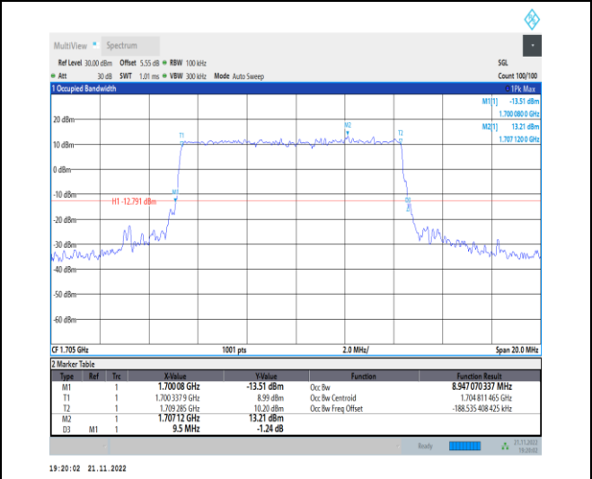
1-N70-PC3-15-10-H-3-DFT-16QAM-Outer_Full-50@ 0-Ant1-8.947-9.500-≤10-PASS
