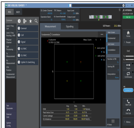
1-N70-PC3-15-15-M-1-DFT-PI2BPSK-Outer_Full-75@0-Ant1-see graph-PASS
