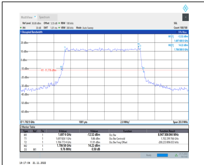
1-N70-PC3-15-10-M-1-DFT-QPSK-Outer_Full-50@0 -Ant1-8.947-9.760-≤10-PASS
