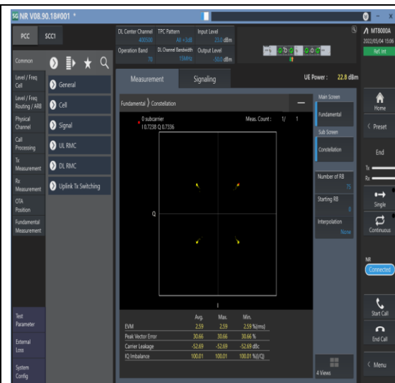
1-N70-PC3-15-15-M-2-DFT-QPSK-Outer_Full-75@0-Ant1-see graph-PASS
