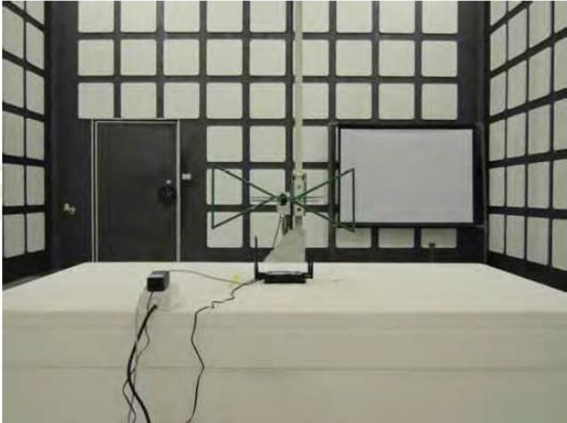
Radiated Emission Set up Photos (Below 1GHz)
