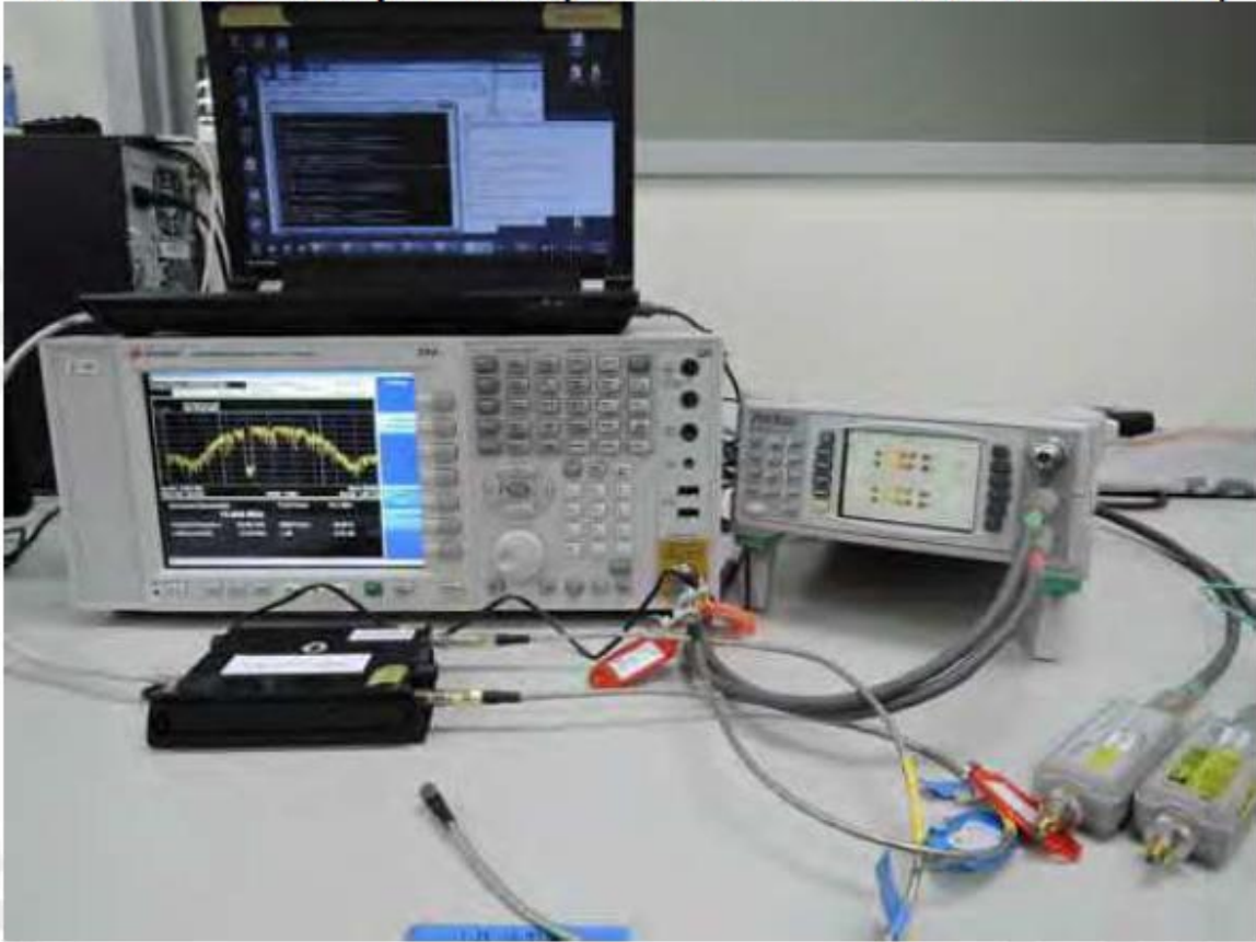
Conducted Setup Photo (Measurement at Antenna Port)
