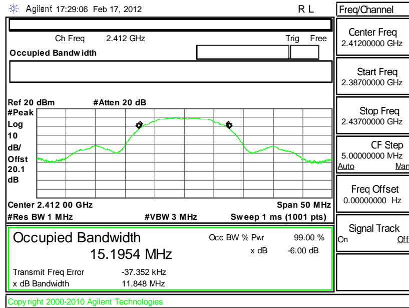
Mode 1 : 99% Occupied Bandwidth Plot on 802.11b Channel 01
