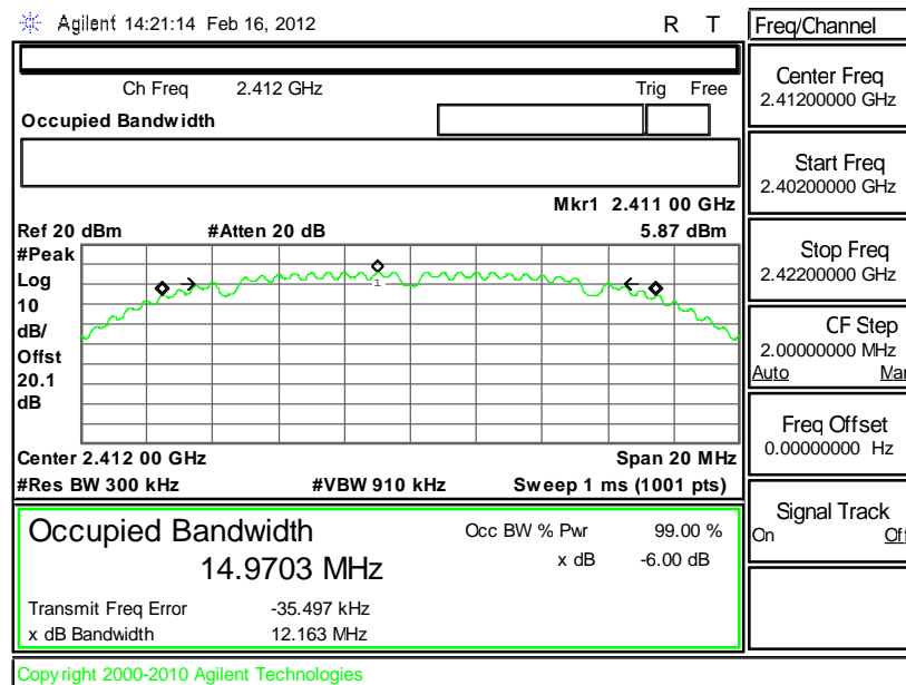
Mode 1 : 6 dB Bandwidth Plot on 802.11b Channel 01 – Chain A
