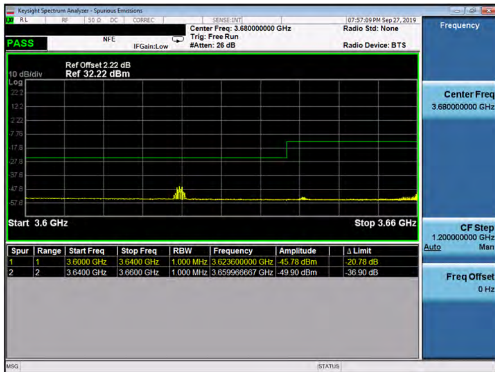
Plot 7-190. Conducted Spurious Plot (Band 48 – 20.0MHz QPSK – Left Carrier 1/0 Right Carrier 1/0 – High Channel)
