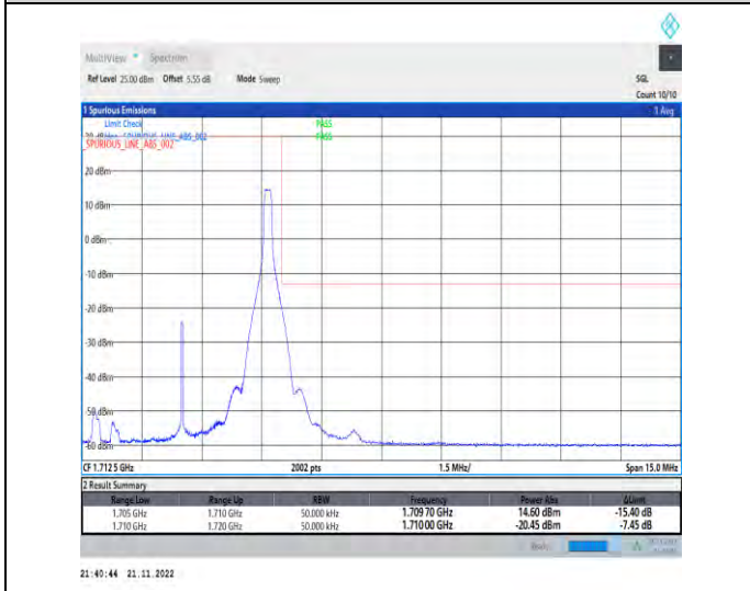
1-N70-PC3-15-5-H-5-CP-QPSK-Edge_1RB_Right-1@24-Ant1-1-seegraph-PASS-see graph
