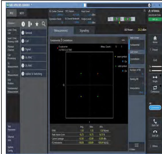
1-N70-PC3-15-15-M-1-DFT-PI2BPSK-Outer_Full-75@0-Ant1-see graph-PASS
