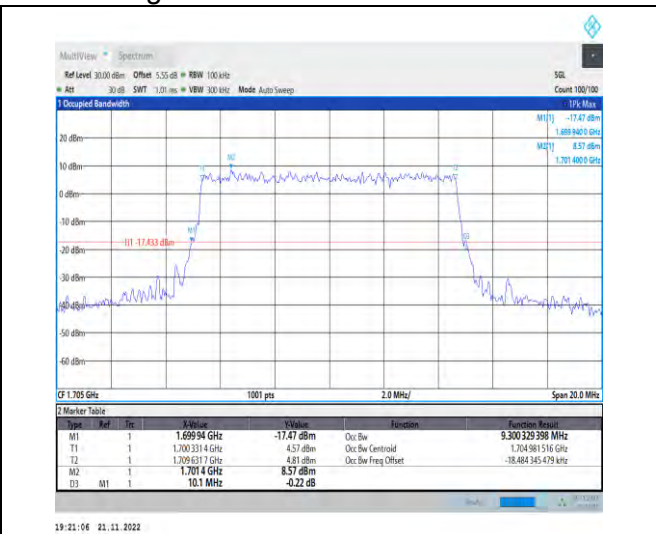
1-N70-PC3-15-10-H-9-CP-256QAM-Outer_Full-52@ 0-Ant1-9.3-10.100-≤10-PASS
