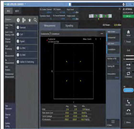
1-N70-PC3-15-15-M-2-DFT-QPSK-Outer_Full-75@0-Ant1-see graph-PASS
