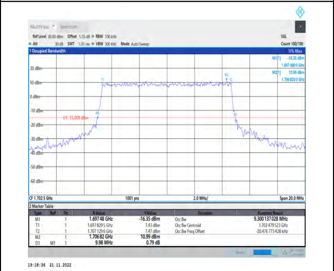
1-N70-PC3-15-10-M-8-CP-64QAM-Outer_Full-52@0-Ant1-9.3-9.980-≤10-PASS
