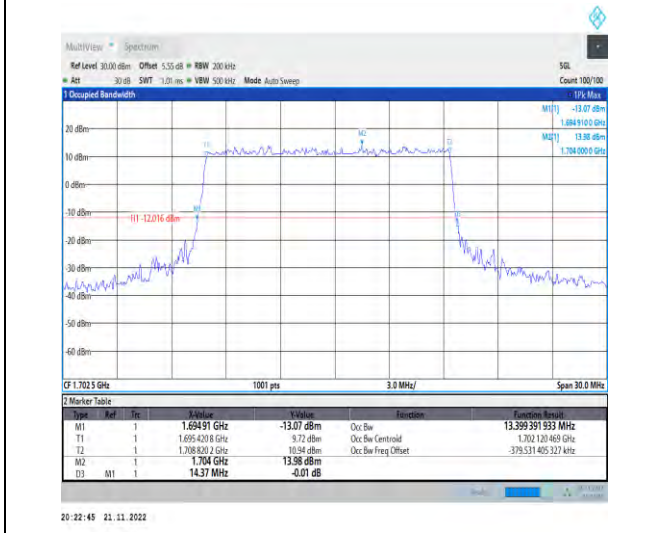
1-N70-PC3-15-15-M-4-DFT-64QAM-Outer_Full-75 @0-Ant1-13.399-14.370-≤15-PASS
