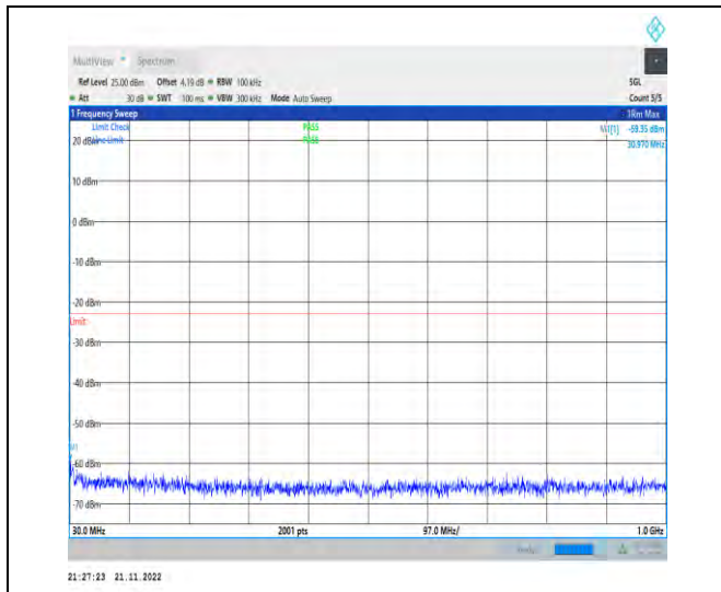
1-N70-PC3-15-15-H-1-DFT-PI2BPSK-Inner_1RB_Le ft-1@1-30-1000-Ant1-30.97--59.35--23-PASS
