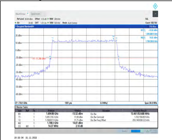
1-N70-PC3-15-15-M-3-DFT-16QAM-Outer_Full-75 @0-Ant1-13.461-14.370-≤15-PASS
