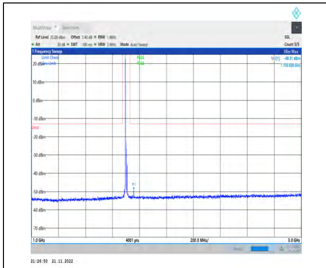
1-N70-PC3-15-15-M-1-DFT-PI2BPSK-Inner_1RB_Le ft-1@1-1000-3000-Ant1-1756.50--49.31--13-PASS
