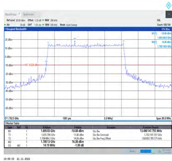
1-N70-PC3-15-15-M-1-DFT-QPSK-Outer_Full-75@0-Ant1-13.49-14.190-≤15-PASS
