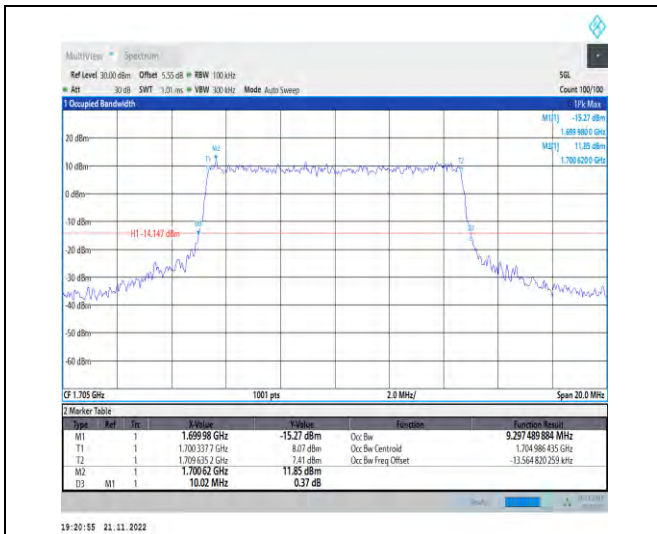
1-N70-PC3-15-10-H-8-CP-64QAM-Outer_Full-52@0 -Ant1-9.297-10.020-≤10-PASS
