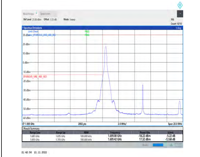
1-N70-PC3-15-10-L-4-CP-QPSK-Edge_1RB_Left-1@0-Ant1-1-seegraph-PASS-see graph
