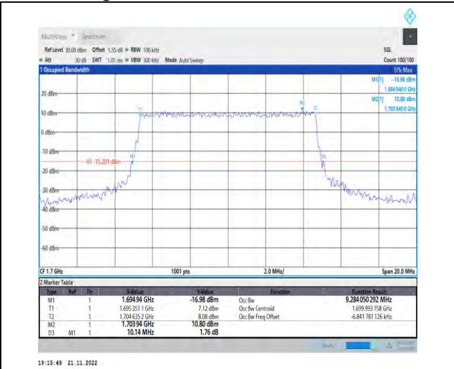
1-N70-PC3-15-10-L-3-DFT-16QAM-Outer_Full-50 @0-Ant1-8.939-9.520-≤10-PASS
