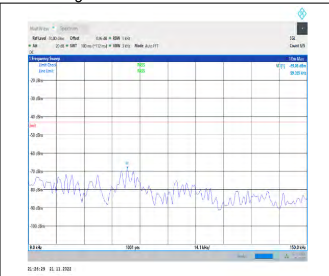
1-N70-PC3-15-15-M-1-DFT-PI2BPSK-Inner_1RB_Le ft-1@1-0.009-0.15-Ant1-0.06--69.06--43-PASS
