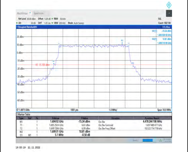
1-N70-PC3-15-5-L-8-CP-64QAM-Outer_Full-25@0-Ant1-4.478-5.100-≤5-PASS
