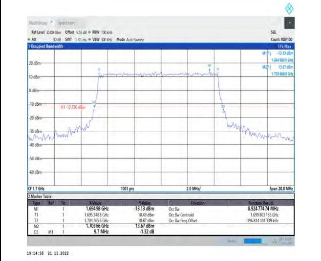
1-N70-PC3-15-10-L-1-DFT-QPSK-Outer_Full-50@0-Ant1-8.925-9.700-≤10-PASS
