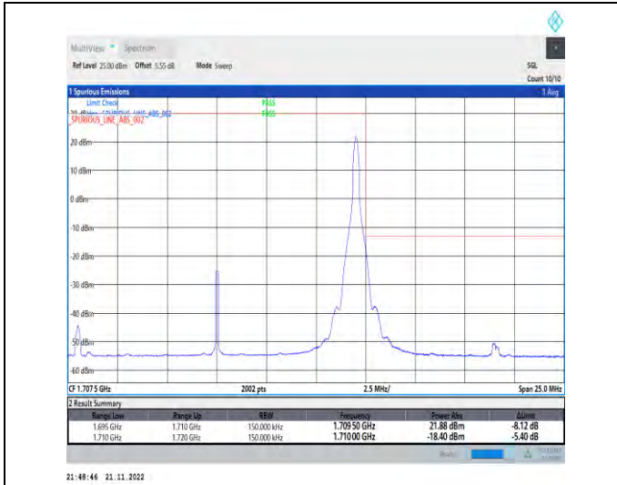
1-N70-PC3-15-15-H-2-DFT-PI2BPSK-Edge_1RB_Right-t1@78-Ant1-1-seegraph-PASS-see graph
