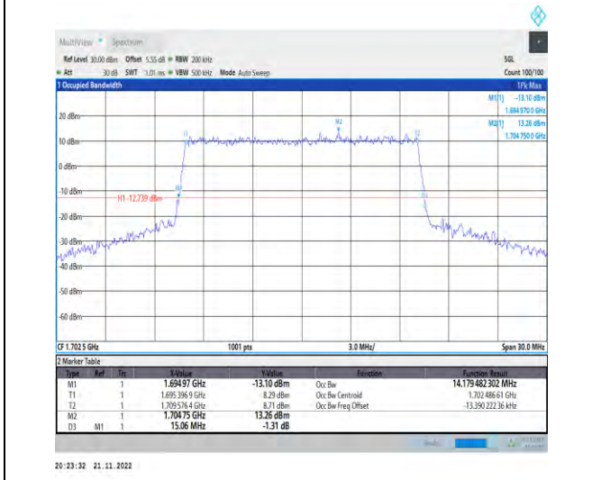
1-N70-PC3-15-15-M-8-CP-64QAM-Outer_Full-79@0-Ant1-14.179-15.060-≤15-PASS
