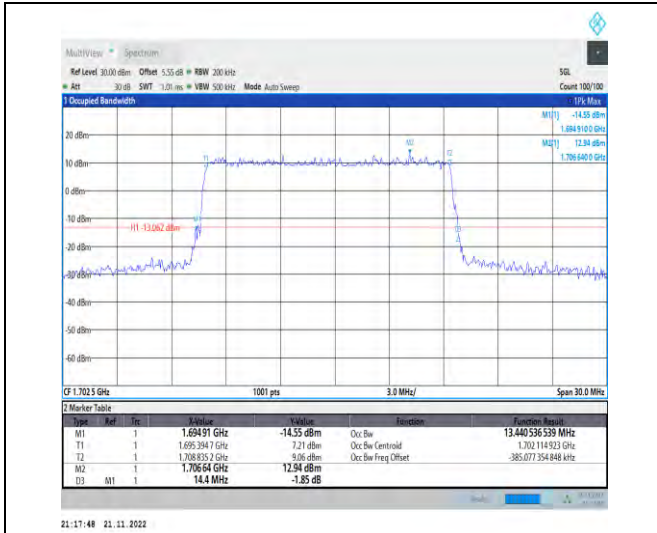
1-N70-PC3-15-15-H-5-DFT-256QAM-Outer_Full-75 @0-Ant1-13.441-14.400-≤15-PASS
