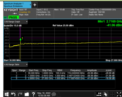
Channel 41540 (2685MHz)
