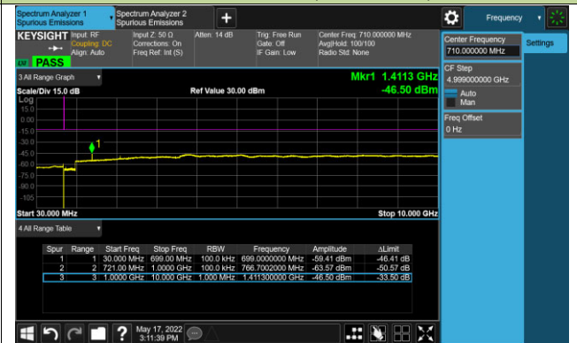
Channel 23790(710.0MHz)
