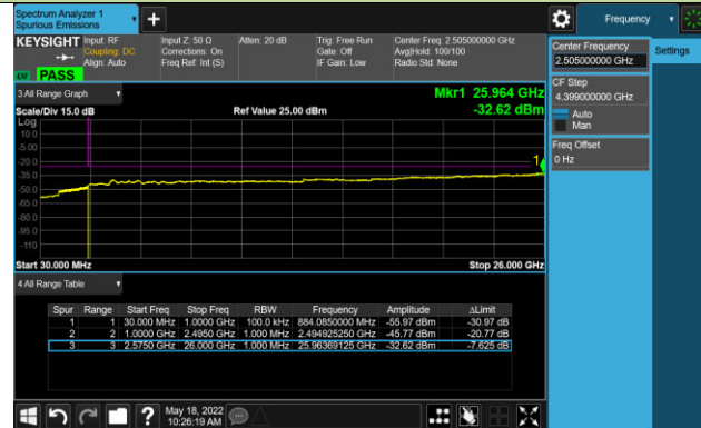
Channel 21400 (2565MHz)
