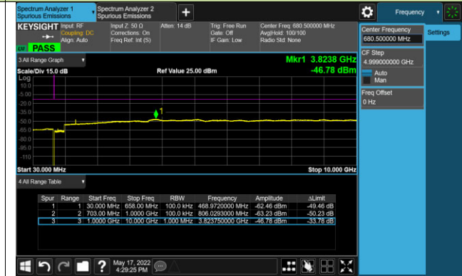
Channel 133297 (680.5MHz)
