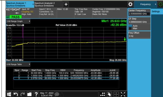
Channel 21100 (2535MHz)
