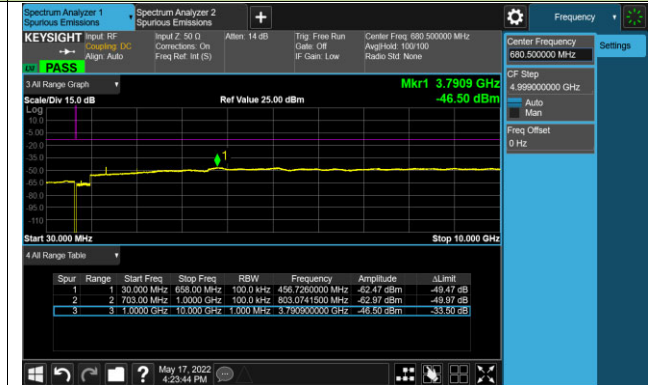
Channel 133297 (680.5MHz)
