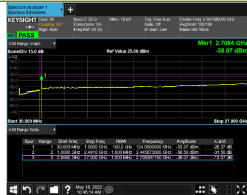
Channel 40565 (2687.5MHz)
