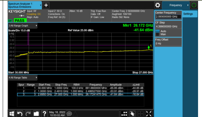
Channel 40620 (2593MHz)
