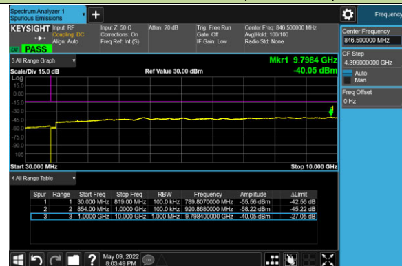
Channel 27015 (846.5MHz)
