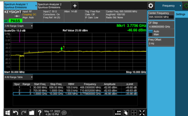
Channel 133447 (695.5MHz)
