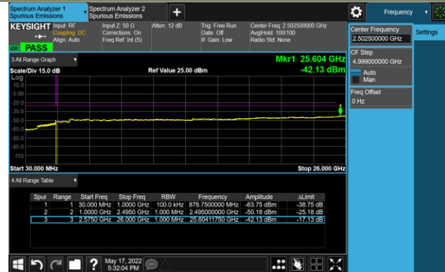
Channel 21425 (2567.5MHz)
