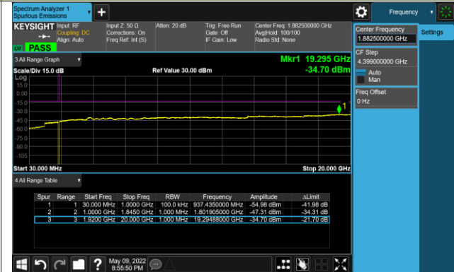
Channel 26365 (1882.5MHz)
