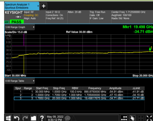
Channel 132647 (1777.5MHz)
