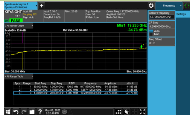
Channel 132597 (1772.5Hz)
