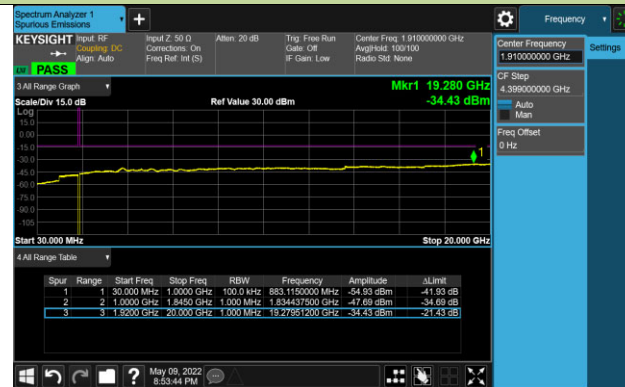
Channel 26640 (1910MHz)
