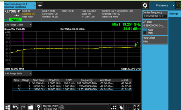
Channel 26590 (1905MHz)
