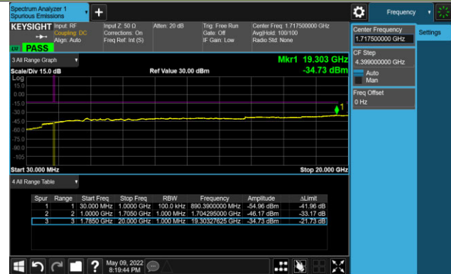
Channel 132597 (1772.5Hz)
