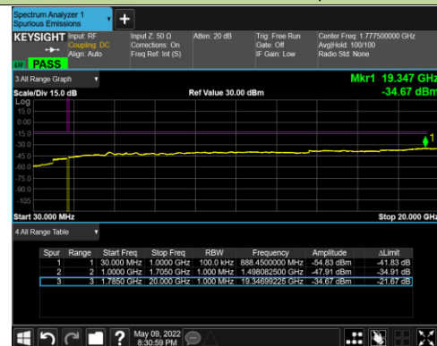
Channel 132647 (1777.5MHz)
