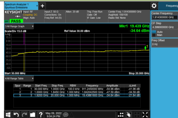
Channel 26683 (1914.3MHz)
