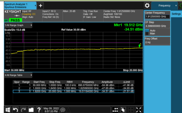
Channel 26665 (1912.5MHz)
