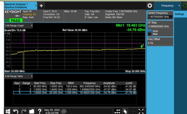
Channel 26615 (1907.5MHz)
