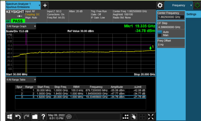
Channel 26365 (1882.5MHz)
