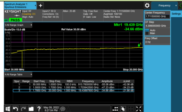
Channel 132657 (1778.5MHz)
