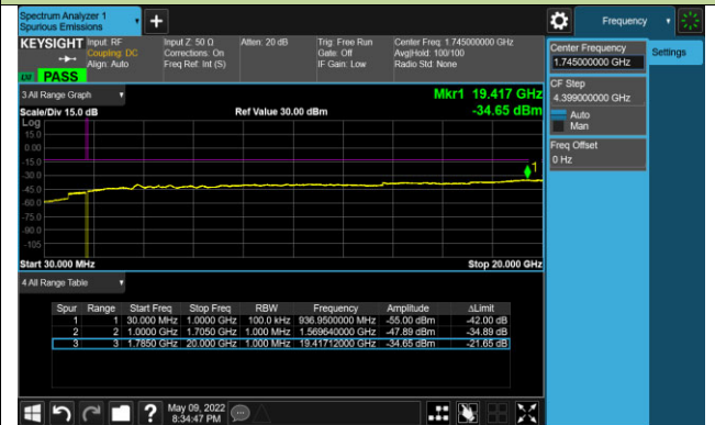
Channel 132322 (1745MHz)
