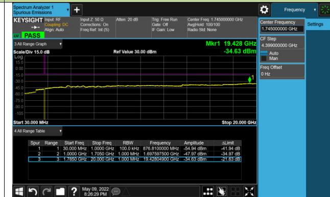
Channel 132322 (1745MHz)
