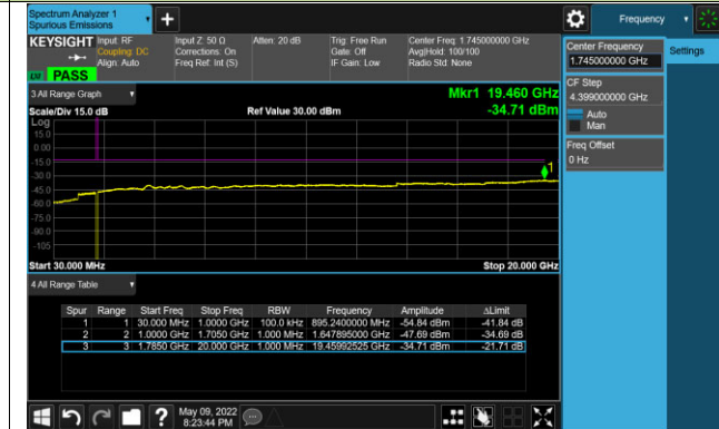
Channel 132322 (1745MHz)
