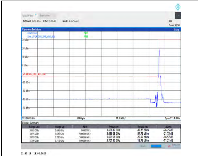
1-N78-3700-3800-PC1-30-90-L-1-DFT-PI2BPSK-Edge_1RB_Left-1@0-Ant1-1--PASS-see graph
