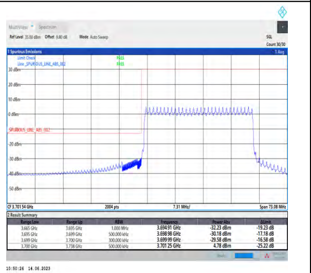
1-N78-3700-3800-PC1-30-30-L-6-CP-QPSK-Outer_Full-78@0-Ant1-1--PASS-see graph
