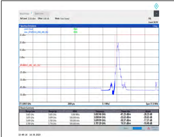
1-N78-3700-3800-PC1-30-30-L-1-DFT-PI2BPSK-Edge_1RB_Left-1@0-Ant1-1--PASS-see graph
