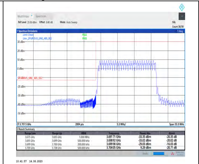
1-N78-3700-3800-PC1-30-20-L-3-DFT-PI2BPSK-Outer_Full-50@0-Ant1-1--PASS-see graph
