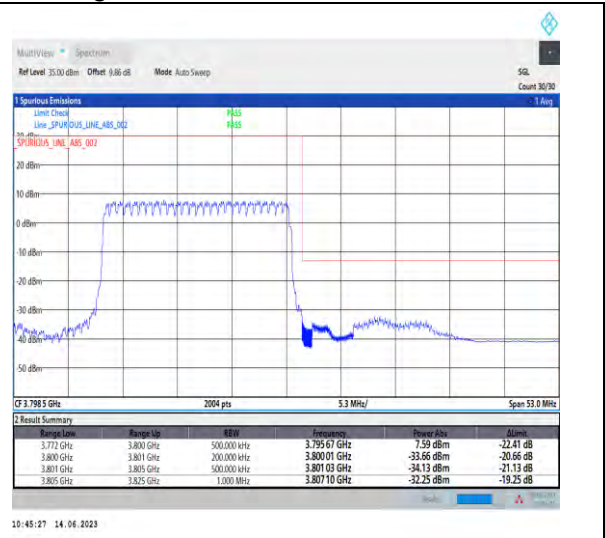
1-N78-3700-3800-PC1-30-20-H-3-DFT-PI2BPSK-Outer_Full-50@0-Ant1-1--PASS-see graph
