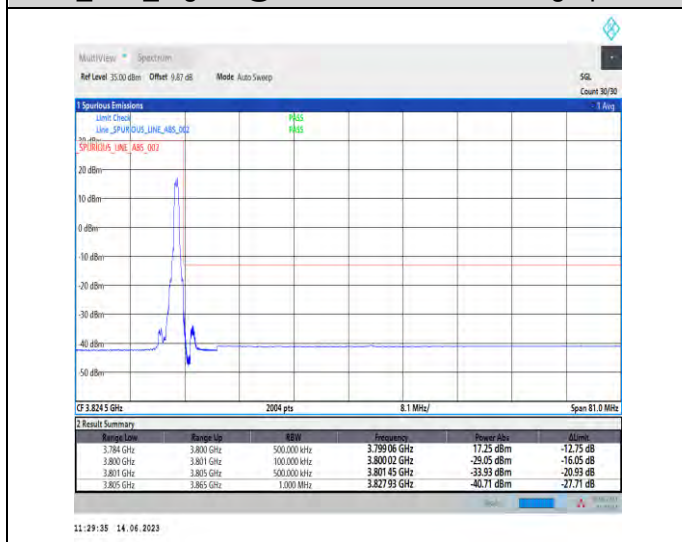
1-N78-3700-3800-PC1-30-60-H-5-CP-QPSK-Edge_1RB_Right-1@161-Ant1-1--PASS-see graph
