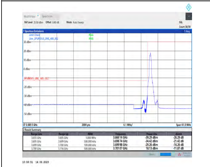
1-N78-3700-3800-PC1-30-40-L-4-CP-QPSK-Edge_1RB_Left-1@0-Ant1-1--PASS-see graph
