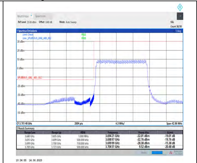
1-N78-3700-3800-PC1-30-15-L-3-DFT-PI2BPSK-Outer_Full-36@0-Ant1-1--PASS-see graph
