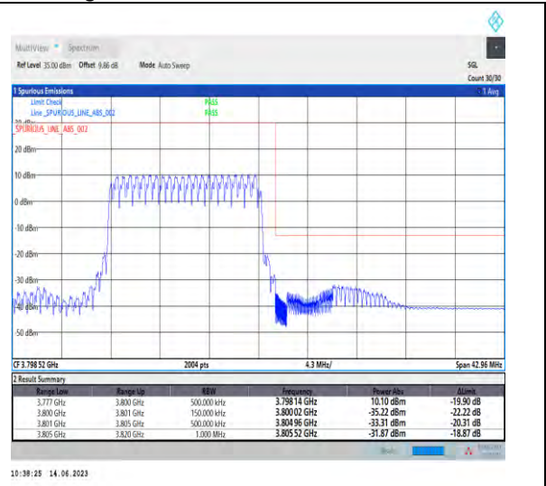
1-N78-3700-3800-PC1-30-15-H-3-DFT-PI2BPSK-Outer_Full-36@0-Ant1-1--PASS-see graph
