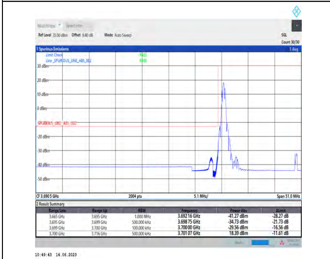
1-N78-3700-3800-PC1-30-30-L-4-CP-QPSK-Edge_1RB_Left-1@0-Ant1-1--PASS-see graph
