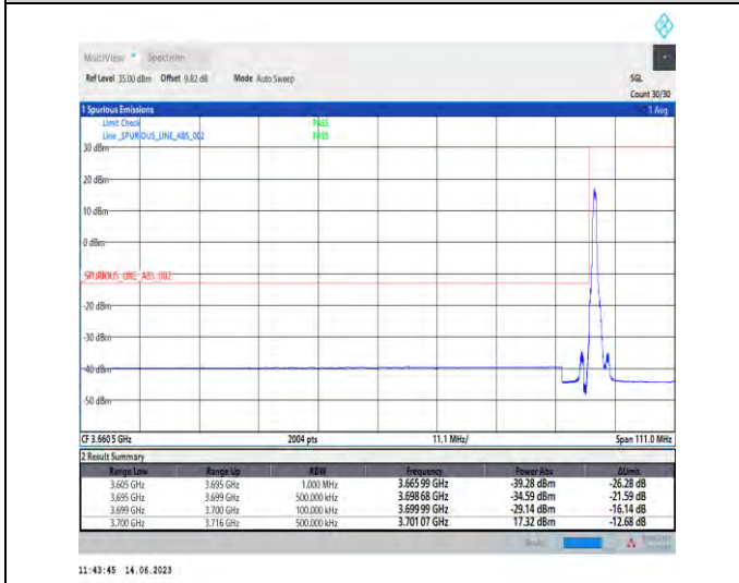
1-N78-3700-3800-PC1-30-90-L-4-CP-QPSK-Edge_1RB_Left-1@0-Ant1-1--PASS-see graph
