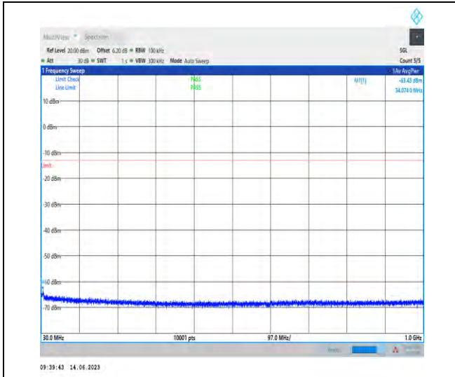
1-N78-3700-3800-PC1-30-100-M-1-N/A-DFT-QPSK-Edge_1RB_Left-1@0-30-1000-Ant1-34.07--63.43--1 3-PASS
