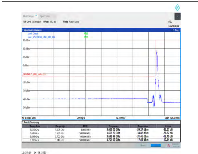
1-N78-3700-3800-PC1-30-80-L-1-DFT-PI2BPSK-Edge_1RB_Left-1@0-Ant1-1--PASS-see graph
