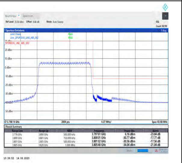
1-N78-3700-3800-PC1-30-15-H-6-CP-QPSK-Outer_Full-38@0-Ant1-1--PASS-see graph
