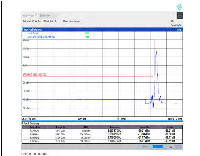
1-N78-3700-3800-PC1-30-70-L-1-DFT-PI2BPSK-Edge_1RB_Left-1@0-Ant1-1--PASS-see graph
