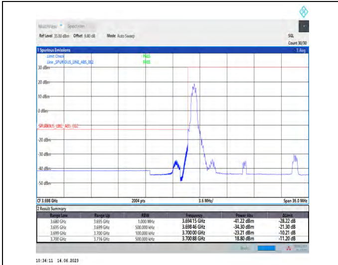
1-N78-3700-3800-PC1-30-15-L-1-DFT-PI2BPSK-Edge_1RB_Left-1@0-Ant1-1--PASS-see graph
