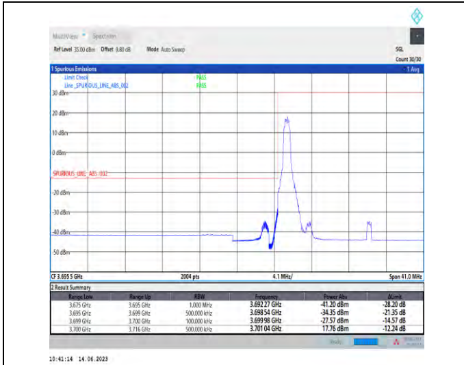
1-N78-3700-3800-PC1-30-20-L-1-DFT-PI2BPSK-Edge_1RB_Left-1@0-Ant1-1--PASS-see graph
