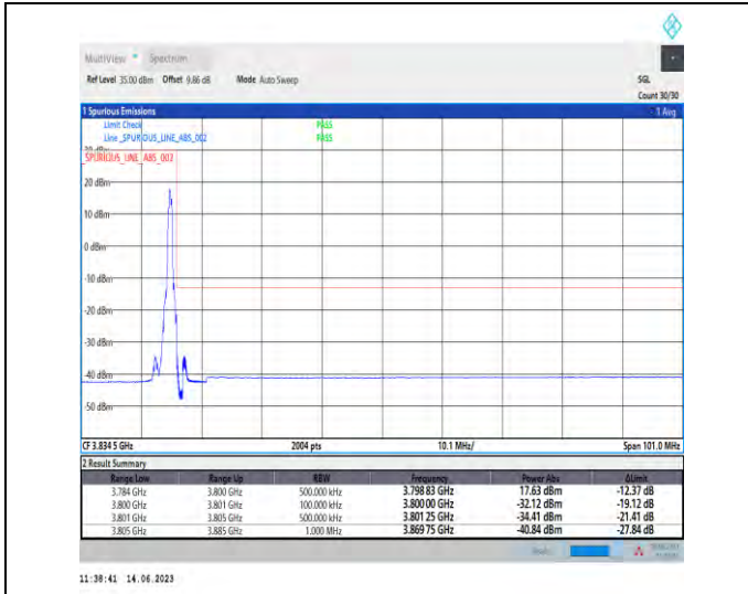
1-N78-3700-3800-PC1-30-80-H-2-DFT-PI2BPSK-Edge_1RB_Right-1@216-Ant1-1--PASS-see graph
