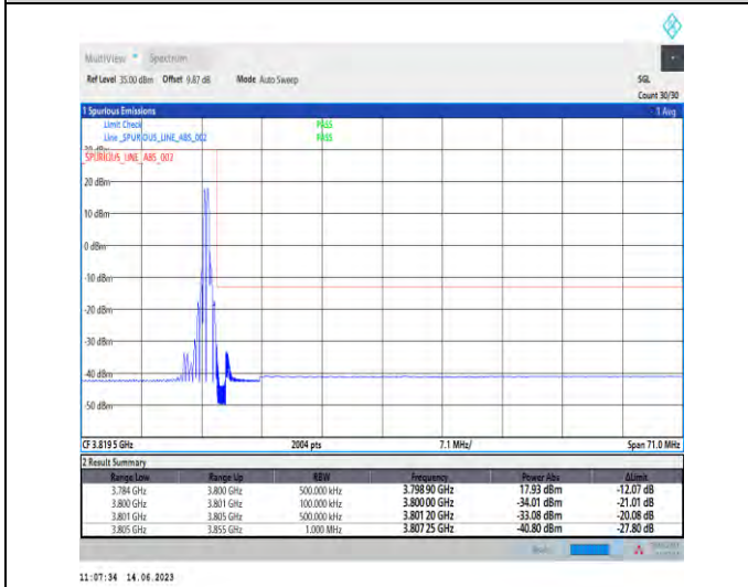
1-N78-3700-3800-PC1-30-50-H-5-CP-QPSK-Edge_1RB_Right-1@132-Ant1-1--PASS-see graph
