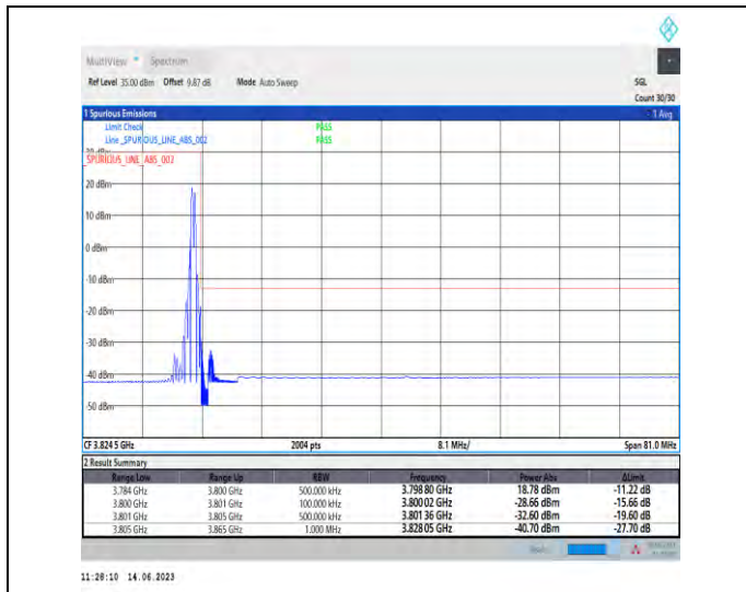
1-N78-3700-3800-PC1-30-60-H-2-DFT-PI2BPSK-Edge_1RB_Right-1@161-Ant1-1--PASS-see graph
