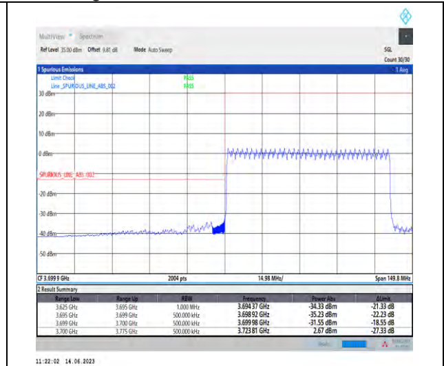
1-N78-3700-3800-PC1-30-70-L-3-DFT-PI2BPSK-Outer_Full-180@0-Ant1-1--PASS-see graph
