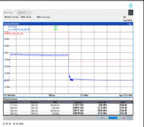
1-N78-3700-3800-PC1-30-80-H-6-CP-QPSK-Outer_Full-217@0-Ant1-1--PASS-see graph
