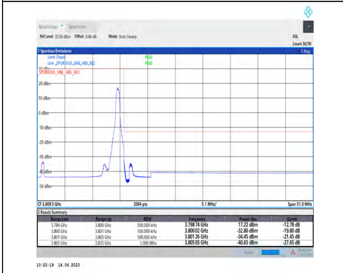
1-N78-3700-3800-PC1-30-30-H-5-CP-QPSK-Edge_1RB_Right-1@77-Ant1-1--PASS-see graph
