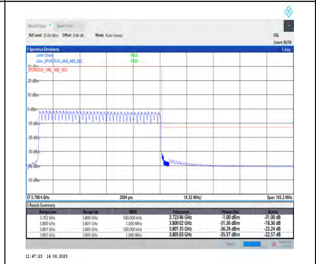
1-N78-3700-3800-PC1-30-90-H-6-CP-QPSK-Outer_Full-245@0-Ant1-1--PASS-see graph
