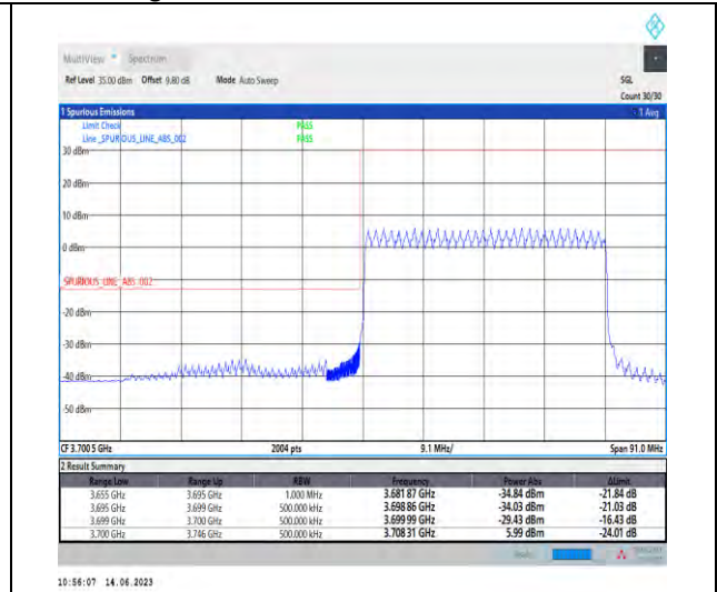
1-N78-3700-3800-PC1-30-40-L-3-DFT-PI2BPSK-Outer_Full-100@0-Ant1-1--PASS-see graph
