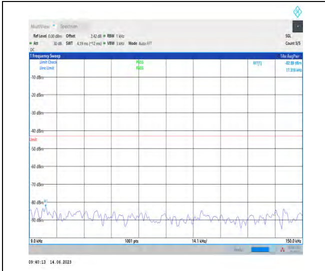
1-N78-3700-3800-PC1-30-100-H-1-N/A-DFT-QPSK-Edge_1RB_Left-1@0-0.009-0.15-Ant1-0.02--82.89--43-PASS
