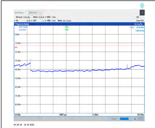
1-N78-3700-3800-PC1-30-100-L-1-N/A-DFT-QPSK-Edge_1RB_Left-1@0-6000-18000-Ant1-7495.20--32.65--13-PASS
