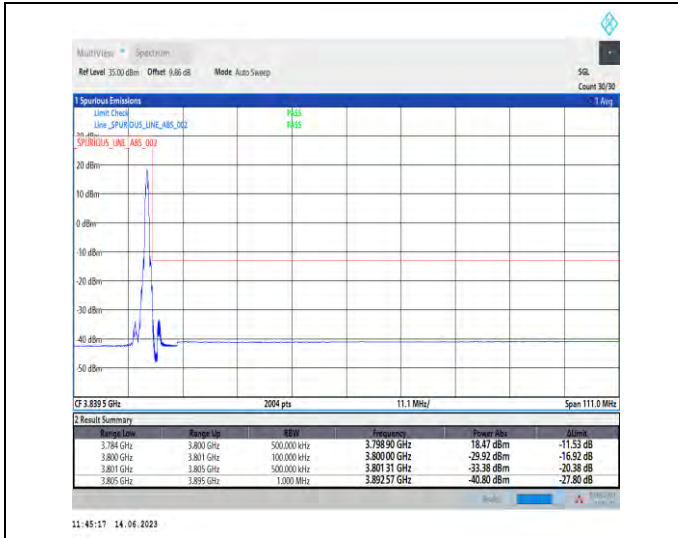
1-N78-3700-3800-PC1-30-90-H-2-DFT-PI2BPSK-Edge_1RB_Right-1@244-Ant1-1--PASS-see graph
