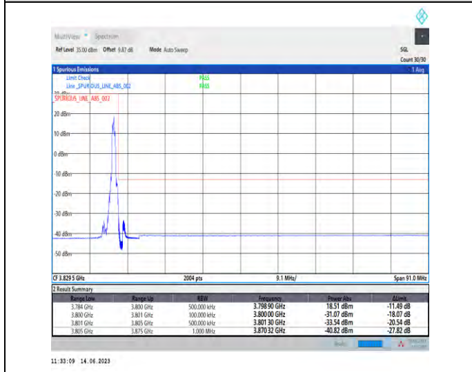
1-N78-3700-3800-PC1-30-70-H-5-CP-QPSK-Edge_1RB_Right-1@188-Ant1-1--PASS-see graph
