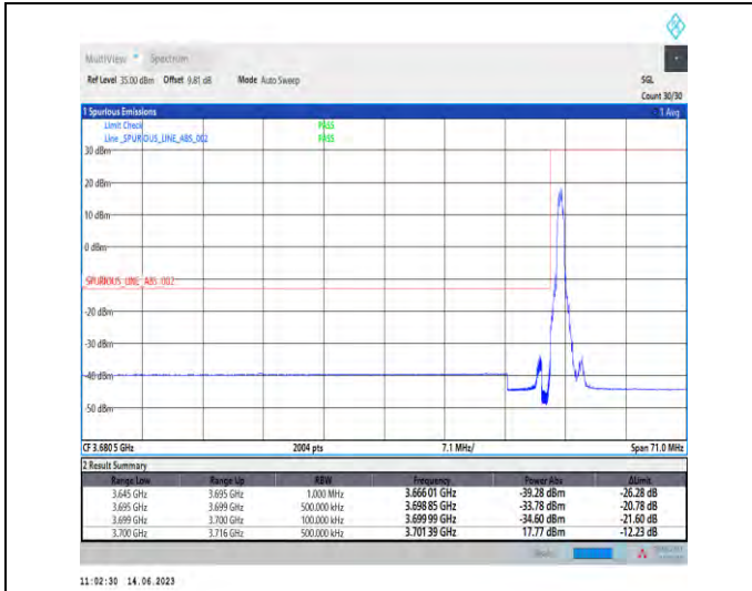
1-N78-3700-3800-PC1-30-50-L-1-DFT-PI2BPSK-Edge_1RB_Left-1@0-Ant1-1--PASS-see graph
