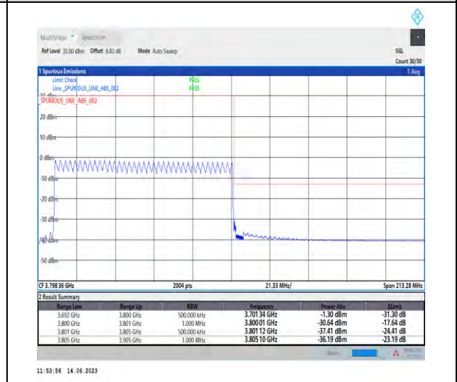
1-N78-3700-3800-PC1-30-100-H-6-CP-QPSK-Outer_Full-273@0-Ant1-1--PASS-see graph
