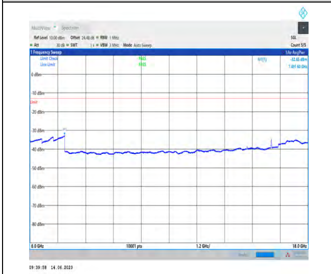
1-N78-3700-3800-PC1-30-100-M-1-N/A-DFT-QPSK-Edge_1RB_Left-1@0-6000-18000-Ant1-7491.60--32.65--13-PASS
