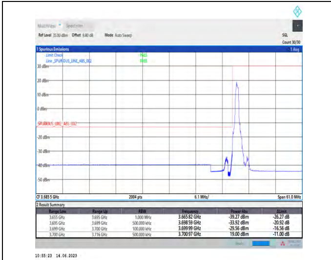
1-N78-3700-3800-PC1-30-40-L-1-DFT-PI2BPSK-Edge_1RB_Left-1@0-Ant1-1--PASS-see graph
