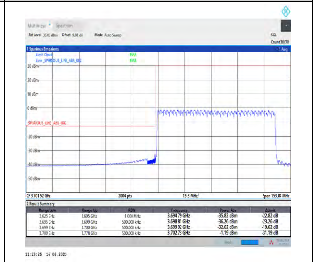
1-N78-3700-3800-PC1-30-70-L-6-CP-QPSK-Outer_Full-189@0-Ant1-1--PASS-see graph
