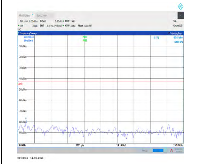
1-N78-3700-3800-PC1-30-100-M-1-N/A-DFT-QPSK-Edge_1RB_Left-1@0-0.009-0.15-Ant1-0.02--80.43--43-PASS
