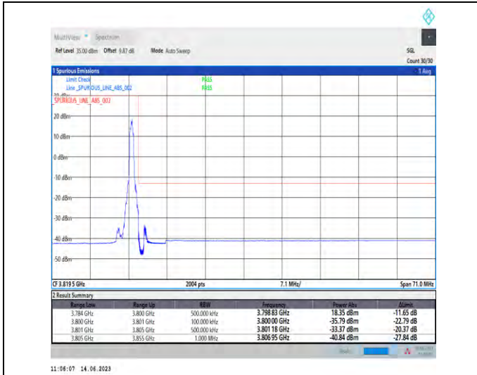
1-N78-3700-3800-PC1-30-50-H-2-DFT-PI2BPSK-Edge_1RB_Right-1@132-Ant1-1--PASS-see graph
