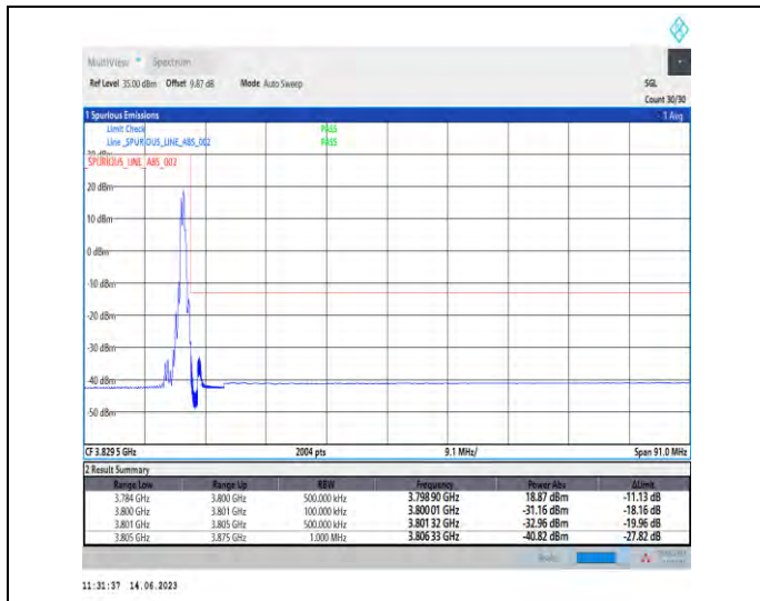
1-N78-3700-3800-PC1-30-70-H-2-DFT-PI2BPSK-Edge_1RB_Right-1@188-Ant1-1--PASS-see graph
