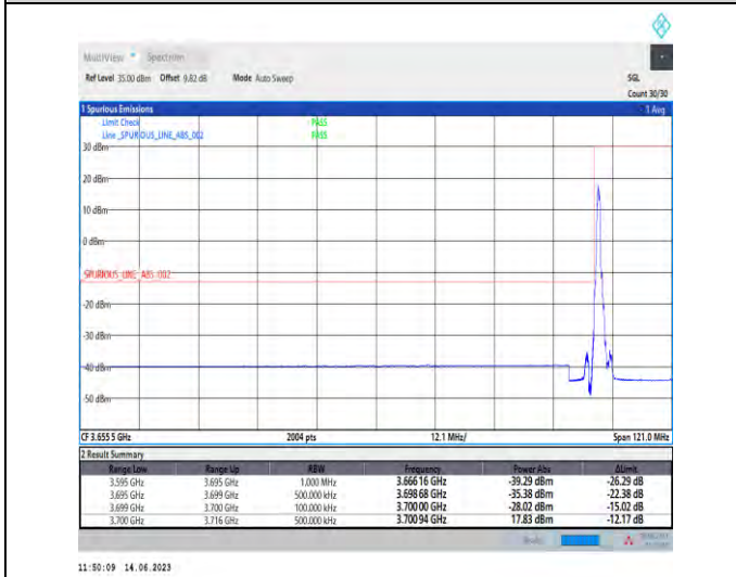
1-N78-3700-3800-PC1-30-100-L-4-CP-QPSK-Edge_1_RB_Left-1@0-Ant1-1--PASS-see graph
