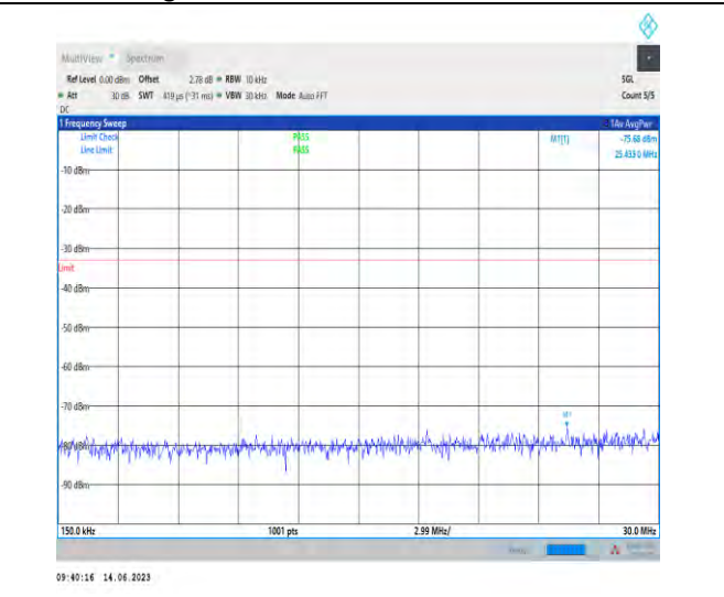
1-N78-3700-3800-PC1-30-100-H-1-N/A-DFT-QPSK-Edge_1RB_Left-1@0-0.15-30-Ant1-25.43--75.68--33-PASS
