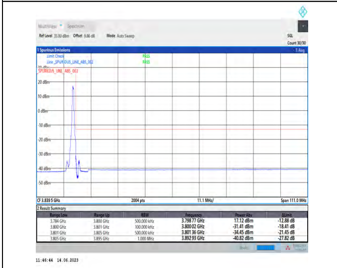
1-N78-3700-3800-PC1-30-90-H-5-CP-QPSK-Edge_1RB_Right-1@244-Ant1-1--PASS-see graph
