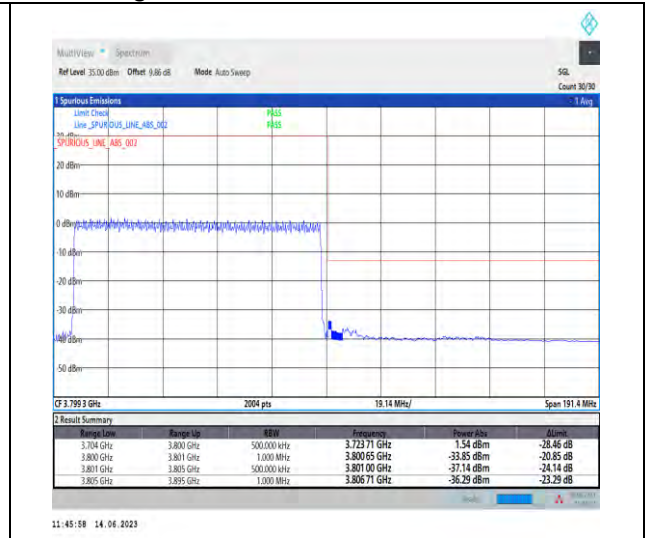
1-N78-3700-3800-PC1-30-90-H-3-DFT-PI2BPSK-Outer_Full-240@0-Ant1-1--PASS-see graph
