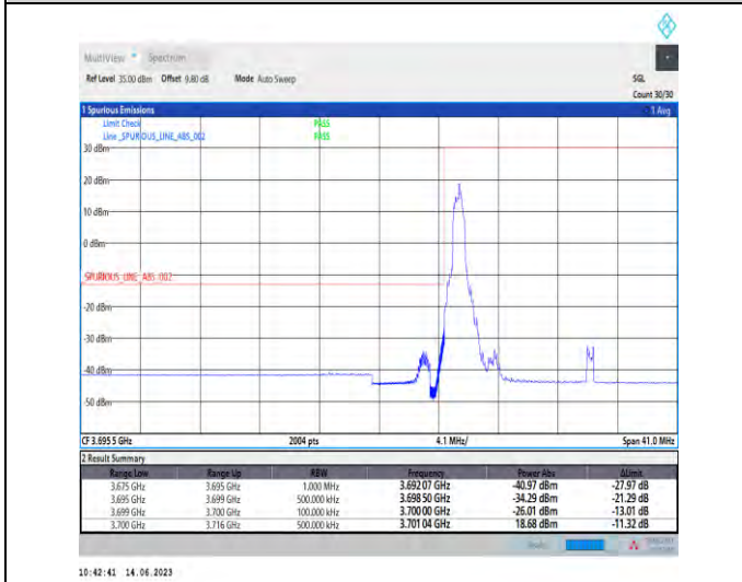
1-N78-3700-3800-PC1-30-20-L-4-CP-QPSK-Edge_1RB_Left-1@0-Ant1-1--PASS-see graph
