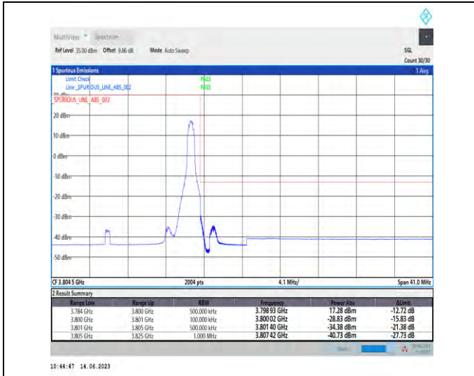
1-N78-3700-3800-PC1-30-20-H-2-DFT-PI2BPSK-Edge_1RB_Right-1@50-Ant1-1--PASS-see graph
