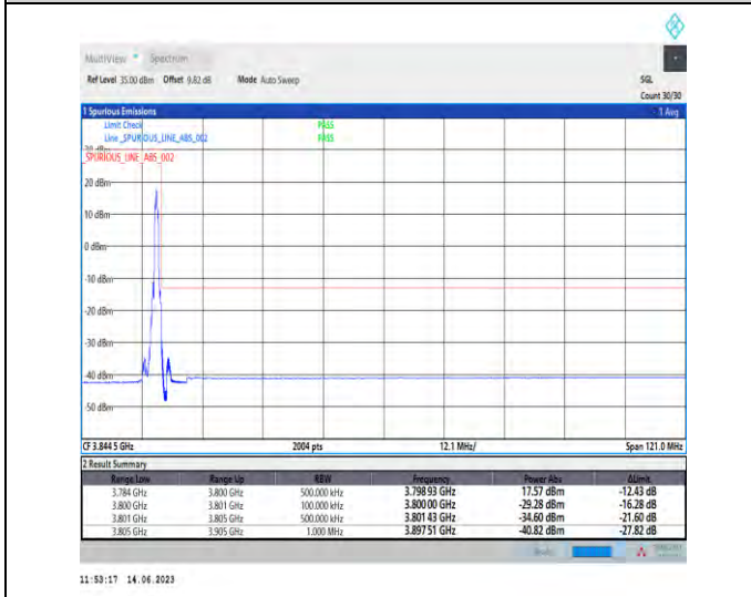
1-N78-3700-3800-PC1-30-100-H-5-CP-QPSK-Edge_1_RB_Right-1@272-Ant1-1--PASS-see graph
