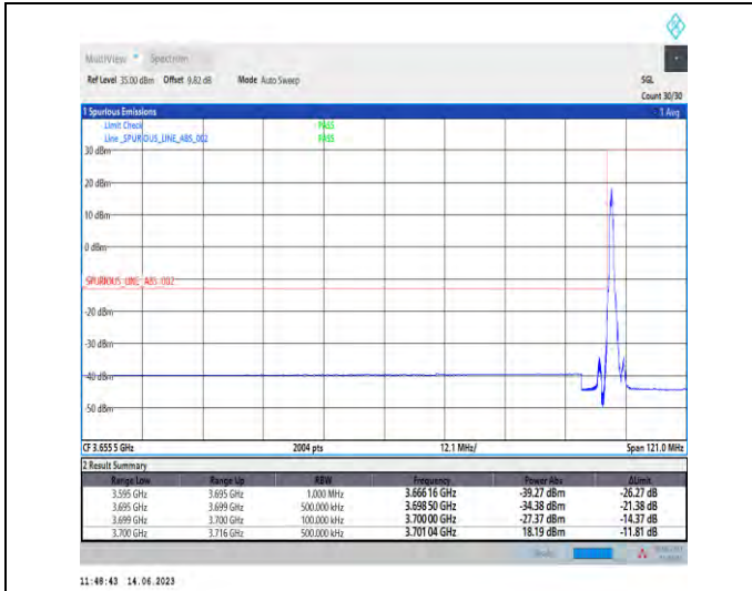
1-N78-3700-3800-PC1-30-100-L-1-DFT-PI2BPSK-Edge_1_RB_Left-1@0-Ant1-1--PASS-see graph
