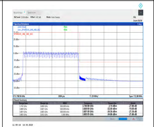
1-N78-3700-3800-PC1-30-50-H-6-CP-QPSK-Outer_Full-133@0-Ant1-1--PASS-see graph
