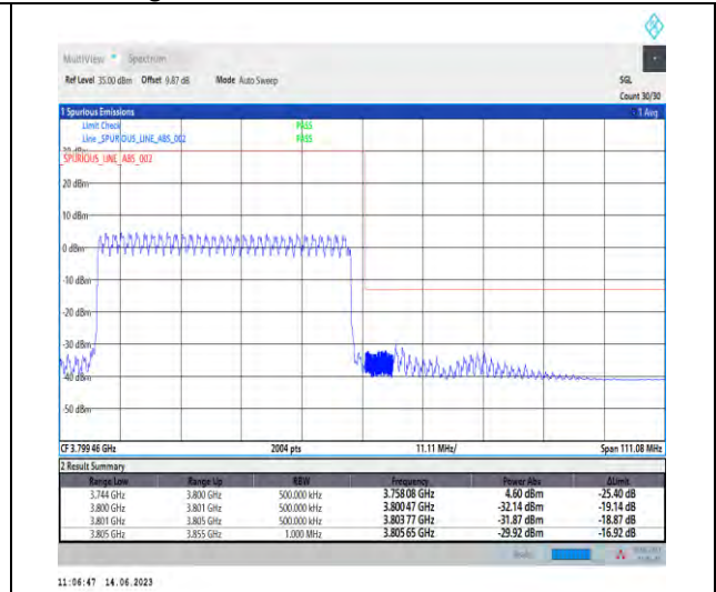
1-N78-3700-3800-PC1-30-50-H-3-DFT-PI2BPSK-Outer_Full-128@0-Ant1-1--PASS-see graph
