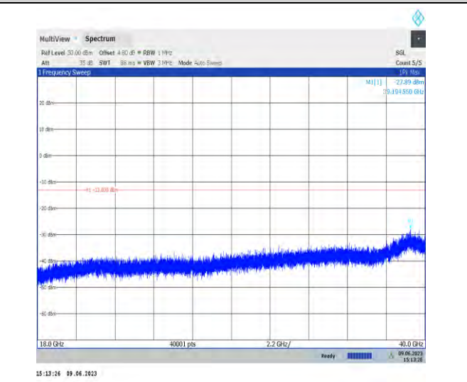
1-N78-3700-3800-PC1-30-100-M-1-N/A-DFT-QPSK-Edge_1RB_Left-1@0-18000-40000-Ant1-18000.00--42.27--13-PASS
