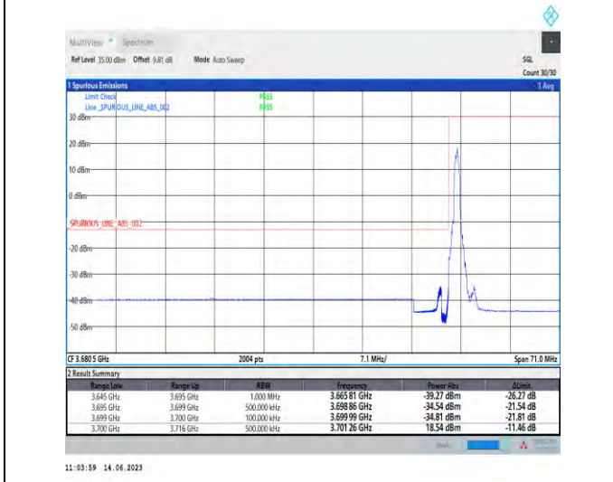
1-N78-3700-3800-PC1-30-50-L-4-CP-QPSK-Edge_1RB_Left-1@0-Ant1-1--PASS-see graph
