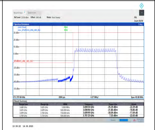
1-N78-3700-3800-PC1-30-15-L-6-CP-QPSK-Outer_Full-38@0-Ant1-1--PASS-see graph
