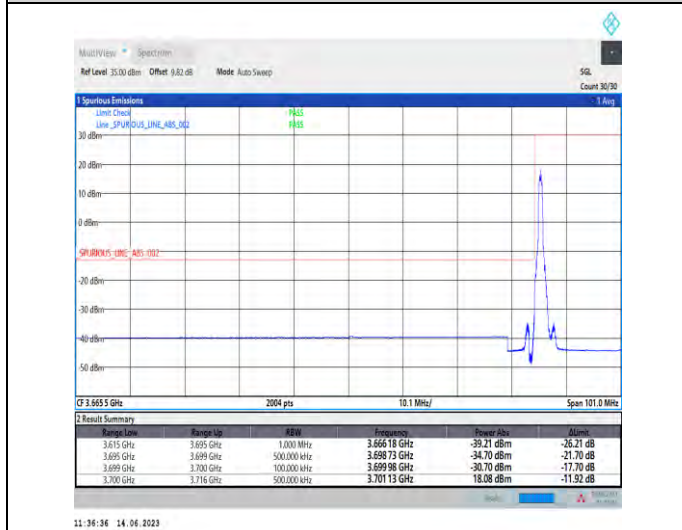
1-N78-3700-3800-PC1-30-80-L-4-CP-QPSK-Edge_1RB_Left-1@0-Ant1-1--PASS-see graph
