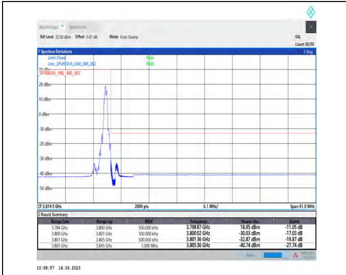
1-N78-3700-3800-PC1-30-40-H-2-DFT-PI2BPSK-Edge_1RB_Right-1@105-Ant1-1--PASS-see graph
