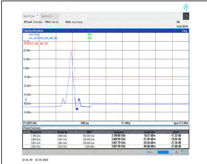
1-N78-3700-3800-PC1-30-30-H-2-DFT-PI2BPSK-Edge_1RB_Right-1@77-Ant1-1--PASS-see graph
