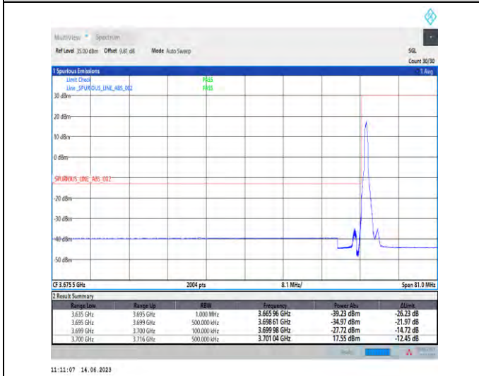
1-N78-3700-3800-PC1-30-60-L-4-CP-QPSK-Edge_1RB_Left-1@0-Ant1-1--PASS-see graph
