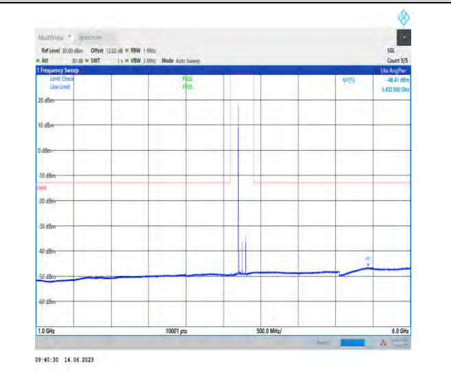
1-N78-3700-3800-PC1-30-100-H-1-N/A-DFT-QPSK-Edge_1RB_Left-1@0-1000-6000-Ant1-5432.50--46.41--13-PASS
