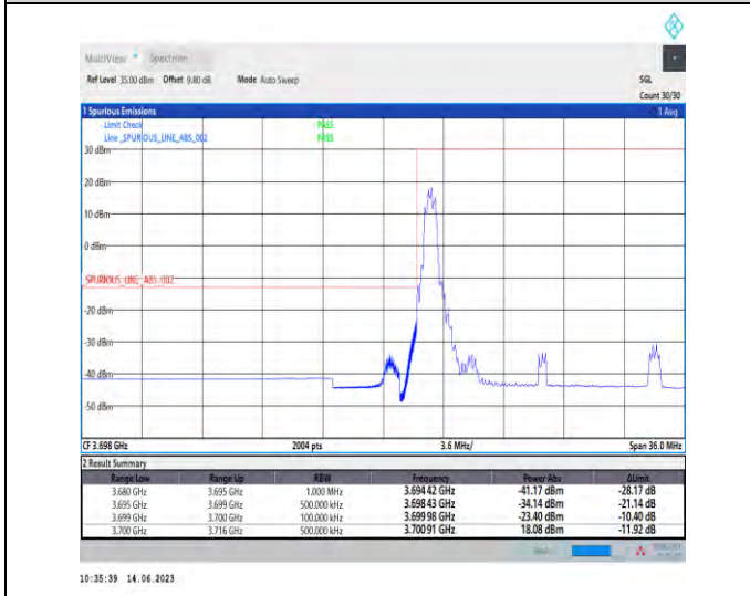
1-N78-3700-3800-PC1-30-15-L-4-CP-QPSK-Edge_1RB_Left-1@0-Ant1-1--PASS-see graph
