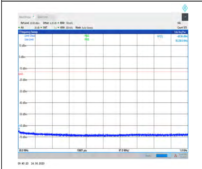
1-N78-3700-3800-PC1-30-100-H-1-N/A-DFT-QPSK-Edge_1RB_Left-1@0-30-1000-Ant1-35.24--63.56--13-PASS
