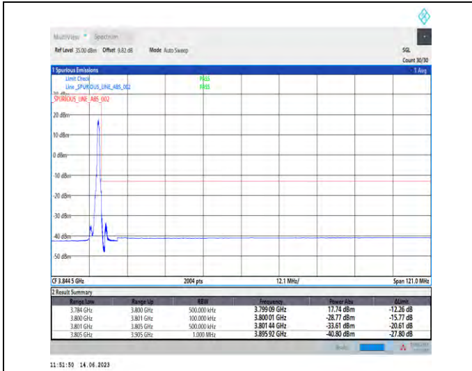
1-N78-3700-3800-PC1-30-100-H-2-DFT-PI2BPSK-Edge_1_RB_Right-1@272-Ant1-1--PASS-see graph
