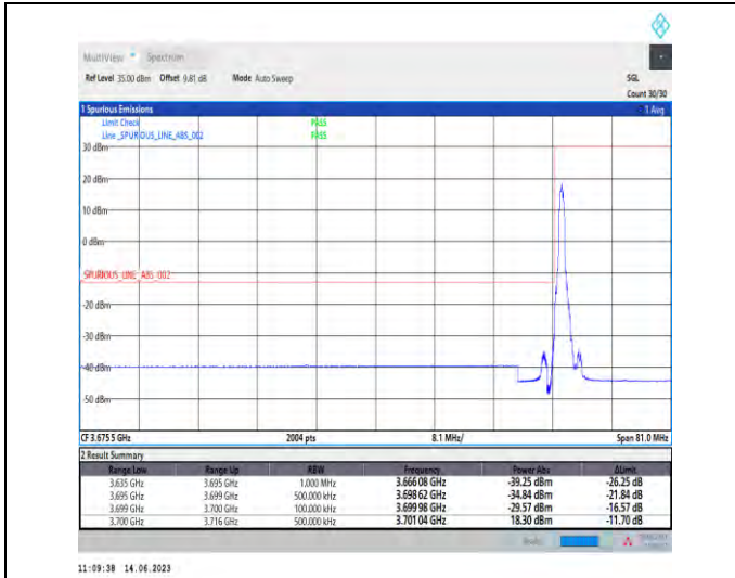
1-N78-3700-3800-PC1-30-60-L-1-DFT-PI2BPSK-Edge_1RB_Left-1@0-Ant1-1--PASS-see graph
