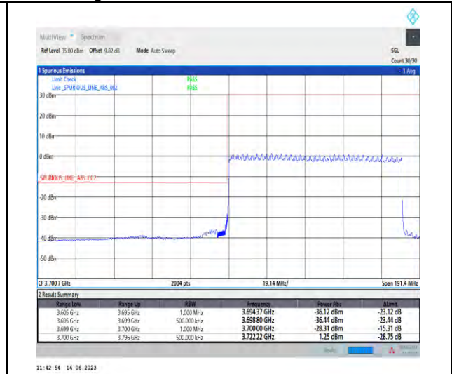
1-N78-3700-3800-PC1-30-90-L-3-DFT-PI2BPSK-Outer_Full-240@0-Ant1-1--PASS-see graph
