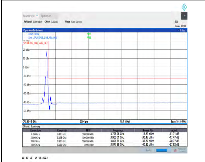
1-N78-3700-3800-PC1-30-80-H-5-CP-QPSK-Edge_1RB_Right-1@216-Ant1-1--PASS-see graph
