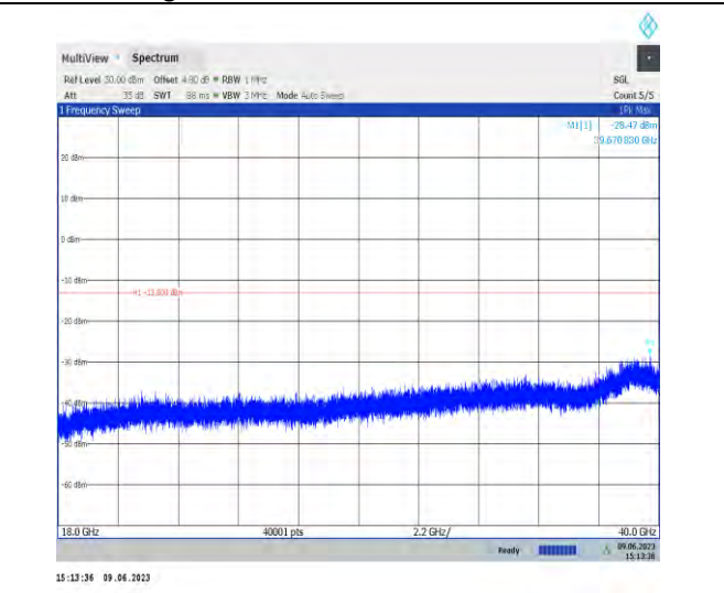
1-N78-3700-3800-PC1-30-100-H-1-N/A-DFT-QPSK-Edge_1RB_Left-1@0-18000-40000-Ant1-18000.00--42.18--13-PASS
