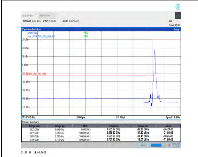
1-N78-3700-3800-PC1-30-70-L-4-CP-QPSK-Edge_1RB_Left-1@0-Ant1-1--PASS-see graph
