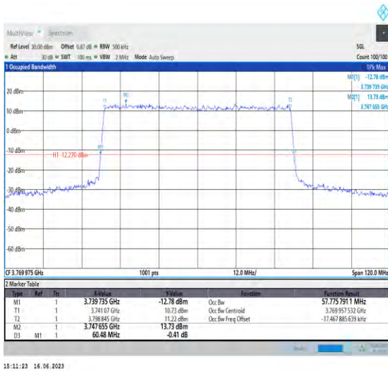
1-N78-3700-3800-PC1-30-60-H-7-CP-16QAM-Outer _Full-162@0-Ant1-57.776-60.480-≤60-PASS
