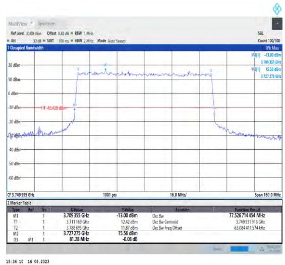
1-N78-3700-3800-PC1-30-80-M-7-CP-16QAM-Outer_Full-217@0-Ant1-77.527-81.280-≤80-PASS
