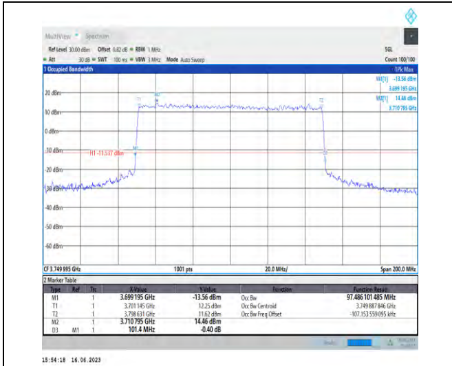
1-N78-3700-3800-PC1-30-100-L-7-CP-16QAM-Outer_Full-273@0-Ant1-97.486-101.400-≤100-PASS
