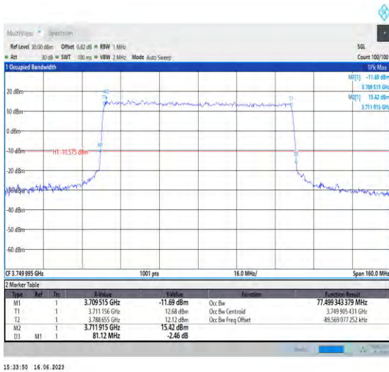
1-N78-3700-3800-PC1-30-80-M-6-CP-QPSK-Outer_Full-217@0-Ant1-77.499-81.120-≤80-PASS
