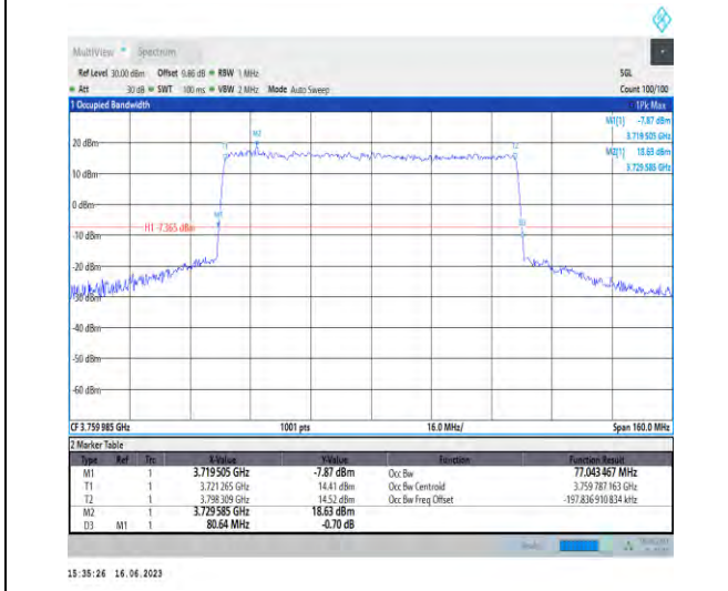
1-N78-3700-3800-PC1-30-80-H-1-DFT-QPSK-Outer_Full-216@0-Ant1-77.043-80.640-≤80-PASS
