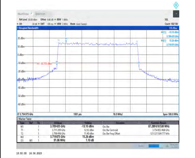
1-N78-3700-3800-PC1-30-90-H-7-CP-16QAM-Outer_Full-245@0-Ant1-87.29-91.080-≤90-PASS
