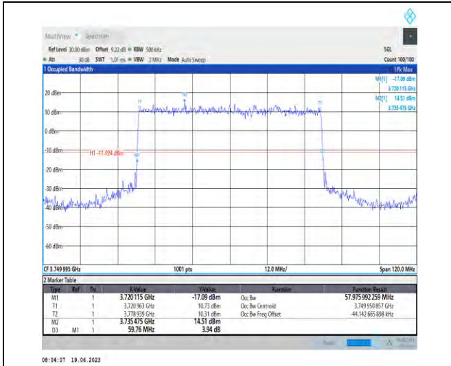
1-N78-3700-3800-PC1-30-60-M-2-DFT-PI2BPSK-Outer_Full-162@0-Ant1-57.976-59.760-≤60-PASS
