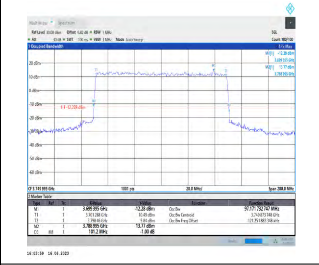
1-N78-3700-3800-PC1-30-100-H-8-CP-64QAM-Outer_Full-273@0-Ant1-97.172-101.200-≤100-PASS
