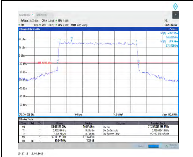
1-N78-3700-3800-PC1-30-80-L-3-DFT-16QAM-Outer_Full-216@0-Ant1-77.255-80.640-≤80-PASS
