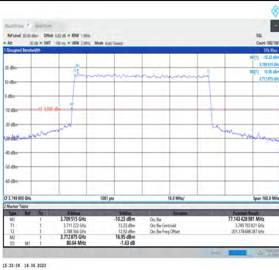
1-N78-3700-3800-PC1-30-80-M-4-DFT-64QAM-Outer_Full-216@0-Ant1-77.143-80.640-≤80-PASS
