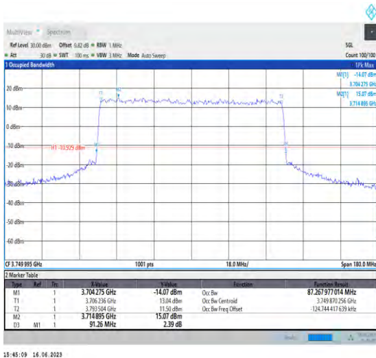
1-N78-3700-3800-PC1-30-90-M-7-CP-16QAM-Outer _Full-245@0-Ant1-87.268-91.260-≤90-PASS
