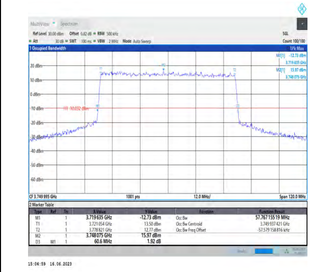
1-N78-3700-3800-PC1-30-60-M-1-DFT-QPSK-Outer_Full-162@0-Ant1-57.767-60.600-≤60-PASS
