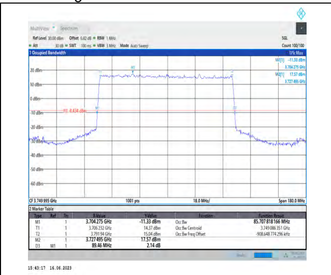
1-N78-3700-3800-PC1-30-90-M-2-DFT-PI2BPSK-Outer_Full-240@0-Ant1-85.708-89.460-≤90-PASS
