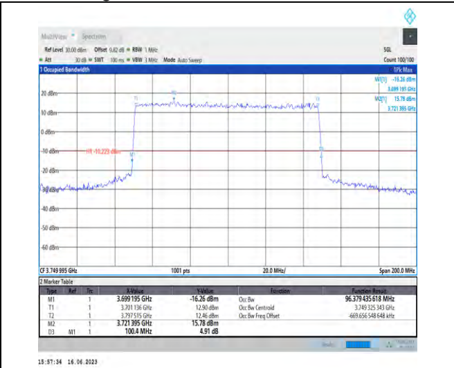
1-N78-3700-3800-PC1-30-100-M-3-DFT-16QAM-Out_Full-270@0-Ant1-96.379-100.400≤100-PASS
