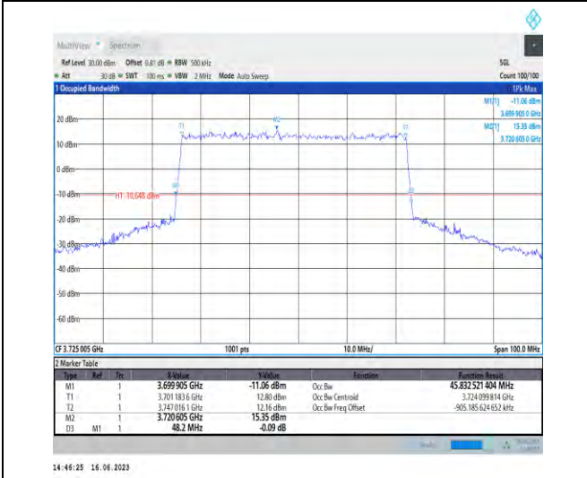
1-N78-3700-3800-PC1-30-50-L-4-DFT-64QAM-Outer_Full-128@0-Ant1-45.833-48.200-≤50-PASS
