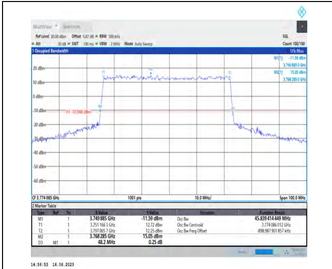
1-N78-3700-3800-PC1-30-50-H-4-DFT-64QAM-Outer_Full-128@0-Ant1-45.839-48.200-≤50-PASS
