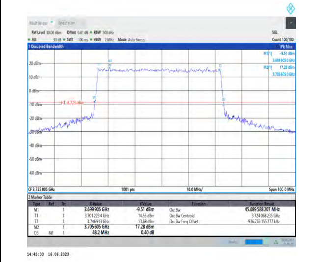
1-N78-3700-3800-PC1-30-50-L-1-DFT-QPSK-Outer_Full-128@0-Ant1-45.69-48.200-≤50-PASS
