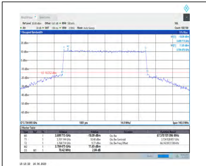
1-N78-3700-3800-PC1-30-70-L-8-CP-64QAM-Outer_Full-189@0-Ant1-67.57-70.420-≤70-PASS
