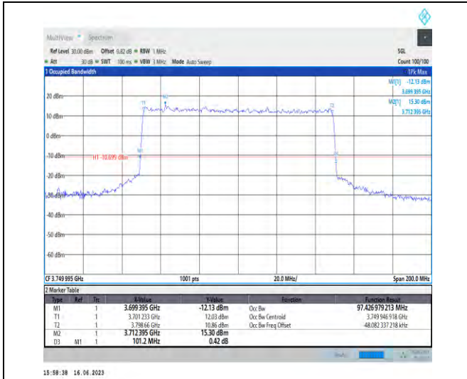
1-N78-3700-3800-PC1-30-100-M-6-CP-QPSK-Outer_Full-273@0-Ant1-97.427-101.200-≤100-PASS
