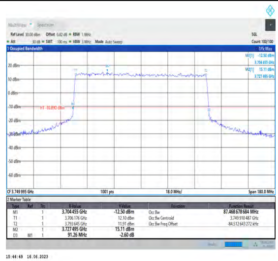
1-N78-3700-3800-PC1-30-90-M-6-CP-QPSK-Outer_ Full-245@0-Ant1-87.469-91.260-≤90-PASS
