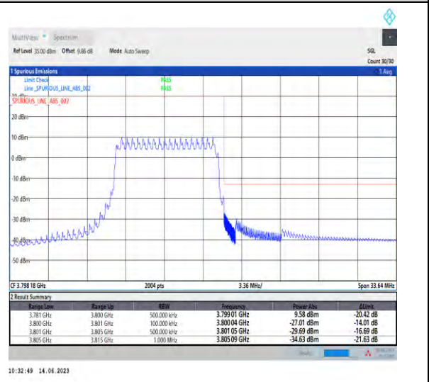
1-N78-3700-3800-PC1-30-10-H-6-CP-QPSK-Outer_Full-24@0-Ant1-1--PASS-see graph
