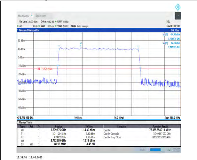
1-N78-3700-3800-PC1-30-80-M-9-CP-256QAM-Outer_Full-217@0-Ant1-77.386-80.960-≤80-PASS
