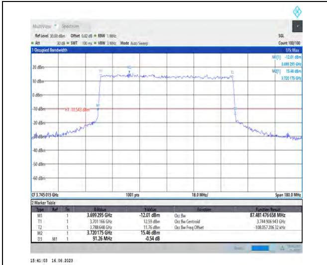
1-N78-3700-3800-PC1-30-90-L-6-CP-QPSK-Outer_Full-245@0-Ant1-87.481-91.260-≤90-PASS
