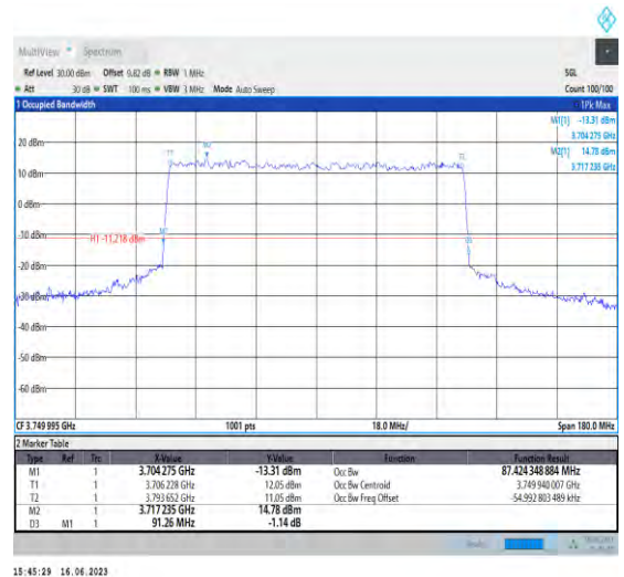
1-N78-3700-3800-PC1-30-90-M-8-CP-64QAM-Outer _Full-245@0-Ant1-87.424-91.260-≤90-PASS
