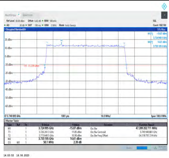
1-N78-3700-3800-PC1-30-50-M-6-CP-QPSK-Outer_Full-133@0-Ant1-47.399-50.100-≤50-PASS
