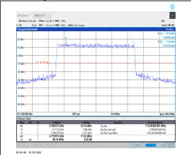
1-N78-3700-3800-PC1-30-80-M-1-DFT-QPSK-Outer_Full-216@0-Ant1-77.079-80.160-<math>\leq</math>80-PASS
