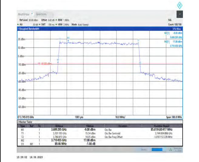
1-N78-3700-3800-PC1-30-90-L-1-DFT-QPSK-Outer_Full-240@0-Ant1-85.62-89.460-≤90-PASS
