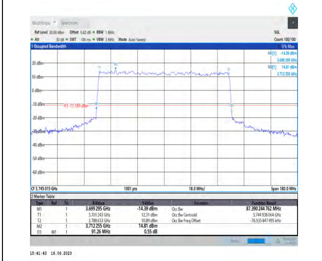
1-N78-3700-3800-PC1-30-90-L-8-CP-64QAM-Outer_Full-245@0-Ant1-87.39-91.260-≤90-PASS
