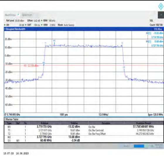
1-N78-3700-3800-PC1-30-60-M-7-CP-16QAM-Outer_Full-162@0-Ant1-57.759-60.480-≤60-PASS
