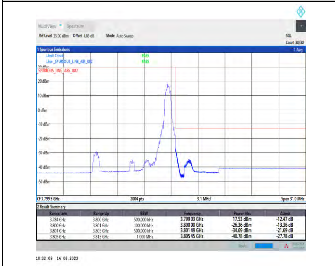
1-N78-3700-3800-PC1-30-10-H-5-CP-QPSK-Edge_1RB_Right-1@23-Ant1-1--PASS-see graph
