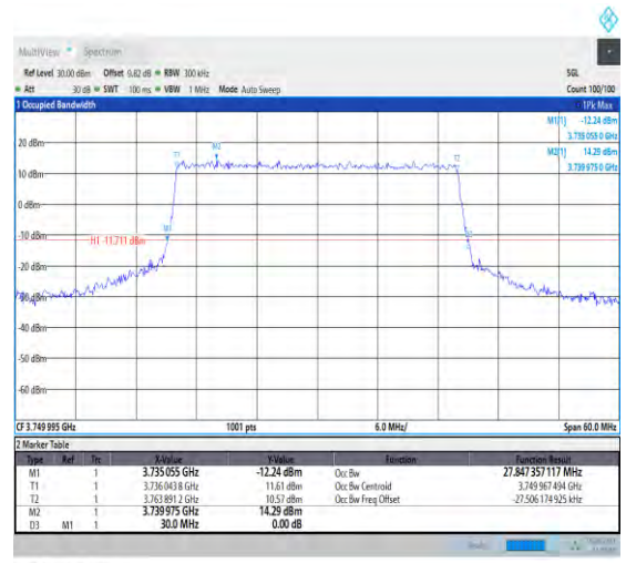
1-N78-3700-3800-PC1-30-30-M-6-CP-QPSK-Outer_Full-78@0-Ant1-27.847-30.000-≤30-PASS
