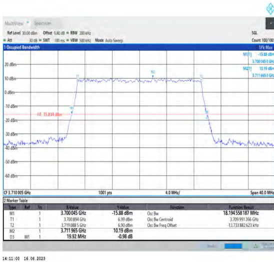
1-N78-3700-3800-PC1-30-20-L-9-CP-256QAM-Outer _Full-51@0-Ant1-18.195-19.920-≤20-PASS
