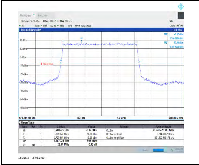
1-N78-3700-3800-PC1-30-30-L-2-DFT-PI2BPSK-Outer_Full-75@0-Ant1-26.741-28.440-≤30-PASS
