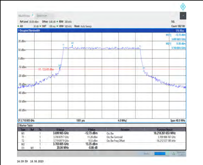
1-N78-3700-3800-PC1-30-20-L-6-CP-QPSK-Outer_Full-51@0-Ant1-18.218-20.040-≤20-PASS
