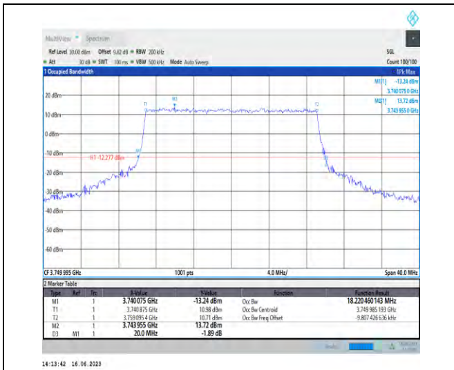
1-N78-3700-3800-PC1-30-20-M-6-CP-QPSK-Outer_Full-51@0-Ant1-18.22-20.000-≤20-PASS
