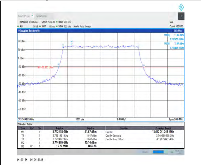
1-N78-3700-3800-PC1-30-15-M-6-CP-QPSK-Outer _Full-38@0-Ant1-13.612-15.270-≤15-PASS
