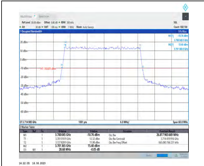
1-N78-3700-3800-PC1-30-30-L-4-DFT-64QAM-Outer_Full-75@0-Ant1-26.818-28.680-≤30-PASS
