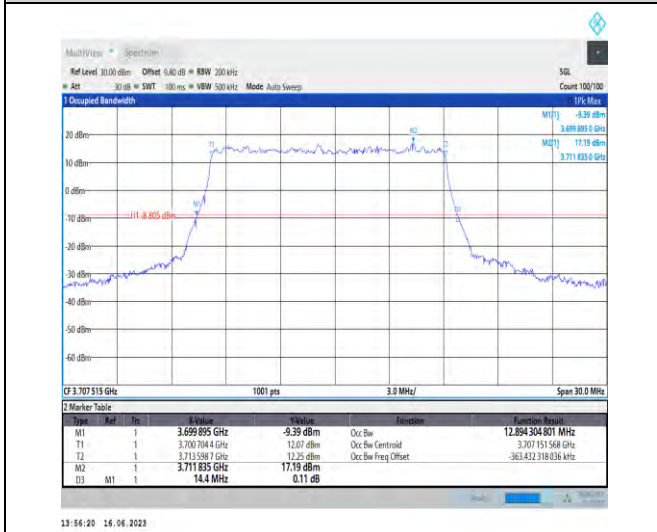
1-N78-3700-3800-PC1-30-15-L-4-DFT-64QAM-Outer_Full-36@0-Ant1-12.894-14.400-≤15-PASS
