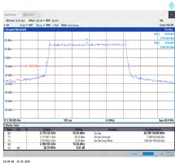
1-N78-3700-3800-PC1-30-30-H-1-DFT-QPSK-Outer _Full-75@0-Ant1-26.789-28.740-≤30-PASS
