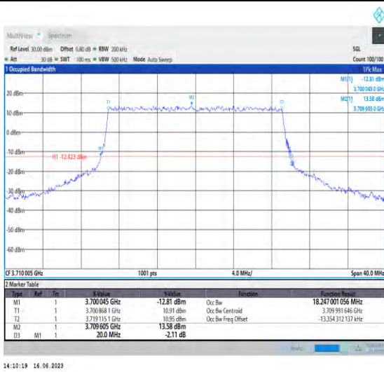
1-N78-3700-3800-PC1-30-20-L-7-CP-16QAM-Outer _Full-51@0-Ant1-18.247-20.000-≤20-PASS
