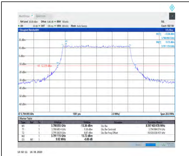
1-N78-3700-3800-PC1-30-10-H-7-CP-16QAM-Outer_Full-24@0-Ant1-8.597-9.920-≤10-PASS
