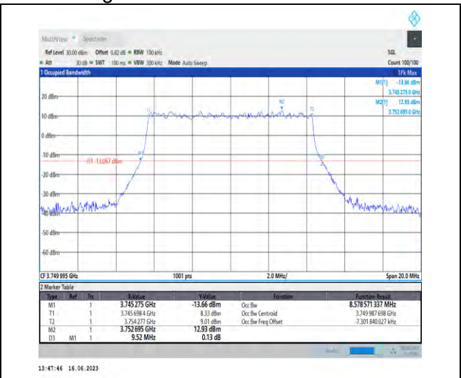
1-N78-3700-3800-PC1-30-10-M-5-DFT-256QAM-Outer_Full-24@0-Ant1-8.579-9.520-≤10-PASS
