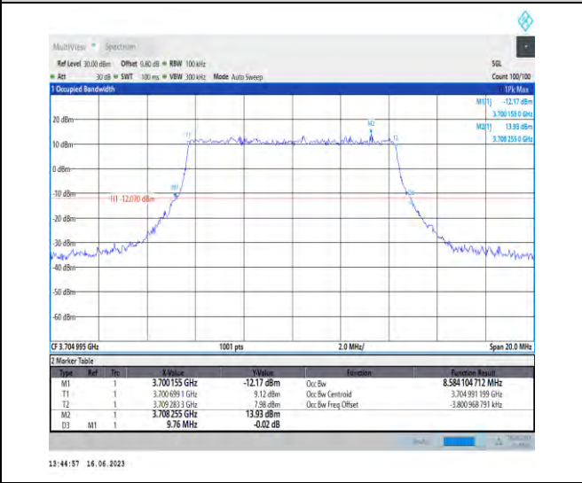
1-N78-3700-3800-PC1-30-10-L-8-CP-64QAM-Outer _Full-24@0-Ant1-8.584-9.760-≤10-PASS
