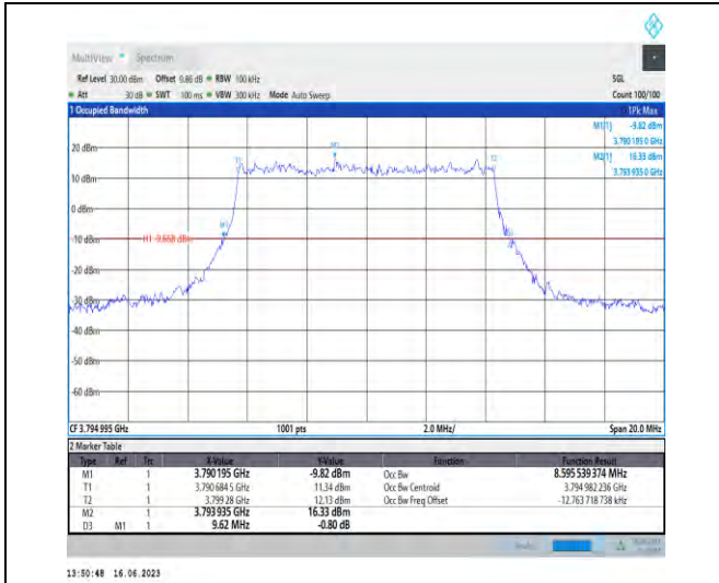
1-N78-3700-3800-PC1-30-10-H-3-DFT-16QAM-Outer_Full-24@0-Ant1-8.596-9.620-≤10-PASS
