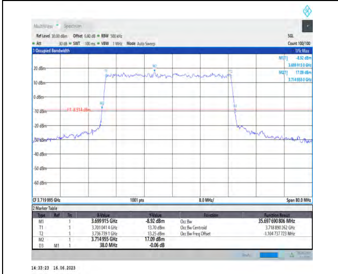
1-N78-3700-3800-PC1-30-40-L-3-DFT-16QAM-Outer_Full-100@0-Ant1-35.698-38.000-≤40-PASS
