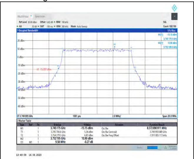
1-N78-3700-3800-PC1-30-10-M-9-CP-256QAM-Outer_Full-24@0-Ant1-8.573-9.580-≤10-PASS
