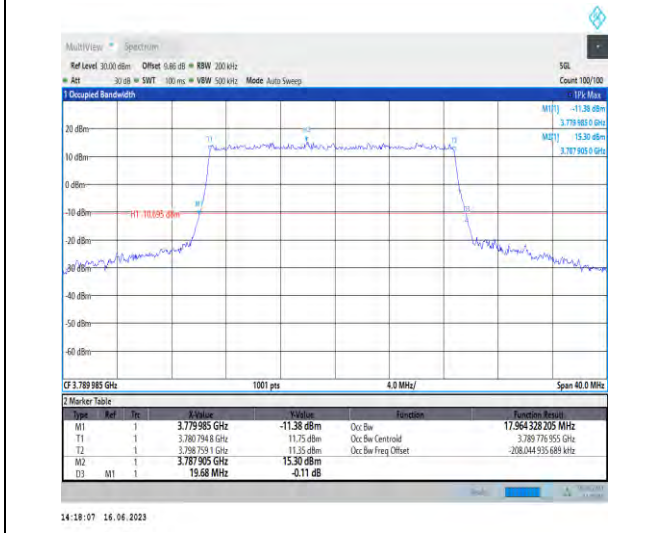
1-N78-3700-3800-PC1-30-20-H-3-DFT-16QAM-Outer_Full-50@0-Ant1-17.964-19.680-≤20-PASS
