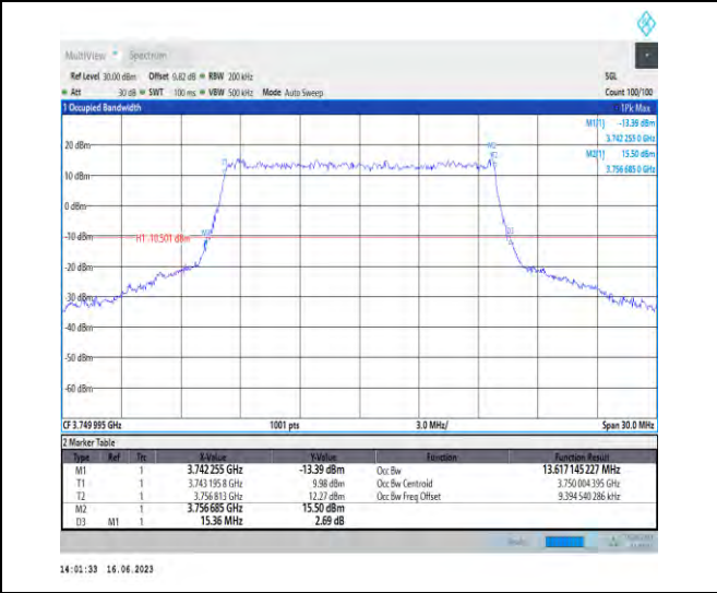
1-N78-3700-3800-PC1-30-15-M-8-CP-64QAM-Outer _Full-38@0-Ant1-13.617-15.360-≤15-PASS
