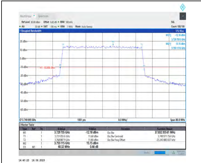
1-N78-3700-3800-PC1-30-40-M-8-CP-64QAM-Outer_Full-106@0-Ant1-37.832-40.320-≤40-PASS
