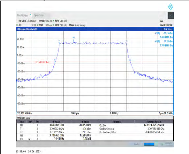
1-N78-3700-3800-PC1-30-15-L-3-DFT-16QAM-Out er_Full-36@0-Ant1-12.897-14.400-≤15-PASS
