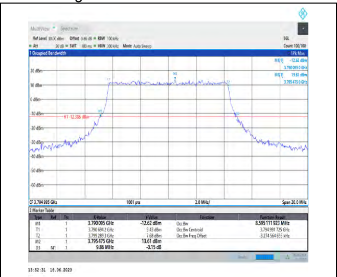
1-N78-3700-3800-PC1-30-10-H-8-CP-64QAM-Outer_Full-24@0-Ant1-8.595-9.860-≤10-PASS
