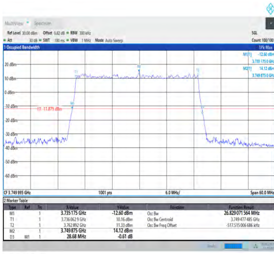
1-N78-3700-3800-PC1-30-30-M-5-DFT-256QAM-Outer_Full-75@0-Ant1-26.829-28.680-≤30-PASS
