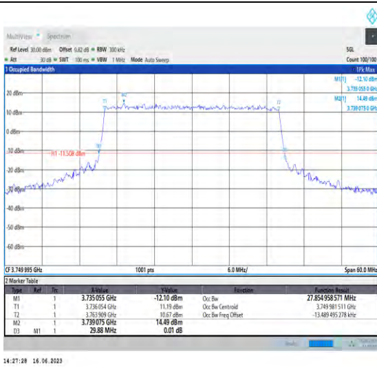
1-N78-3700-3800-PC1-30-30-M-7-CP-16QAM-Outer _Full-78@0-Ant1-27.855-29.880-≤30-PASS
