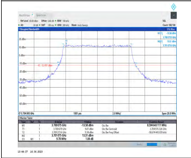
1-N78-3700-3800-PC1-30-10-L-7-CP-16QAM-Outer _Full-24@0-Ant1-8.595-9.780-≤10-PASS
