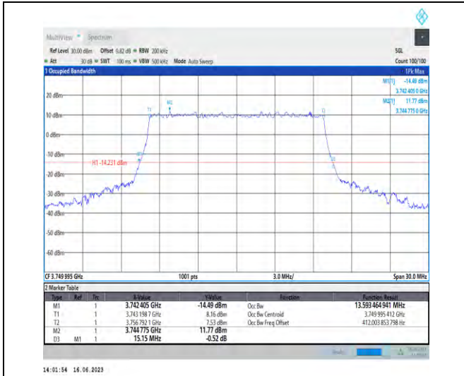
1-N78-3700-3800-PC1-30-15-M-9-CP-256QAM-Outer_Full-38@0-Ant1-13.593-15.150-≤15-PASS
