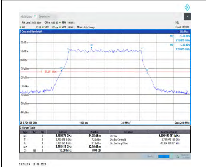
1-N78-3700-3800-PC1-30-10-H-5-DFT-256QAM-Outer_Full-24@0-Ant1-8.6-10.080-≤10-PASS
