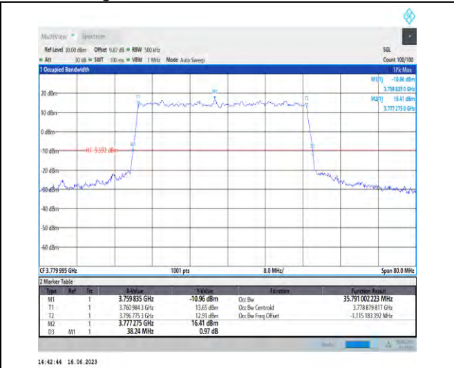
1-N78-3700-3800-PC1-30-40-H-4-DFT-64QAM-Outer_Full-100@0-Ant1-35.791-38.240-≤40-PASS
