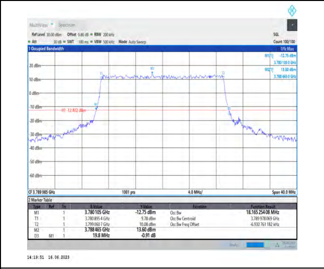
1-N78-3700-3800-PC1-30-20-H-8-CP-64QAM-Outer _Full-51@0-Ant1-18.165-19.800-≤20-PASS
