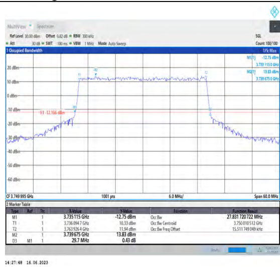
1-N78-3700-3800-PC1-30-30-M-8-CP-64QAM-Outer _Full-78@0-Ant1-27.832-29.700-≤30-PASS
