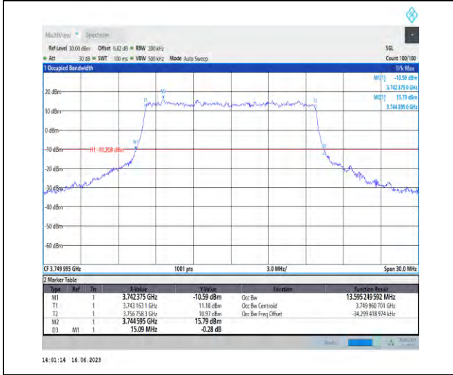
1-N78-3700-3800-PC1-30-15-M-7-CP-16QAM-Outer _Full-38@0-Ant1-13.595-15.090-≤15-PASS
