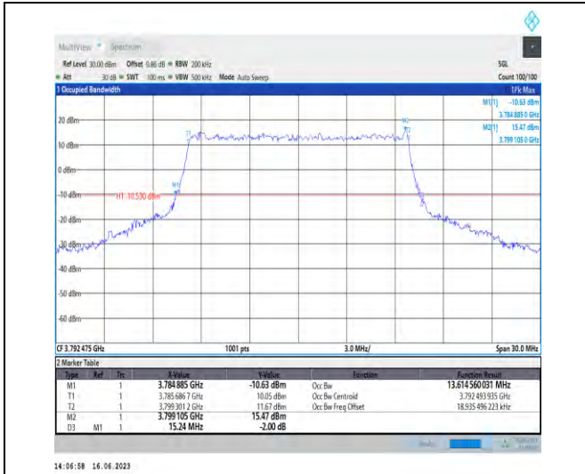
1-N78-3700-3800-PC1-30-15-H-8-CP-64QAM-Outer_Full-38@0-Ant1-13.615-15.240-≤15-PASS
