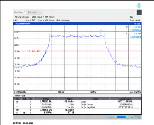
1-N78-3700-3800-PC1-30-10-M-3-DFT-16QAM-Outer_Full-24@0-Ant1-8.613-9.840-≤10-PASS
