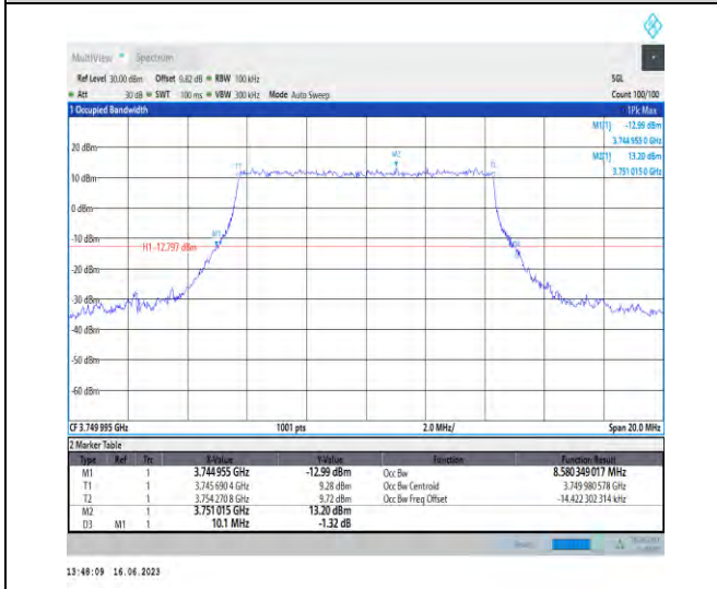
1-N78-3700-3800-PC1-30-10-M-6-CP-QPSK-Outer_Full-24@0-Ant1-8.58-10.100-≤10-PASS
