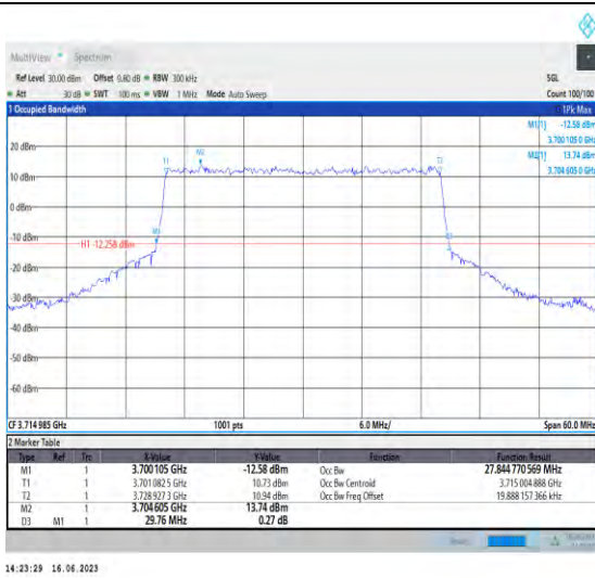
1-N78-3700-3800-PC1-30-30-L-8-CP-64QAM-Outer_Full-78@0-Ant1-27.845-29.760-≤30-PASS
