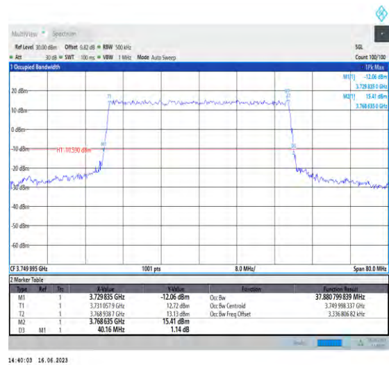
1-N78-3700-3800-PC1-30-40-M-7-CP-16QAM-Outer_Full-106@0-Ant1-37.881-40.160-≤40-PASS
