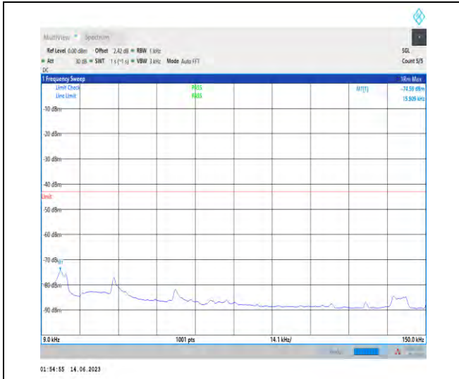
1-N78-3450-3550-PC1.5-30-100-H-1-N/A-DFT-QPS K-Edge_1RB_Left-1@0-0.009-0.15-Ant1-0.02--74.5 9--43-PASS
