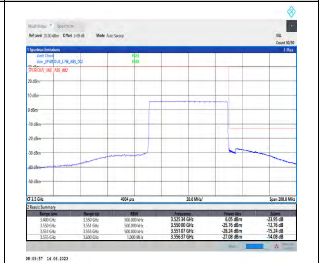
1-N78-3450-3550-PC1.5-30-60-H-6-CP-QPSK-Outer_Full-162@0-Ant1-1--PASS-see graph
