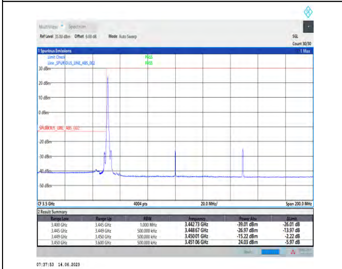
1-N78-3450-3550-PC1.5-30-100-L-4-CP-QPSK-Edge_1RB_Left-1@0-Ant1-1--PASS-see graph
