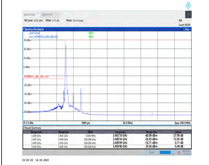
1-N78-3450-3550-PC1.5-30-20-L-4-CP-QPSK-Edge_1RB_Left-1@0-Ant1-1--PASS-see graph
