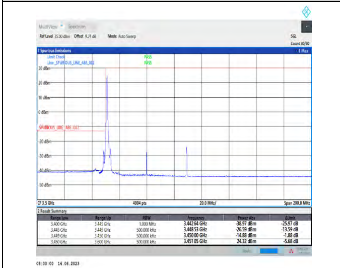
1-N78-3450-3550-PC1.5-30-60-L-4-CP-QPSK-Edge_1RB_Left-1@0-Ant1-1-PASS-see graph
