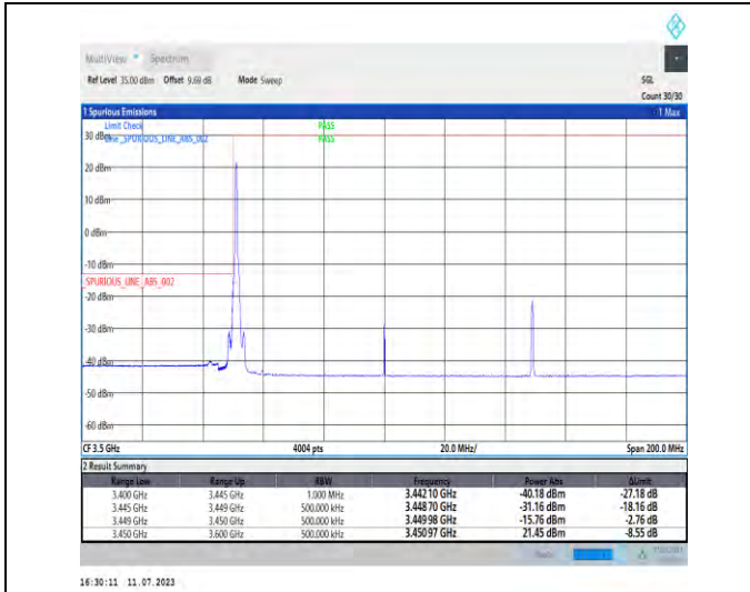
1-N78-3450-3550-PC1.5-30-100-L-1-DFT-PI2BPSK-E dge_1RB_Left-1@0-Ant1-1--PASS-see graph
