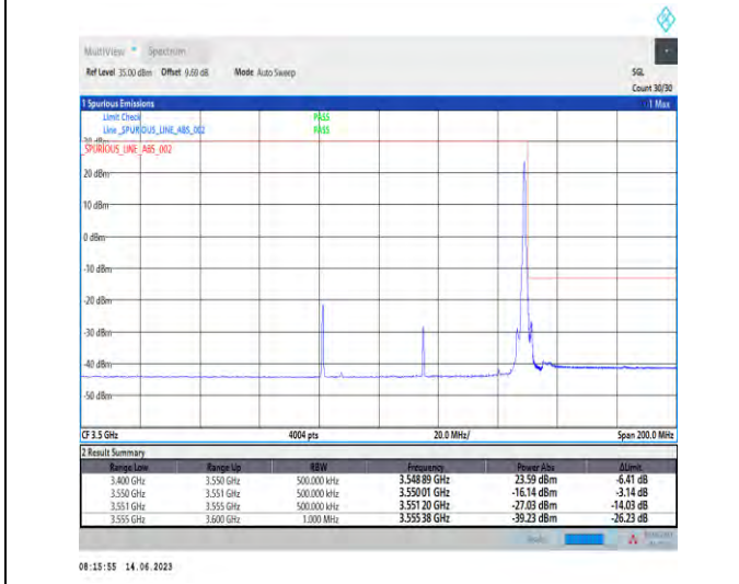
1-N78-3450-3550-PC1.5-30-70-H-5-CP-QPSK-Edge_1RB_Right-1@188-Ant1-1--PASS-see graph
