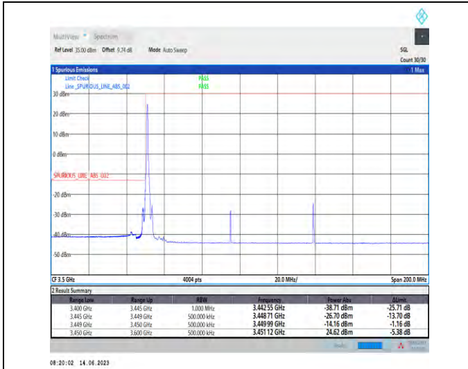
1-N78-3450-3550-PC1.5-30-90-L-1-DFT-PI2BPSK-Edge_1RB_Left-1@0-Ant1-1-PASS-see graph
