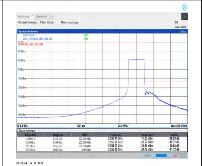
1-N78-3450-3550-PC1.5-30-20-H-6-CP-QPSK-Outer_Full-51@0-Ant1-1--PASS-see graph
