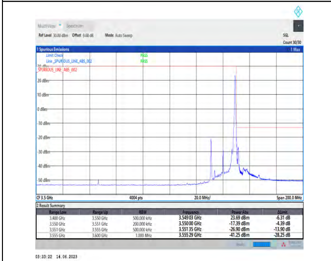
1-N78-3450-3550-PC1.5-30-20-H-5-CP-QPSK-Edge_1RB_Right-1@50-Ant1-1--PASS-see graph
