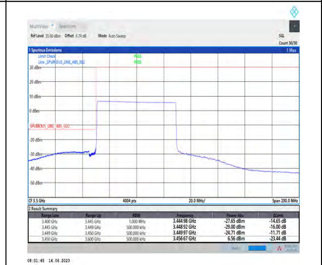
1-N78-3450-3550-PC1.5-30-60-L-6-CP-QPSK-Outer_Full-162@0-Ant1-1-PASS-see graph
