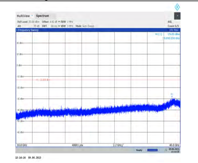
1-N78-3450-3550-PC1.5-30-100-L-1-N/A-DFT-QPSK -Edge_1RB_Left-1@0-18000-38000-Ant1-18000.00-- 50.19--13-PASS
