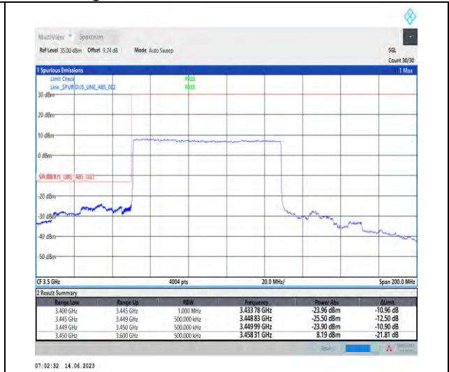
1-N78-3450-3550-PC1.5-30-80-L-3-DFT-PI2BPSK-Outer_Full-216@0-Ant1-1-PASS-see graph
