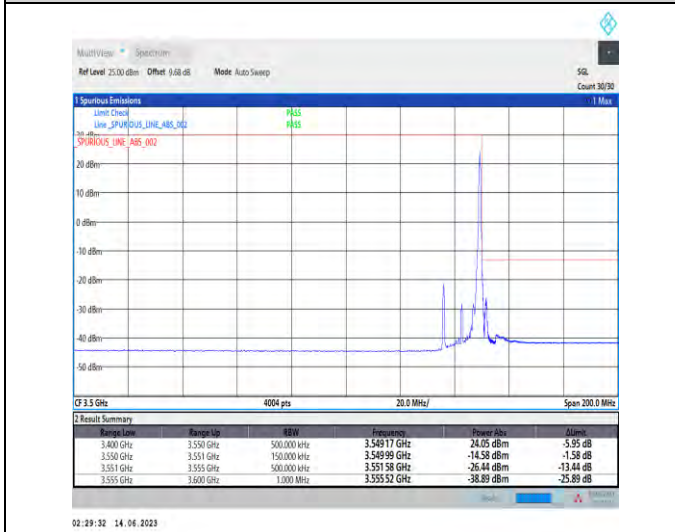
1-N78-3450-3550-PC1.5-30-15-H-5-CP-QPSK-Edge_1RB_Right-1@37-Ant1-1--PASS-see graph
