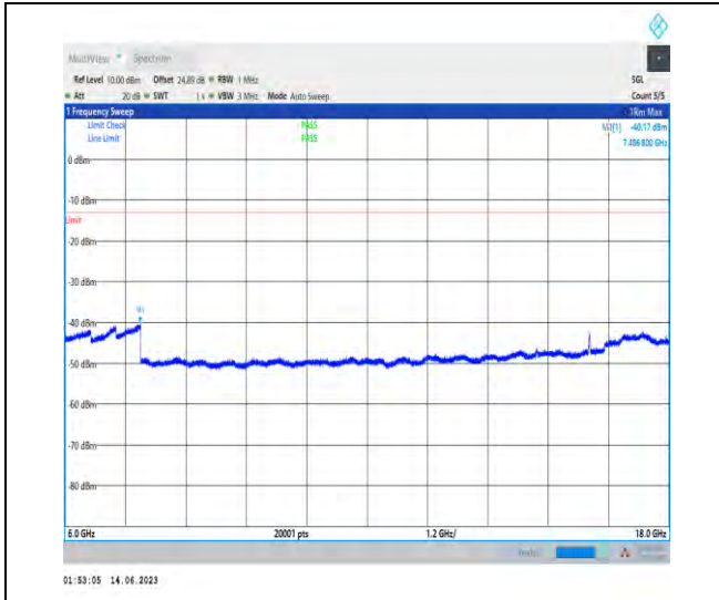
1-N78-3450-3550-PC1.5-30-100-L-1-N/A-DFT-QPS K-Edge_1RB_Left-1@0-6000-18000-Ant1-7486.80-- 40.17--13-PASS
