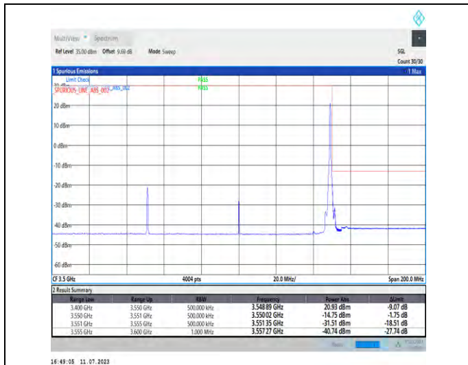
1-N78-3450-3550-PC1.5-30-100-H-2-DFT-PI2BPSK-E dge_1RB_Right-1@272-Ant1-1--PASS-see graph
