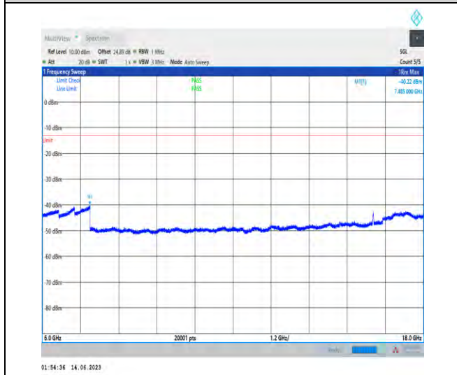
1-N78-3450-3550-PC1.5-30-100-M-1-N/A-DFT-QPSK K-Edge_1RB_Left-1@0-6000-18000-Ant1-7485.00-- 40.22--13-PASS
