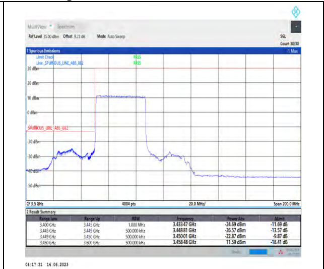
1-N78-3450-3550-PC1.5-30-40-L-3-DFT-PI2BPSK-Outer_Full-100@0-Ant1-1--PASS-see graph
