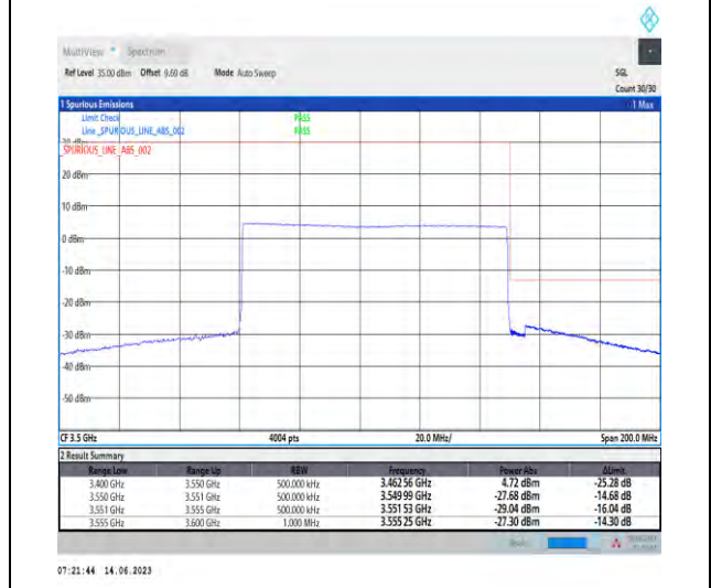
1-N78-3450-3550-PC1.5-30-90-H-6-CP-QPSK-Outer_Full-245@0-Ant1-1--PASS-see graph
