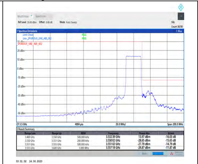
1-N78-3450-3550-PC1.5-30-20-H-3-DFT-PI2BPSK-Outer_Full-50@0-Ant1-1--PASS-see graph
