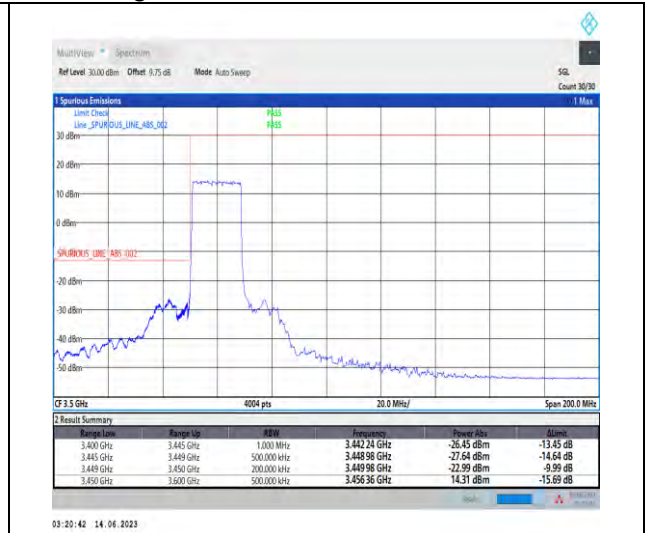
1-N78-3450-3550-PC1.5-30-20-L-3-DFT-PI2BPSK-Outer_Full-50@0-Ant1-1--PASS-see graph
