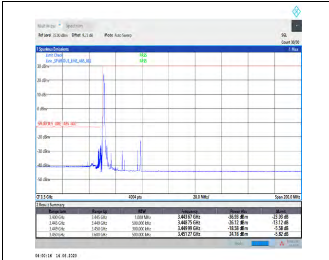
1-N78-3450-3550-PC1.5-30-30-L-1-DFT-PI2BPSK-Edge_1RB_Left-1@0-Ant1-1--PASS-see graph
