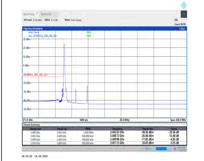
1-N78-3450-3550-PC1.5-30-30-L-4-CP-QPSK-Edge_1RB_Left-1@0-Ant1-1--PASS-see graph
