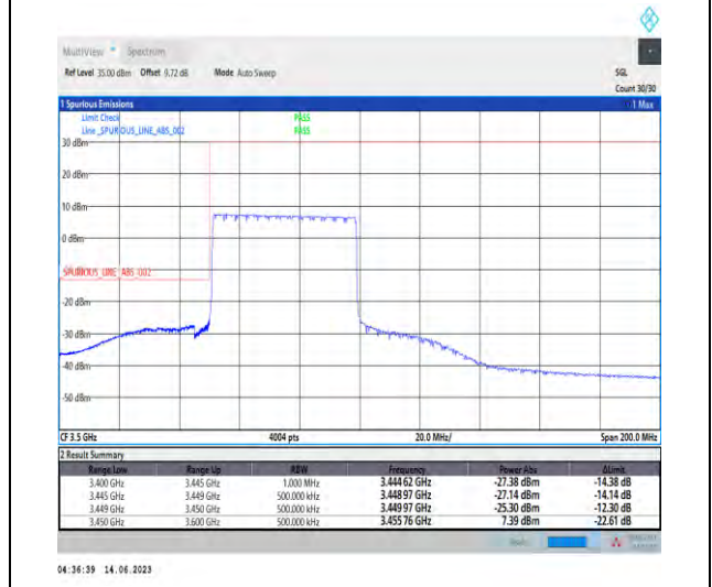
1-N78-3450-3550-PC1.5-30-50-L-6-CP-QPSK-Outer_Full-133@0-Ant1-1-PASS-see graph
