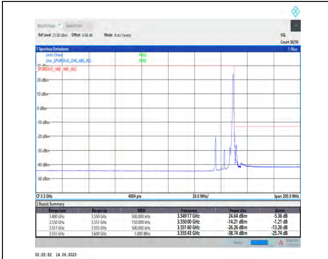
1-N78-3450-3550-PC1.5-30-15-H-2-DFT-PI2BPSK-Edge_1RB_Right-1@37-Ant1-1--PASS-see graph
