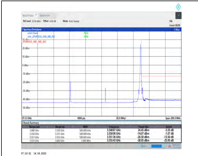
1-N78-3450-3550-PC1.5-30-90-H-2-DFT-PI2BPSK-Edge_1RB_Right-1@244-Ant1-1--PASS-see graph
