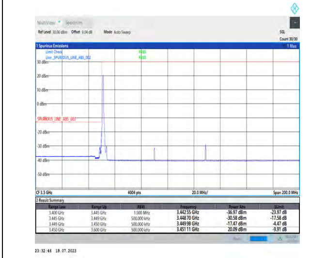
1-N78-3450-3550-PC1.5-30-80-L-4-CP-QPSK-Edge_1RB_Left-1@0-Ant1-1-PASS-see graph
