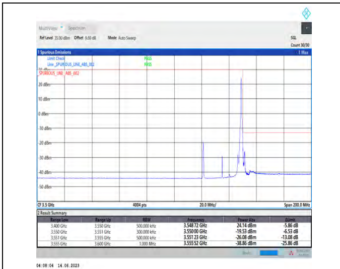
1-N78-3450-3550-PC1.5-30-30-H-2-DFT-PI2BPSK-Edge_1RB_Right-1@77-Ant1-1--PASS-see graph
