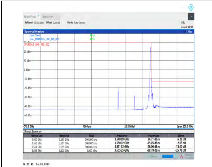
1-N78-3450-3550-PC1.5-30-40-H-2-DFT-PI2BPSK-Edge_1RB_Right-1@105-Ant1-1--PASS-see graph
