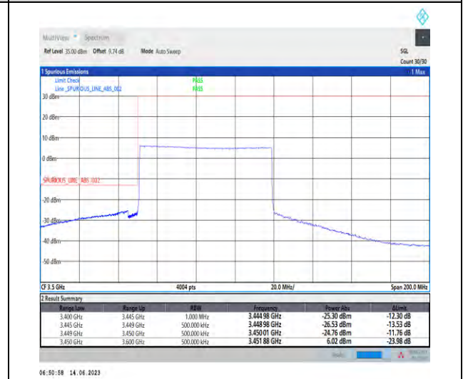
1-N78-3450-3550-PC1.5-30-70-L-6-CP-QPSK-Outer_Full-189@0-Ant1-1-PASS-see graph
