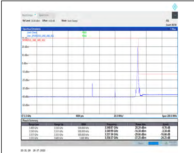
1-N78-3450-3550-PC1.5-30-60-H-2-DFT-PI2BPSK-Edge_1RB_Right-1@161-Ant1-1--PASS-see graph
