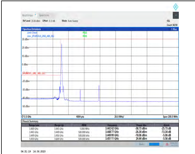
1-N78-3450-3550-PC1.5-30-50-L-1-DFT-PI2BPSK-Edge_1RB_Left-1@0-Ant1-1-PASS-see graph
