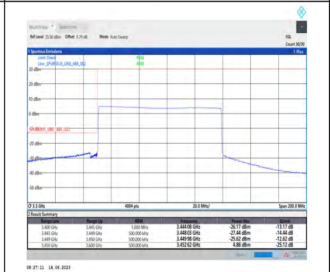
1-N78-3450-3550-PC1.5-30-90-L-6-CP-QPSK-Outer_Full-245@0-Ant1-1-PASS-see graph
