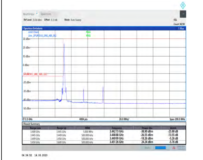
1-N78-3450-3550-PC1.5-30-50-L-4-CP-QPSK-Edge_1RB_Left-1@0-Ant1-1-PASS-see graph
