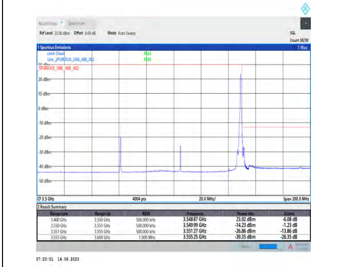
1-N78-3450-3550-PC1.5-30-90-H-5-CP-QPSK-Edge_1RB_Right-1@244-Ant1-1--PASS-see graph
