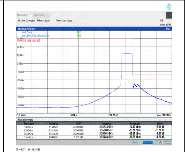
1-N78-3450-3550-PC1.5-30-15-H-6-CP-QPSK-Outer_Full-38@0-Ant1-1--PASS-see graph
