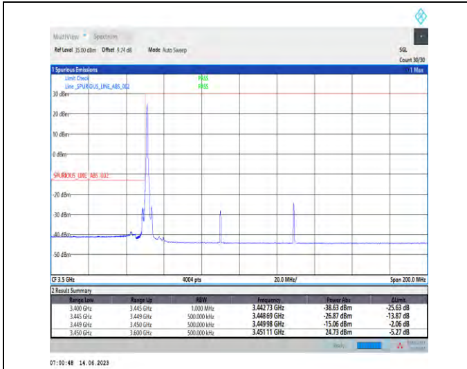
1-N78-3450-3550-PC1.5-30-80-L-1-DFT-PI2BPSK-Edge_1RB_Left-1@0-Ant1-1-PASS-see graph
