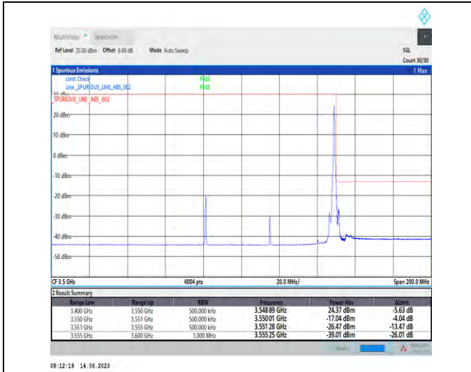
1-N78-3450-3550-PC1.5-30-70-H-2-DFT-PI2BPSK-Edge_1RB_Right-1@188-Ant1-1--PASS-see graph
