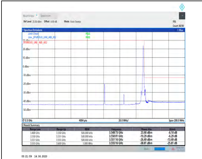
1-N78-3450-3550-PC1.5-30-50-H-2-DFT-PI2BPSK-Edge_1RB_Right-1@132-Ant1-1--PASS-see graph
