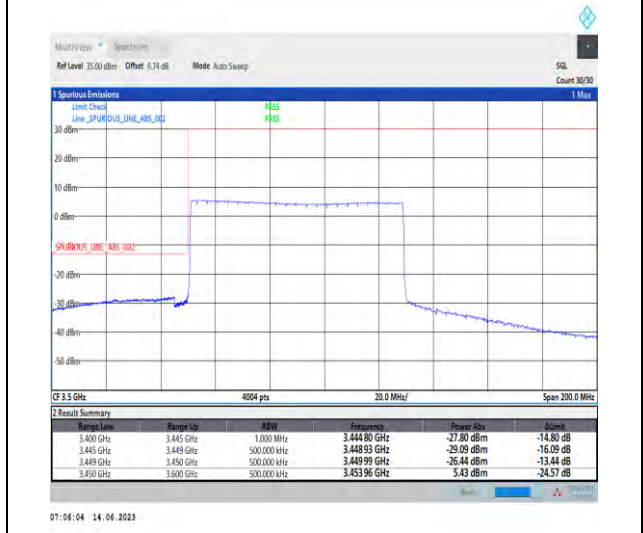
1-N78-3450-3550-PC1.5-30-80-L-6-CP-QPSK-Outer_Full-217@0-Ant1-1-PASS-see graph
