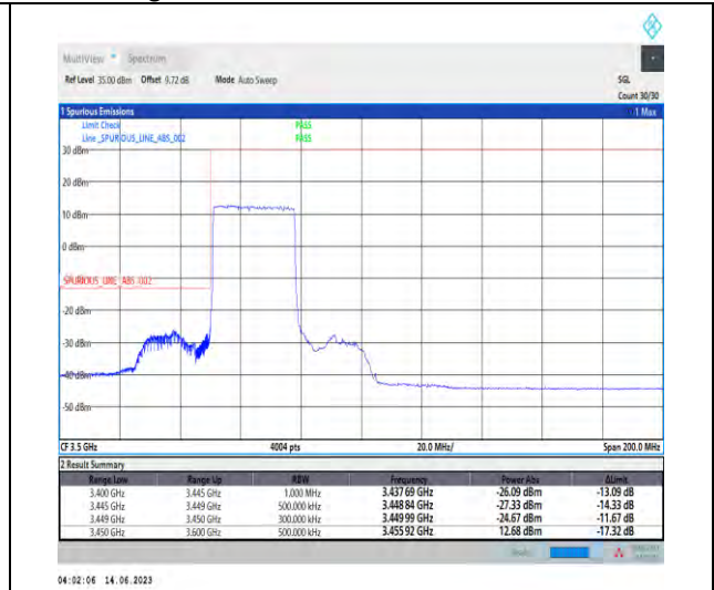
1-N78-3450-3550-PC1.5-30-30-L-3-DFT-PI2BPSK-Outer_Full-75@0-Ant1-1--PASS-see graph
