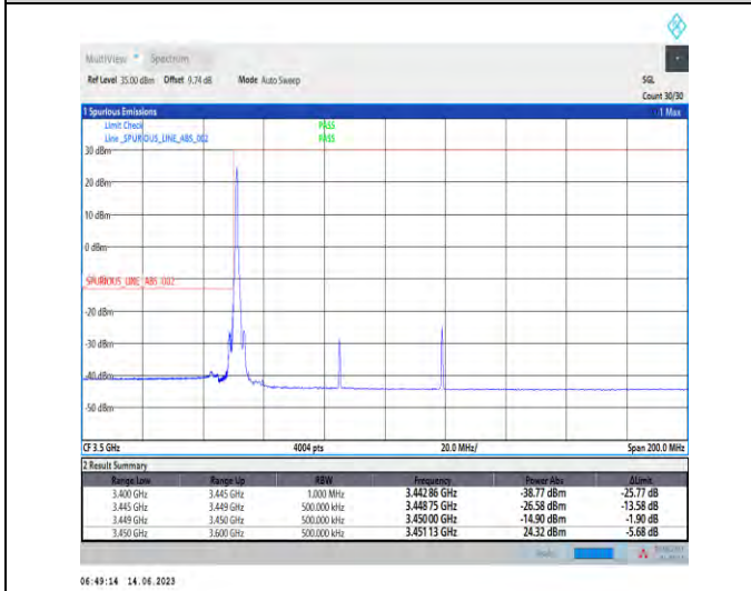
1-N78-3450-3550-PC1.5-30-70-L-4-CP-QPSK-Edge_1RB_Left-1@0-Ant1-1-PASS-see graph
