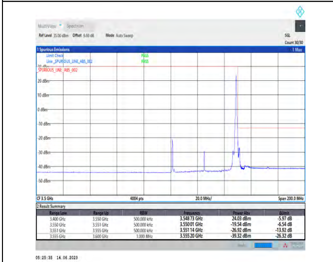
1-N78-3450-3550-PC1.5-30-50-H-5-CP-QPSK-Edge_1RB_Right-1@132-Ant1-1--PASS-see graph
