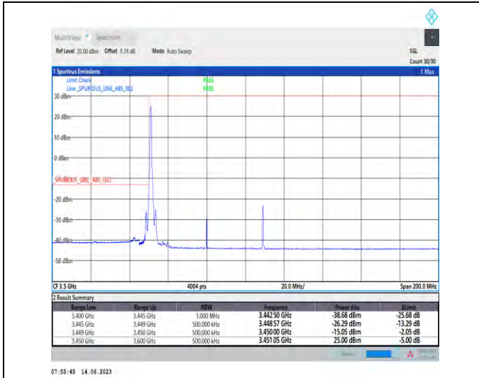
1-N78-3450-3550-PC1.5-30-60-L-1-DFT-PI2BPSK-Edge_1RB_Left-1@0-Ant1-1-PASS-see graph
