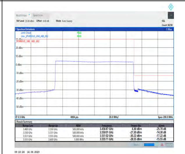
1-N78-3450-3550-PC1.5-30-100-H-6-CP-QPSK-O uter_Full-273@0-Ant1-1--PASS-see graph
