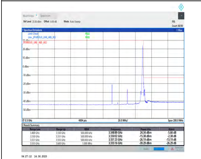
1-N78-3450-3550-PC1.5-30-40-H-5-CP-QPSK-Edge_1RB_Right-1@105-Ant1-1--PASS-see graph
