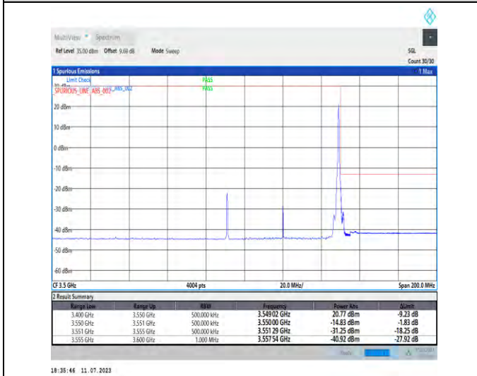
1-N78-3450-3550-PC1.5-30-60-H-5-CP-QPSK-Edge_1RB_Right-1@161-Ant1-1--PASS-see graph
