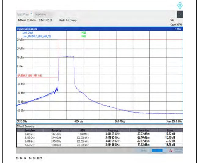
1-N78-3450-3550-PC1.5-30-20-L-6-CP-QPSK-Outer_Full-51@0-Ant1-1--PASS-see graph
