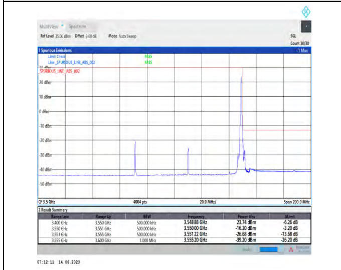
1-N78-3450-3550-PC1.5-30-80-H-5-CP-QPSK-Edge_1RB_Right-1@216-Ant1-1--PASS-see graph
