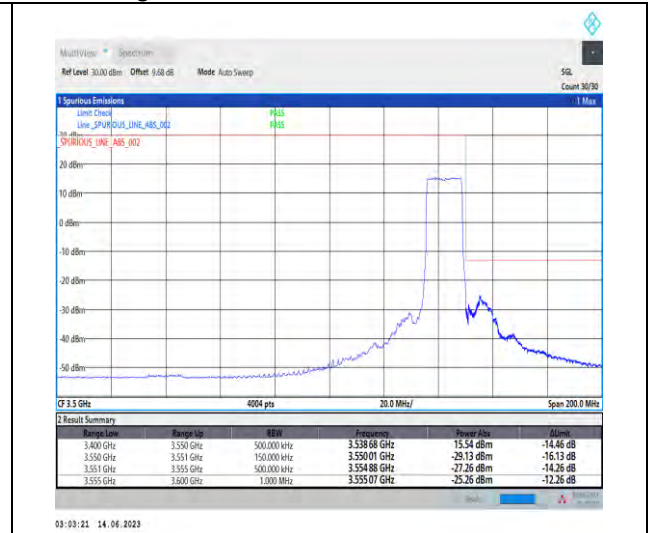
1-N78-3450-3550-PC1.5-30-15-H-3-DFT-PI2BPSK-Outer_Full-36@0-Ant1-1--PASS-see graph
