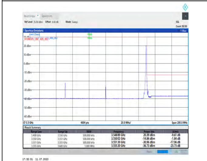
1-N78-3450-3550-PC1.5-30-100-H-5-CP-QPSK-Edge_1RB_Right-1@272-Ant1-1--PASS-see graph
