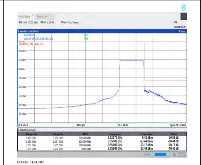
1-N78-3450-3550-PC1.5-30-30-H-6-CP-QPSK-Outer_Full-78@0-Ant1-1--PASS-see graph
