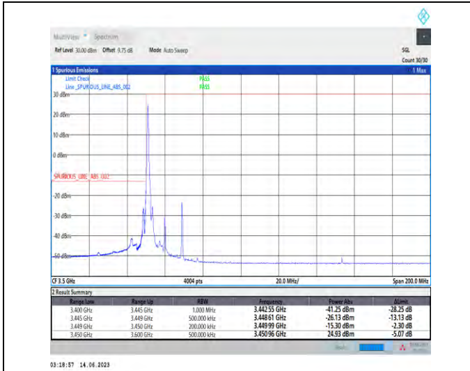
1-N78-3450-3550-PC1.5-30-20-L-1-DFT-PI2BPSK-Edge_1RB_Left-1@0-Ant1-1--PASS-see graph
