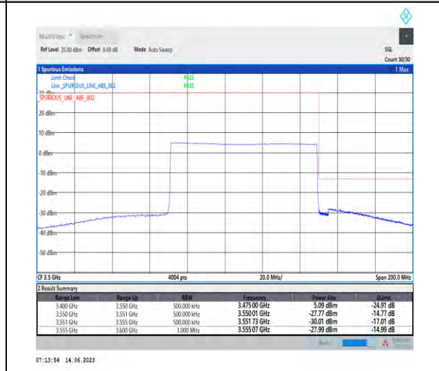
1-N78-3450-3550-PC1.5-30-80-H-6-CP-QPSK-Outer_Full-217@0-Ant1-1--PASS-see graph
