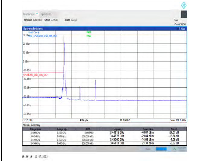
1-N78-3450-3550-PC1.5-30-40-L-4-CP-QPSK-Edge_1RB_Left-1@0-Ant1-1--PASS-see graph
