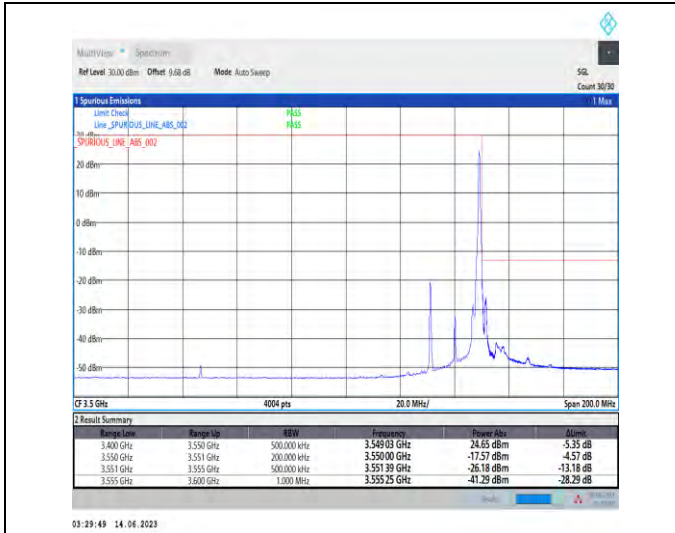
1-N78-3450-3550-PC1.5-30-20-H-2-DFT-PI2BPSK-Edge_1RB_Right-1@50-Ant1-1--PASS-see graph
