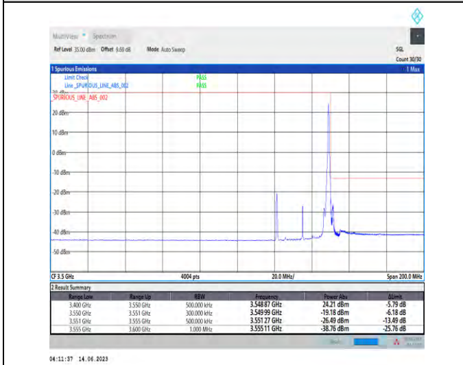
1-N78-3450-3550-PC1.5-30-30-H-5-CP-QPSK-Edge_1RB_Right-1@77-Ant1-1--PASS-see graph
