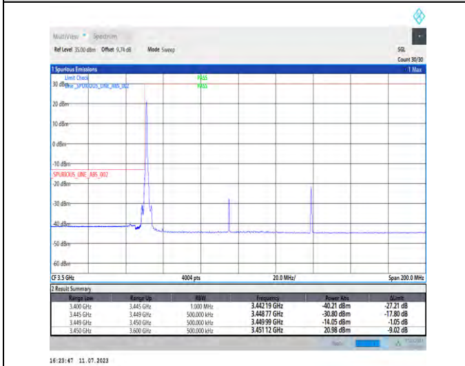
1-N78-3450-3550-PC1.5-30-90-L-4-CP-QPSK-Edge_1RB_Left-1@0-Ant1-1-PASS-see graph
