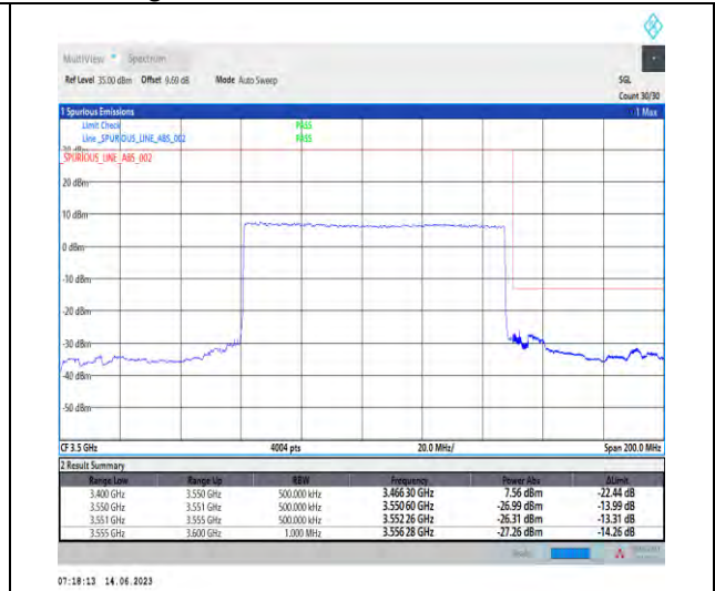
1-N78-3450-3550-PC1.5-30-90-H-3-DFT-PI2BPSK-Outer_Full-240@0-Ant1-1--PASS-see graph
