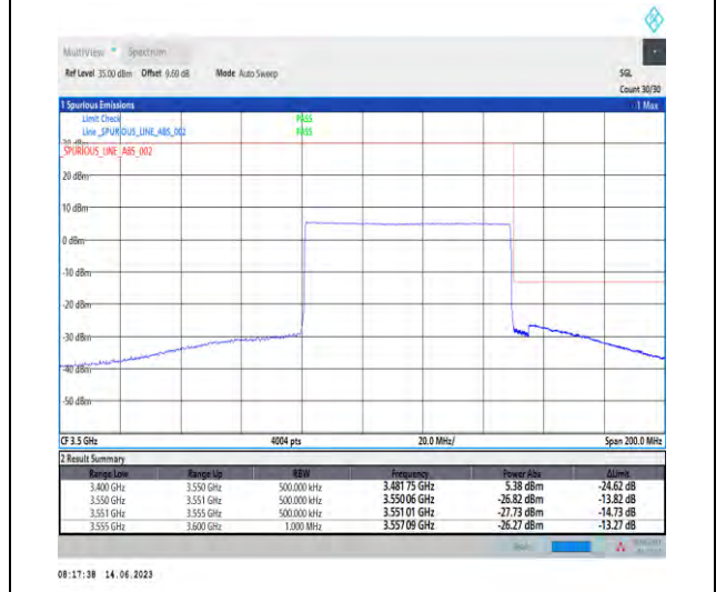
1-N78-3450-3550-PC1.5-30-70-H-6-CP-QPSK-Outer_Full-189@0-Ant1-1--PASS-see graph
