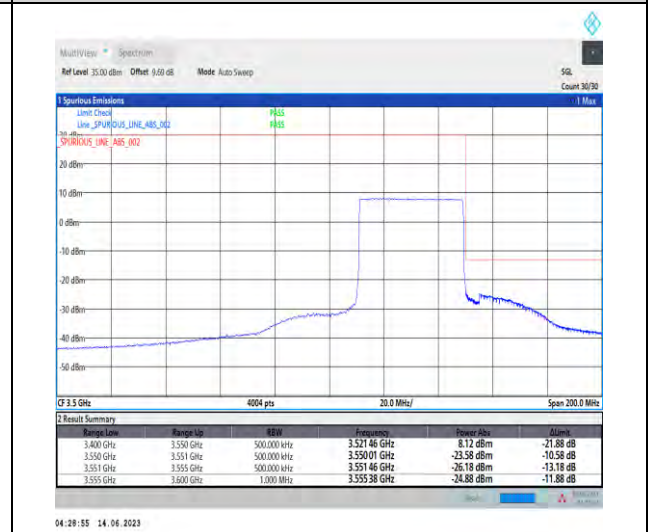
1-N78-3450-3550-PC1.5-30-40-H-6-CP-QPSK-Outer_Full-106@0-Ant1-1--PASS-see graph
