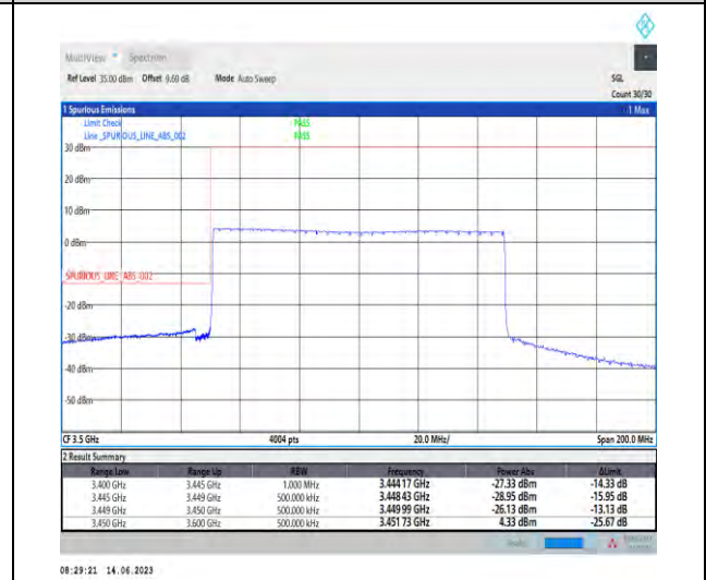
1-N78-3450-3550-PC1.5-30-100-L-6-CP-QPSK-Outer_Full-273@0-Ant1-1--PASS-see graph
